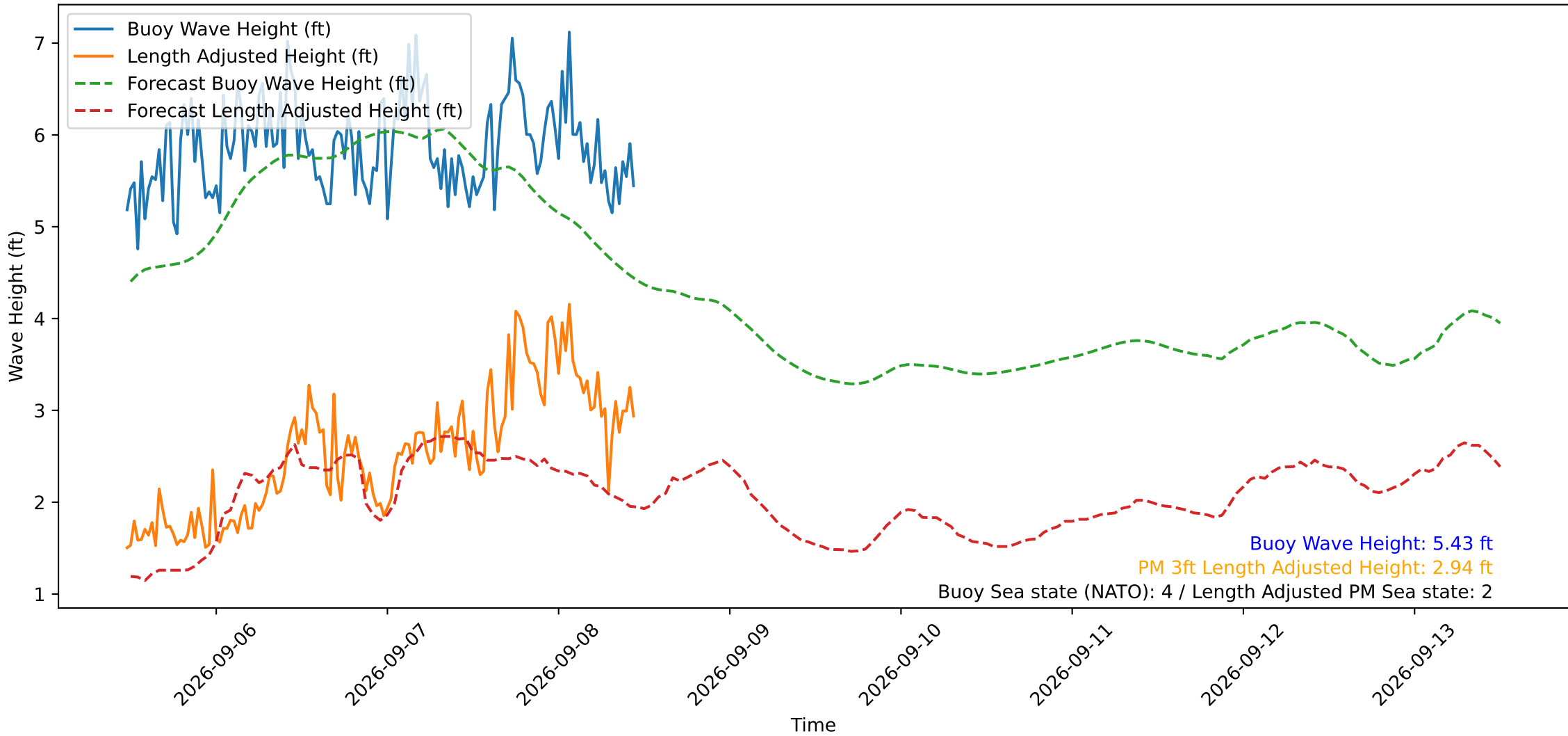
Wave Heights over Time for Oceanside Harbor at 2026-09-08 11:30:29
