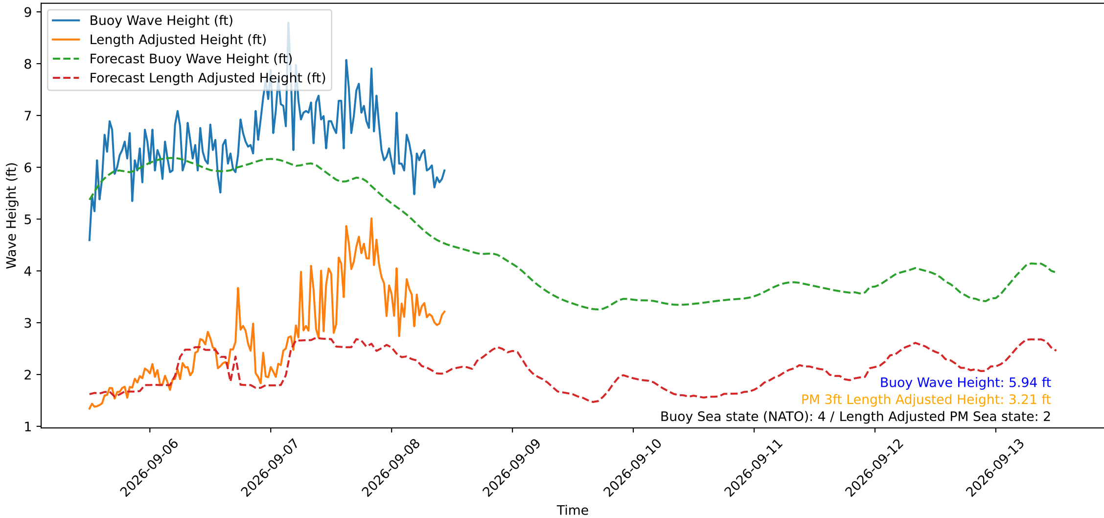
Wave Heights over Time for Green Beach at 2026-09-08 11:31:12
