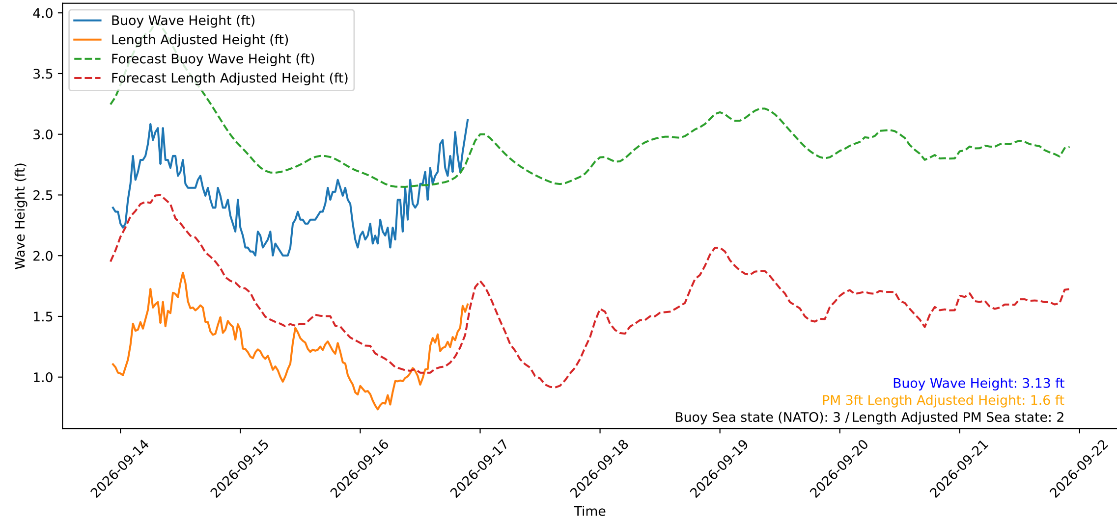
Wave Heights over Time for Red Beach at 2026-09-16 22:20:49
