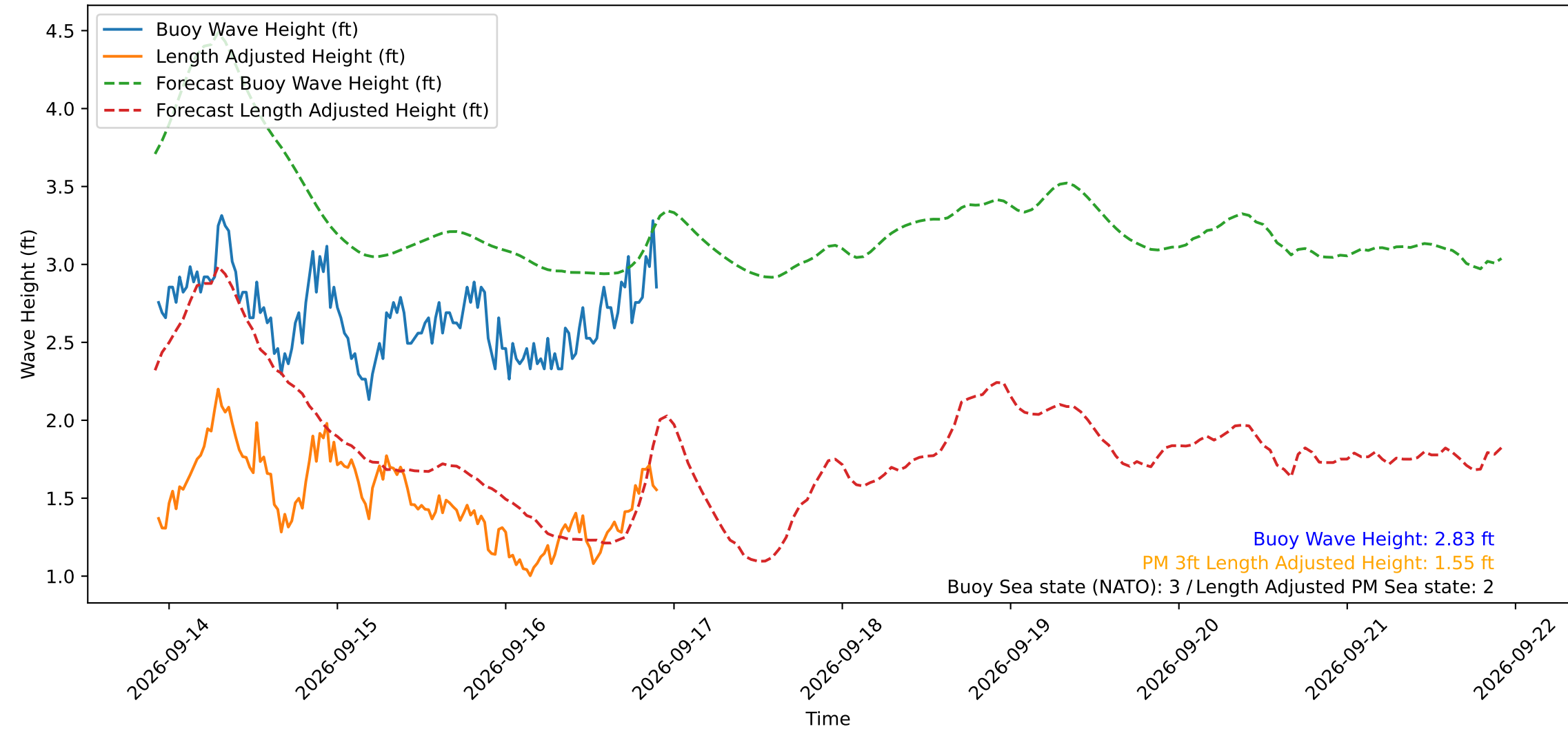
Wave Heights over Time for Green Beach at 2026-09-16 22:21:13
