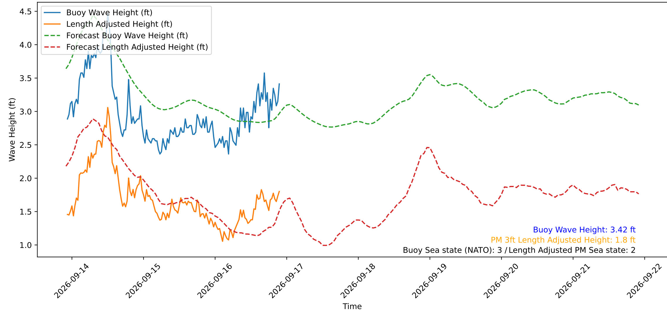
Wave Heights over Time for Oceanside Harbor at 2026-09-16 22:20:29
