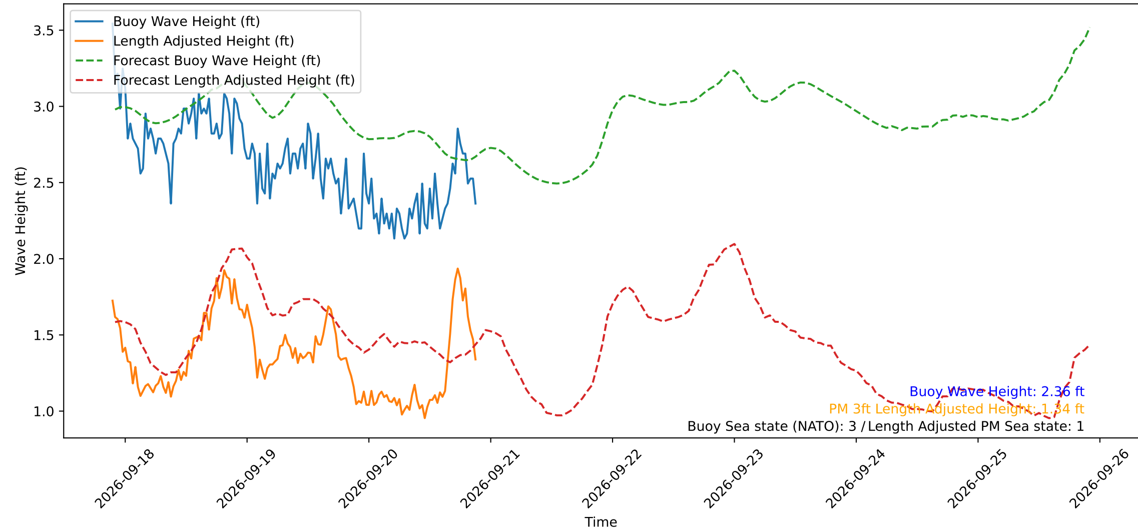
Wave Heights over Time for Oceanside Harbor at 2026-09-20 21:30:29
