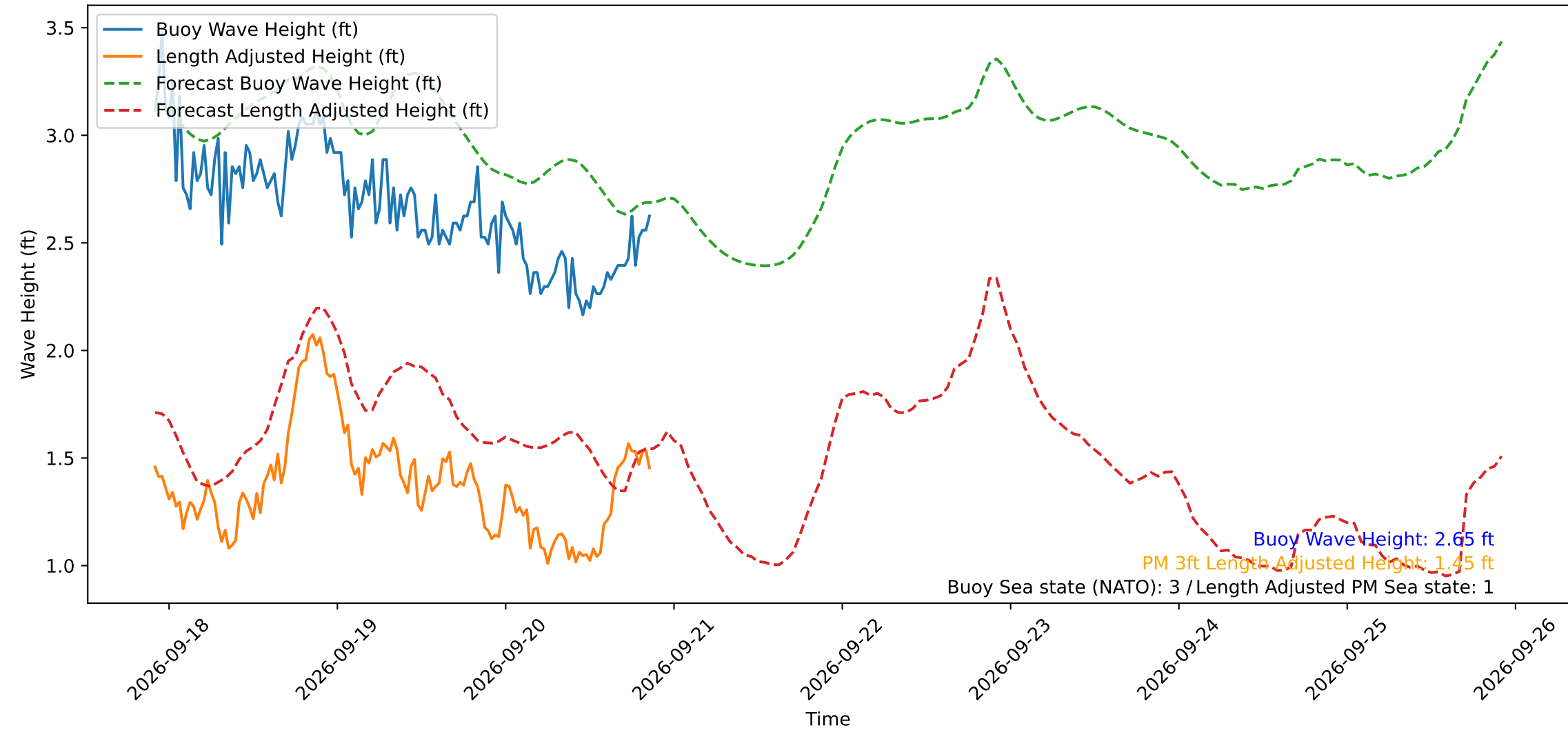
Wave Heights over Time for Green Beach at 2026-09-20 21:31:11
