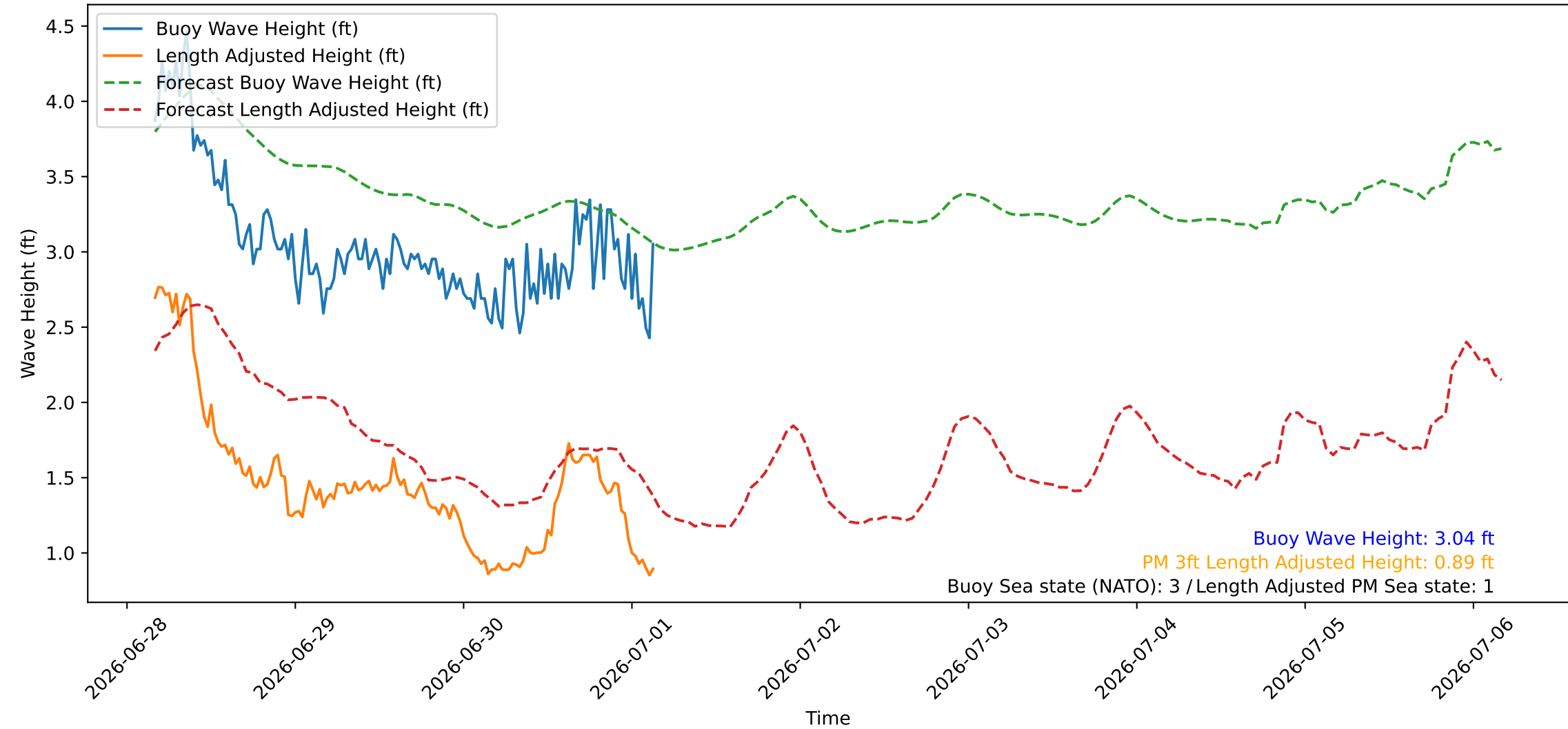
Wave Heights over Time for Red Beach at 2026-07-01 03:40:45
