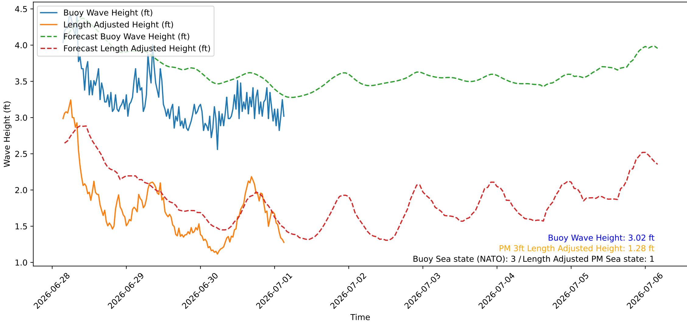
Wave Heights over Time for Oceanside Harbor at 2026-07-01 03:40:26
