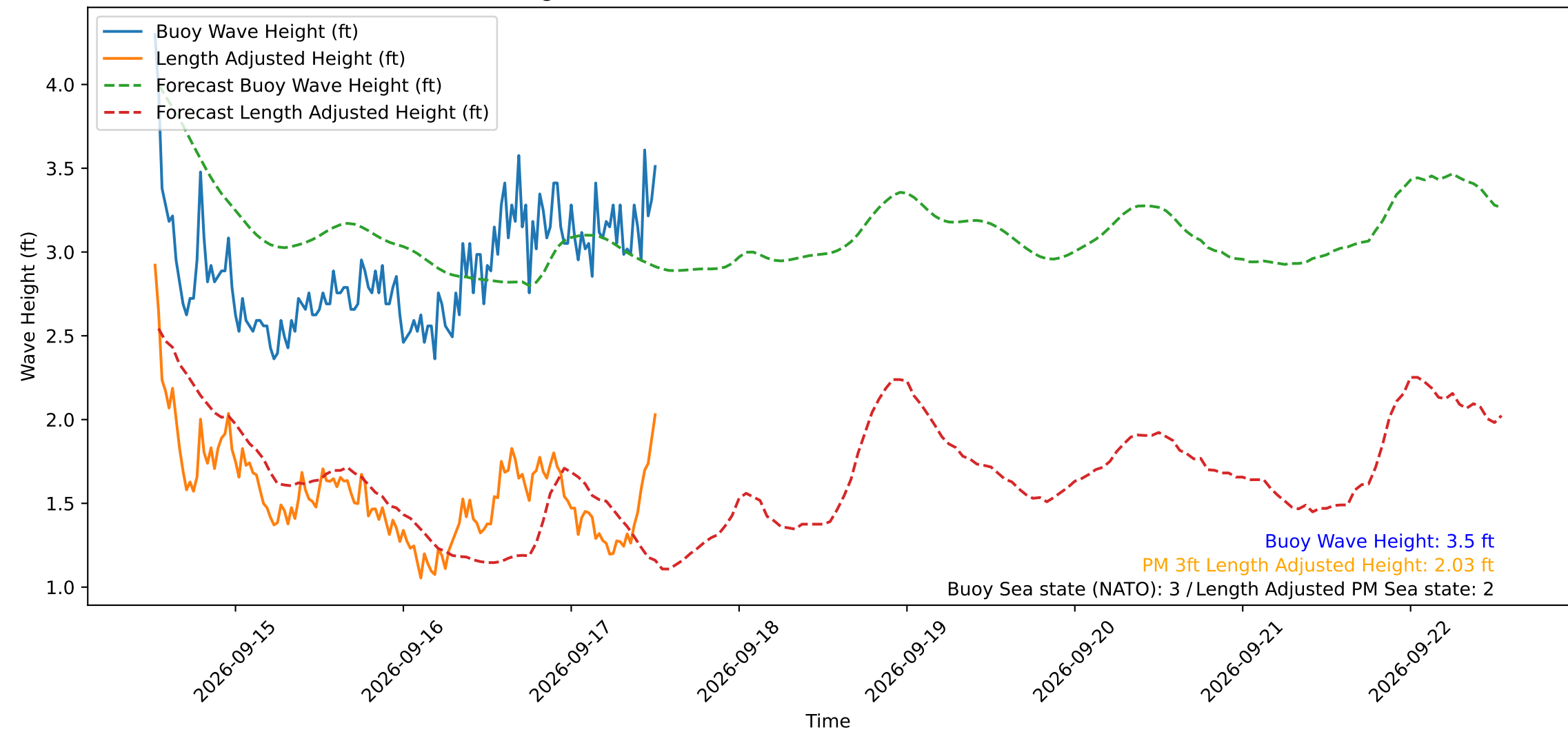
Wave Heights over Time for Oceanside Harbor at 2026-09-17 12:30:30
