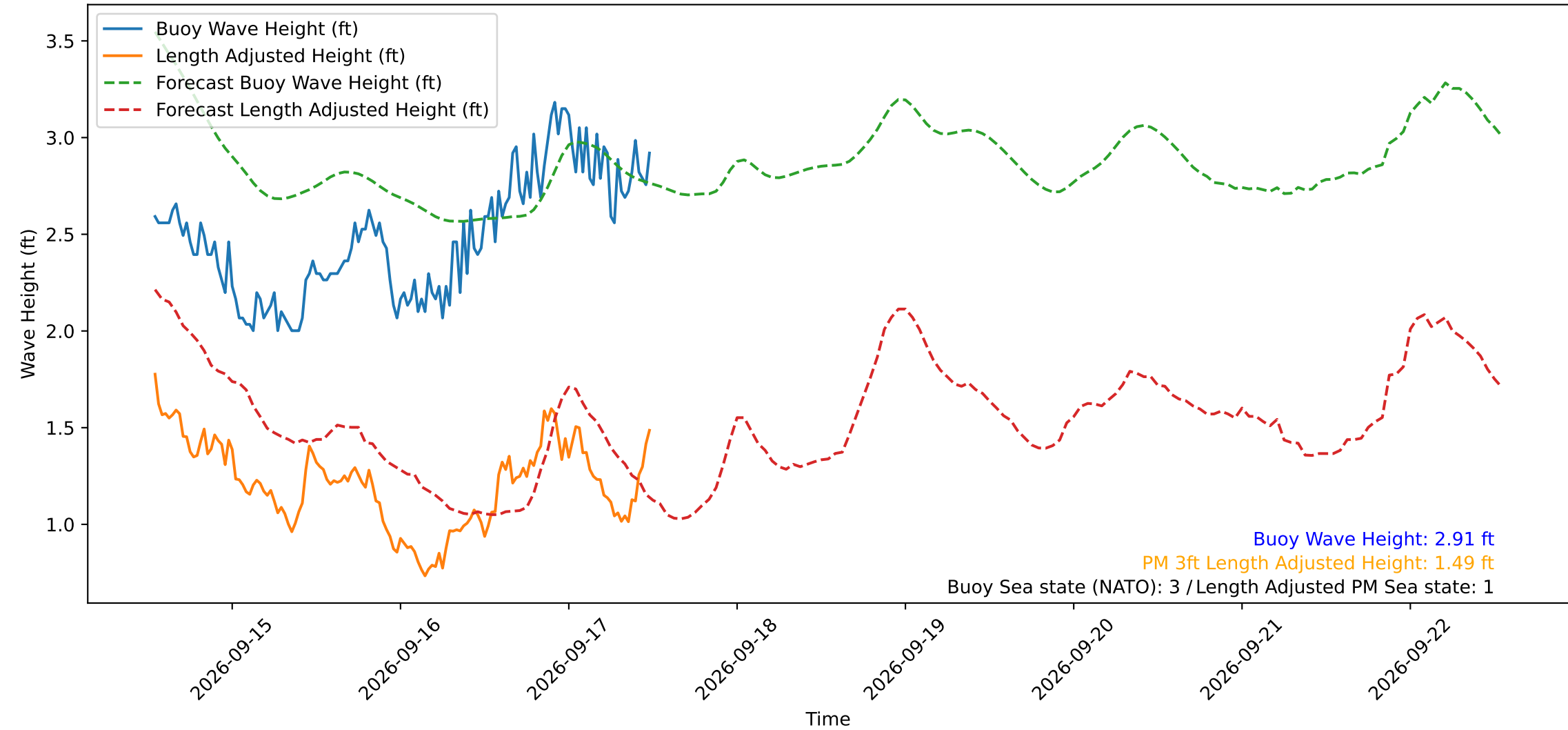
Wave Heights over Time for Red Beach at 2026-09-17 12:30:50
