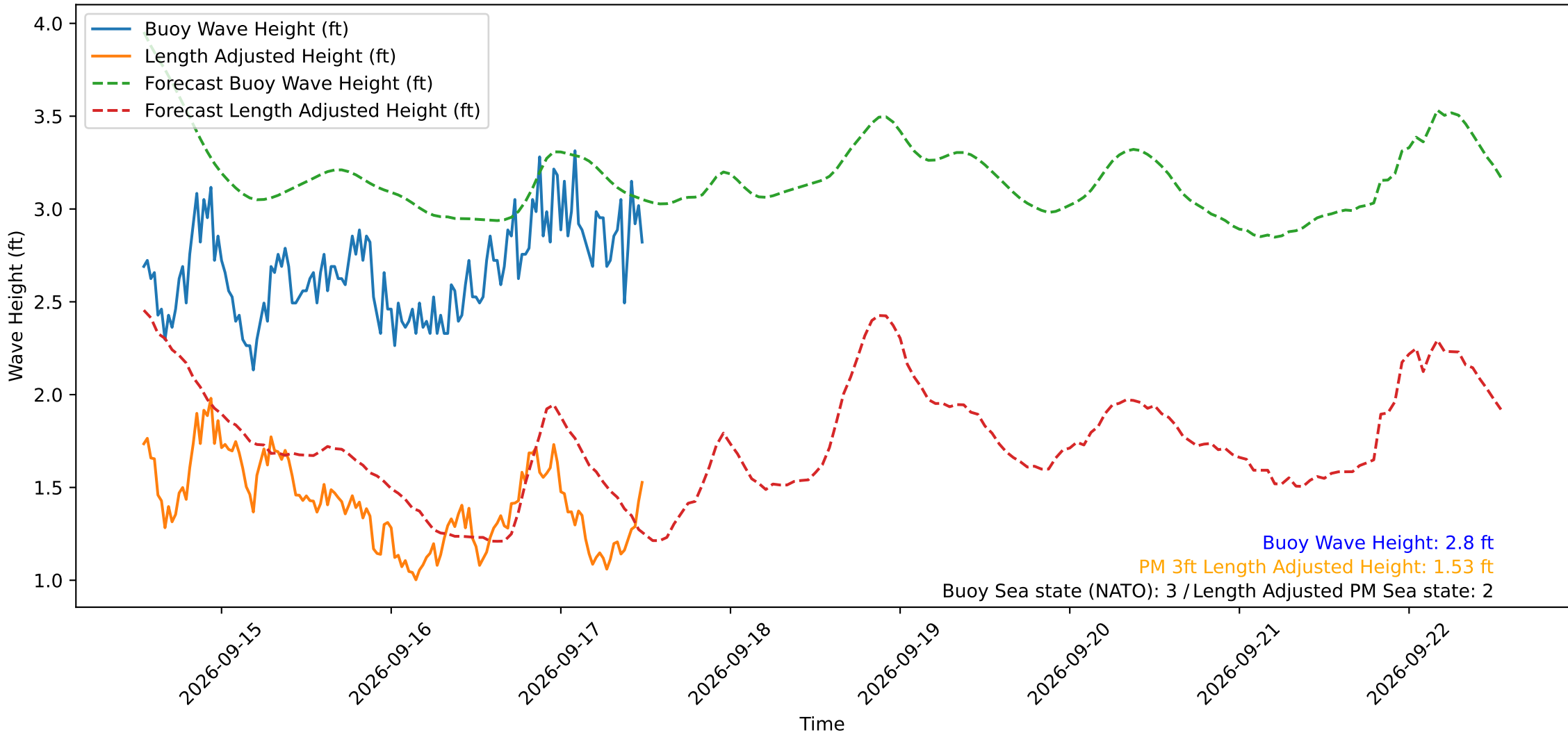
Wave Heights over Time for Green Beach at 2026-09-17 12:31:12
