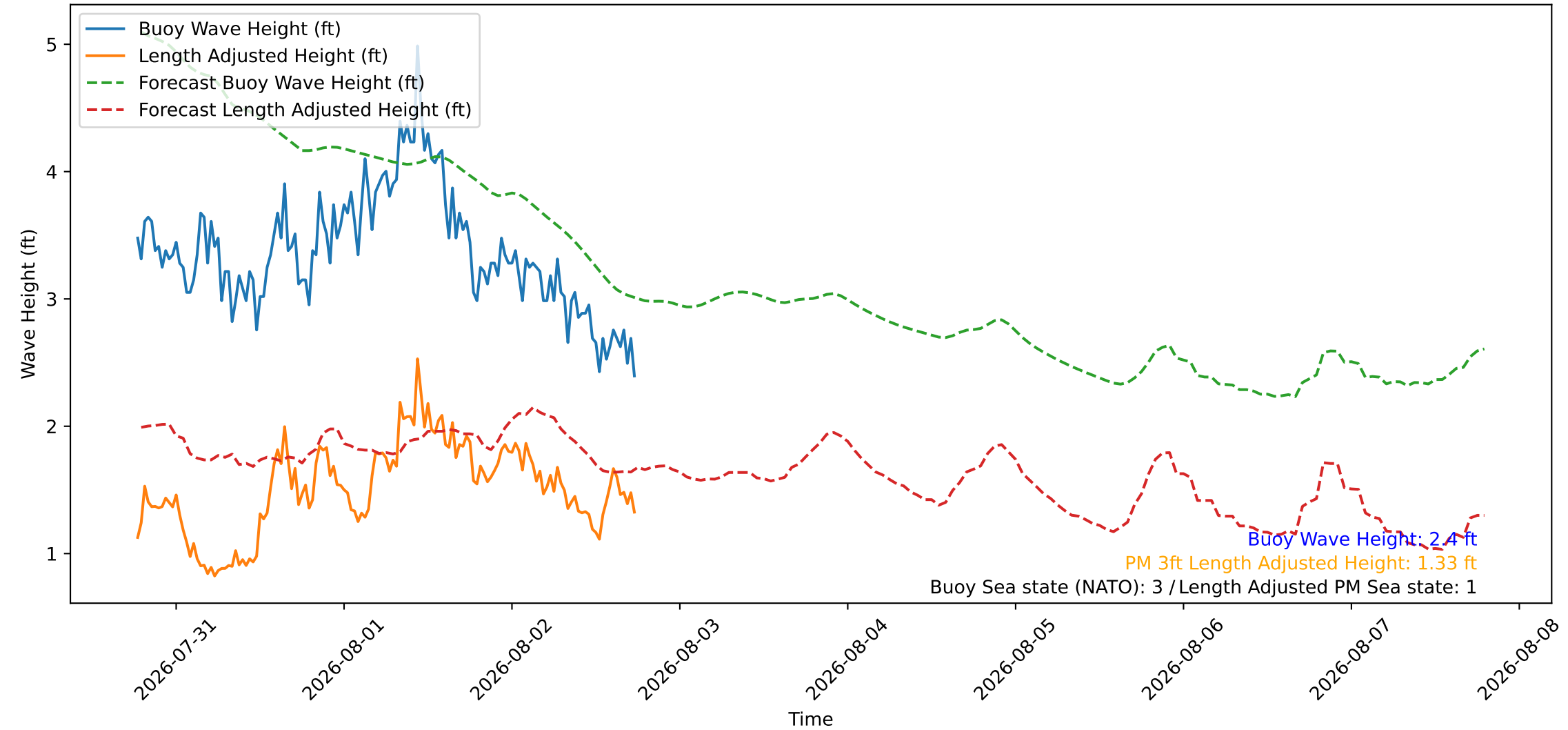
Wave Heights over Time for Green Beach at 2026-08-02 18:31:08
