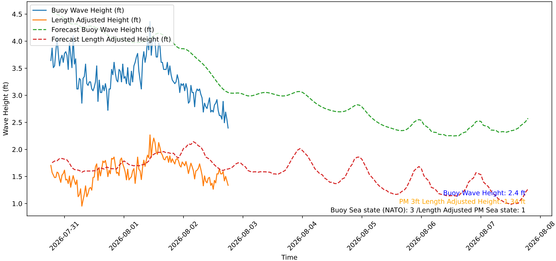
Wave Heights over Time for Oceanside Harbor at 2026-08-02 18:30:26
