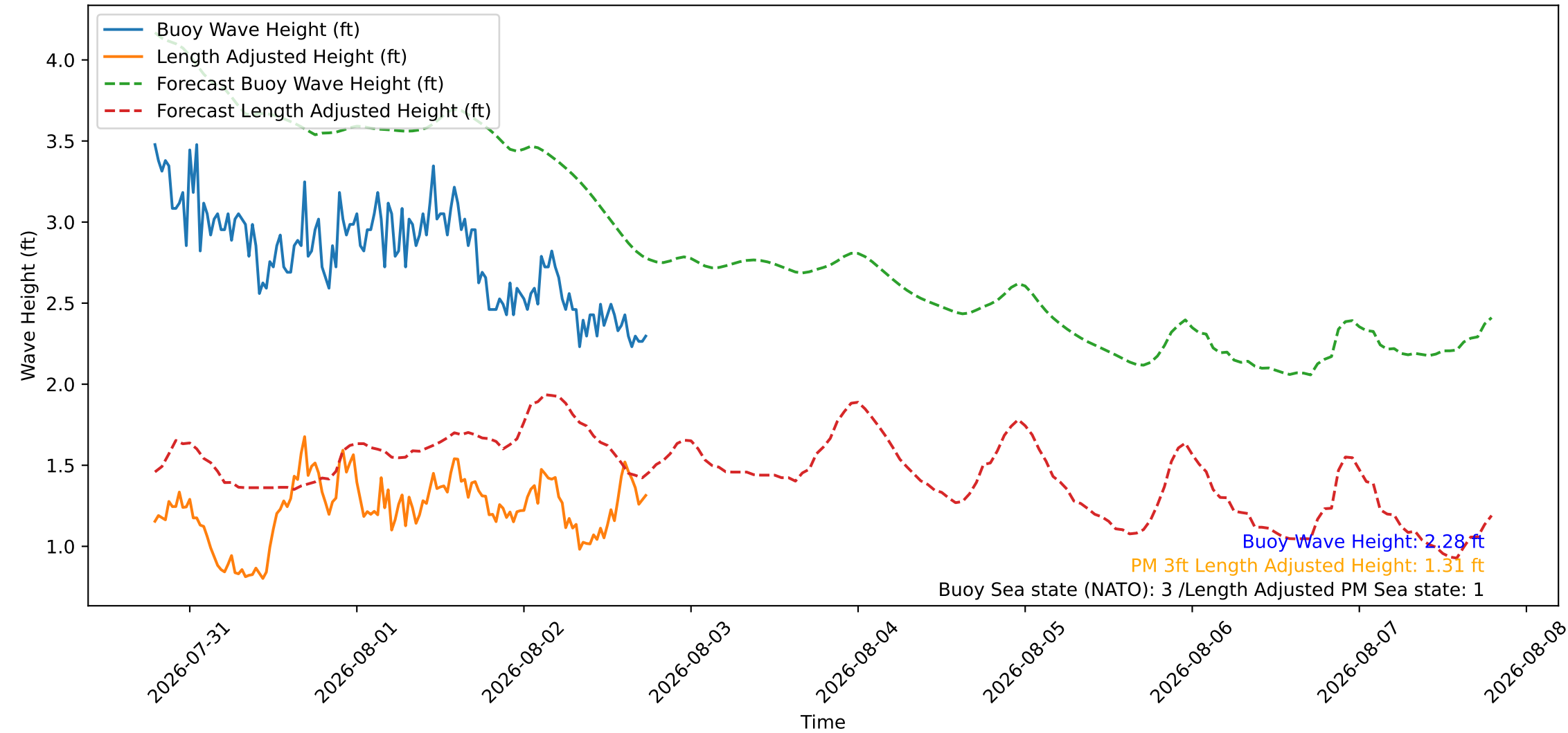
Wave Heights over Time for Red Beach at 2026-08-02 18:30:46
