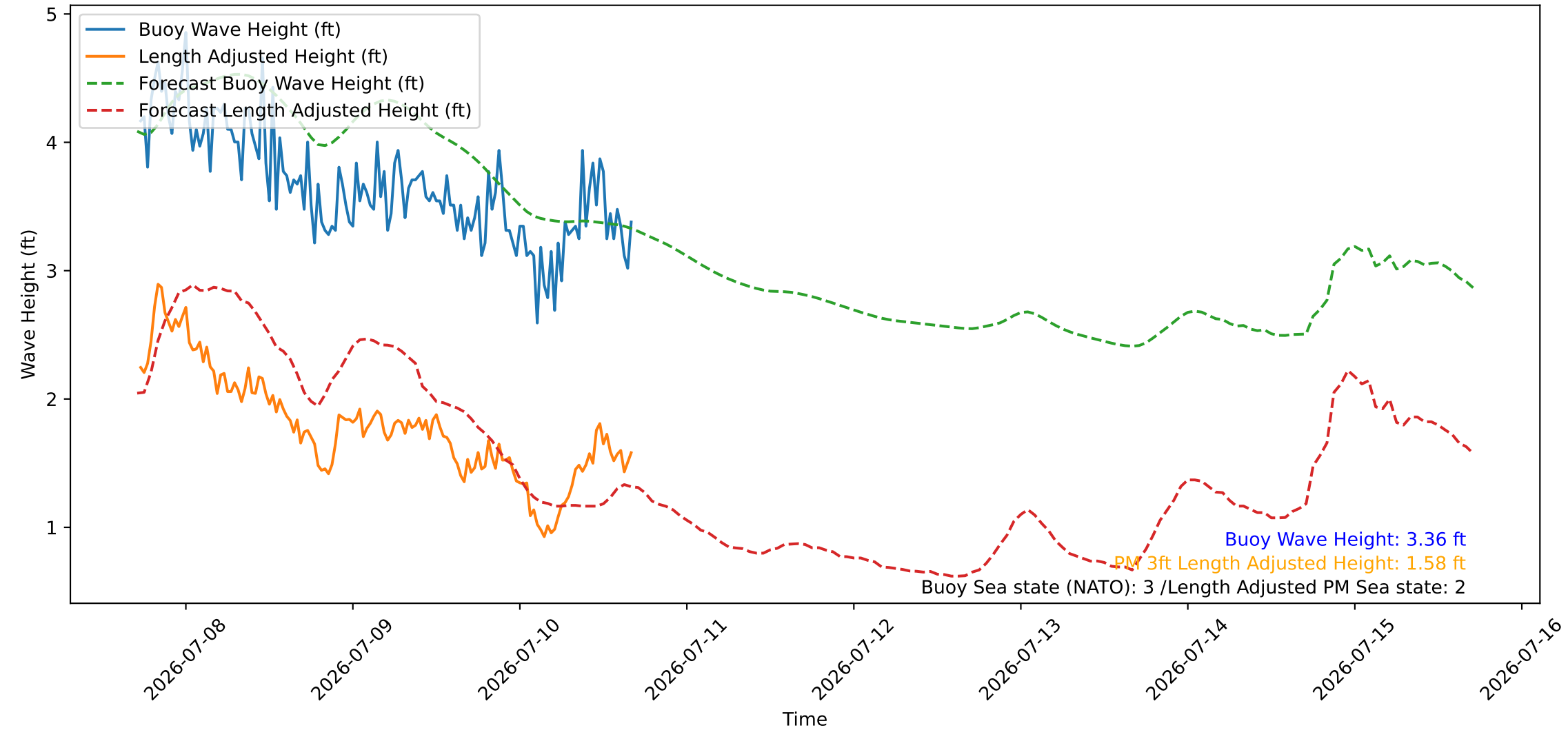
Wave Heights over Time for Red Beach at 2026-07-10 17:10:46
