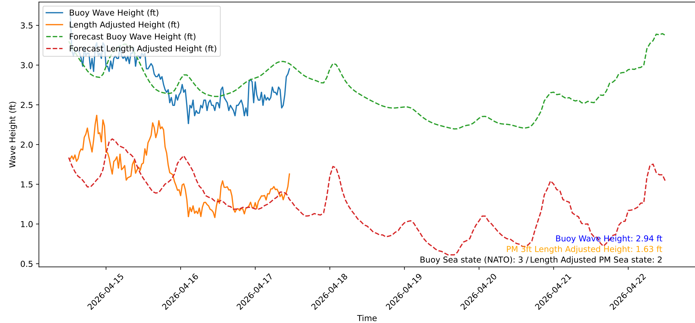
Wave Heights over Time for Red Beach at 2026-04-17 12:00:50
