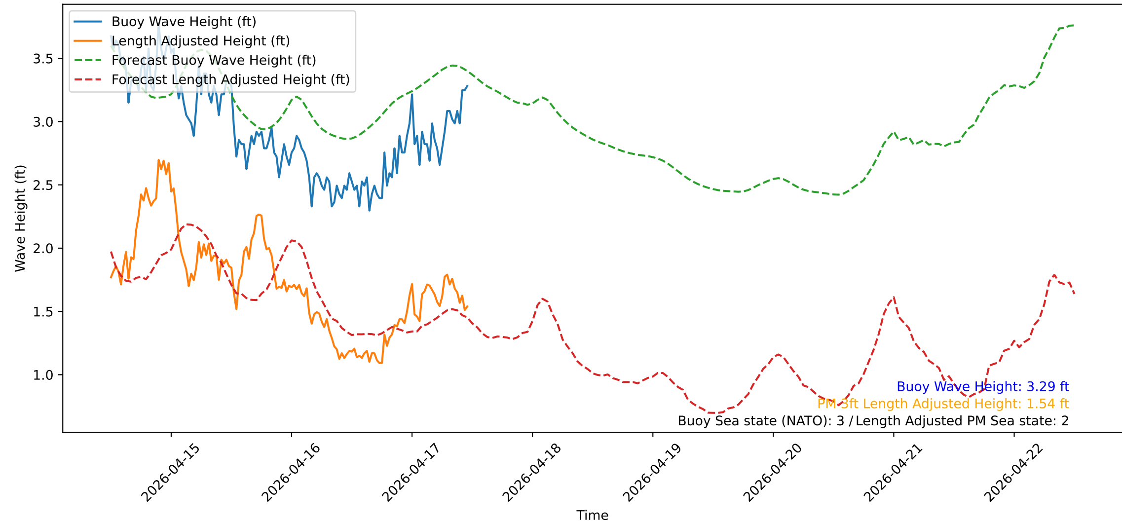
Wave Heights over Time for Oceanside Harbor at 2026-04-17 12:00:31
