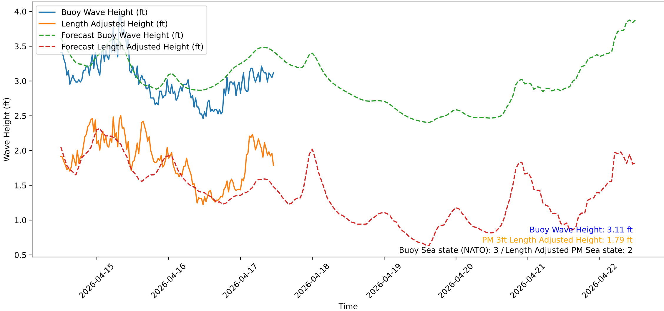
Wave Heights over Time for Green Beach at 2026-04-17 12:01:13
