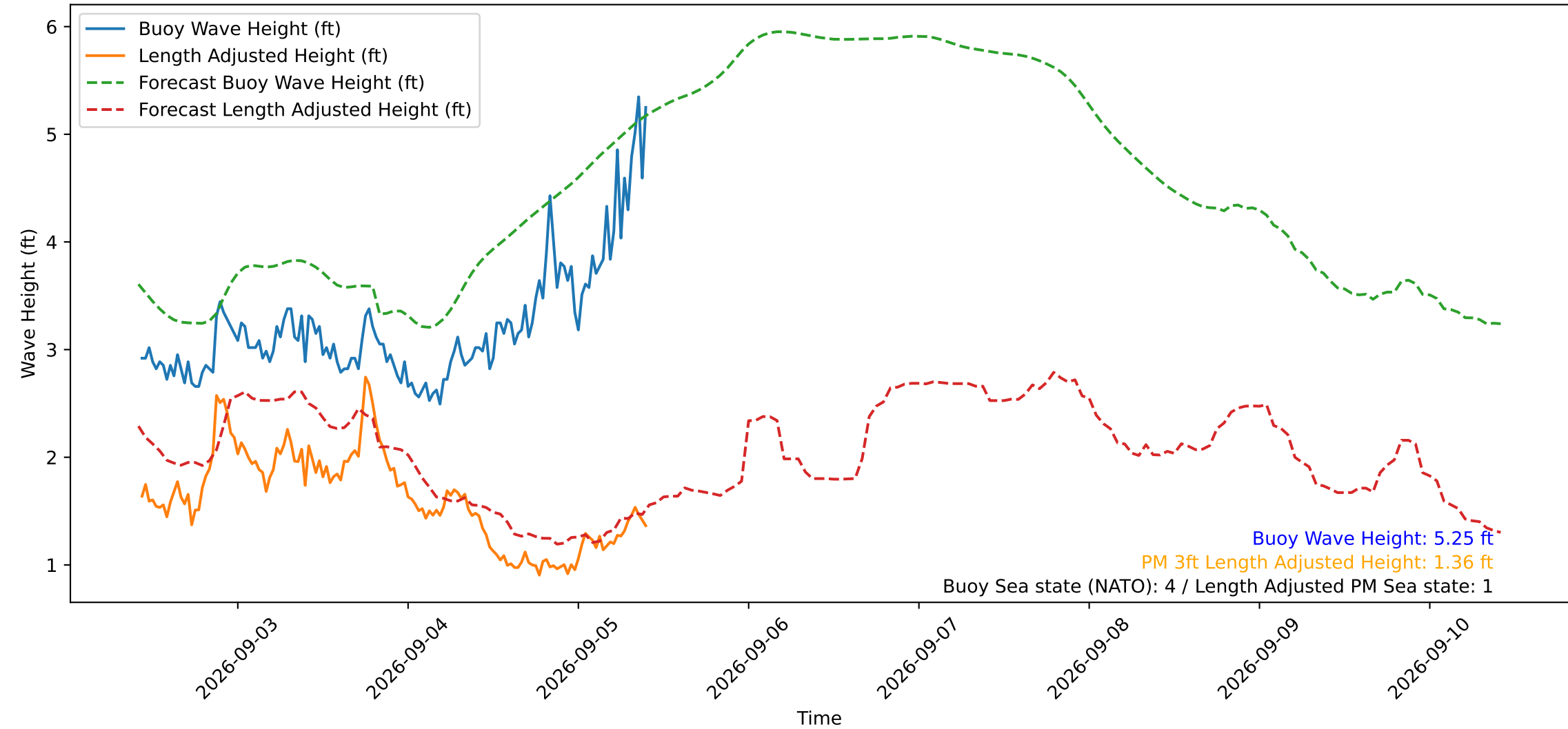
Wave Heights over Time for Green Beach at 2026-09-05 10:21:14
