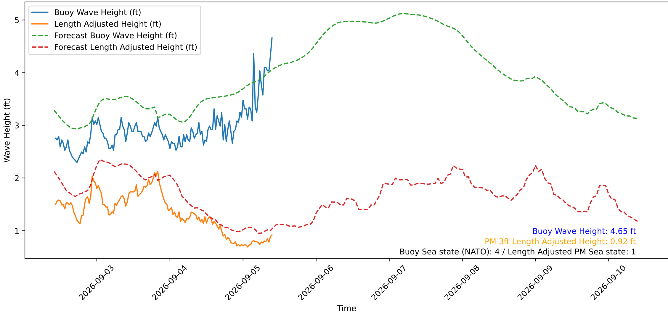
Wave Heights over Time for Red Beach at 2026-09-05 10:20:50
