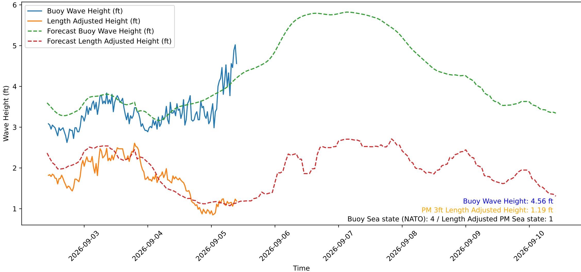
Wave Heights over Time for Oceanside Harbor at 2026-09-05 10:20:29
