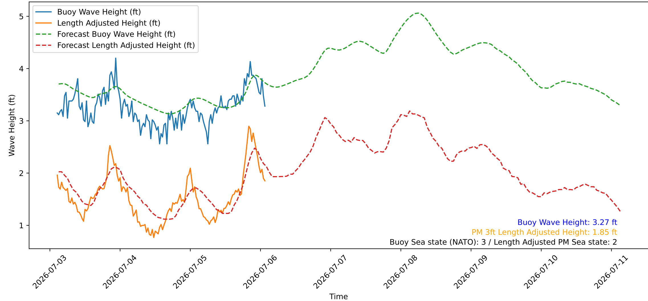
Wave Heights over Time for Green Beach at 2026-07-06 02:31:07
