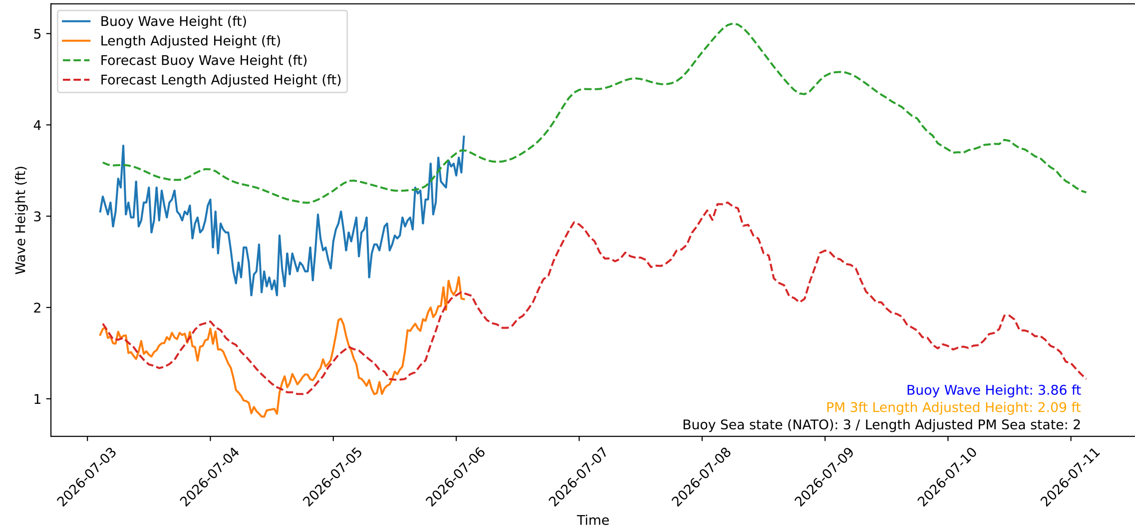
Wave Heights over Time for Oceanside Harbor at 2026-07-06 02:30:26
