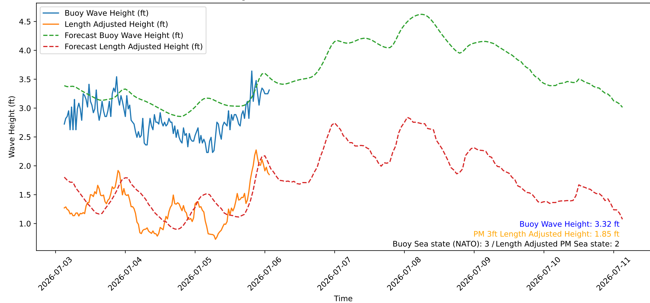
Wave Heights over Time for Red Beach at 2026-07-06 02:30:45
