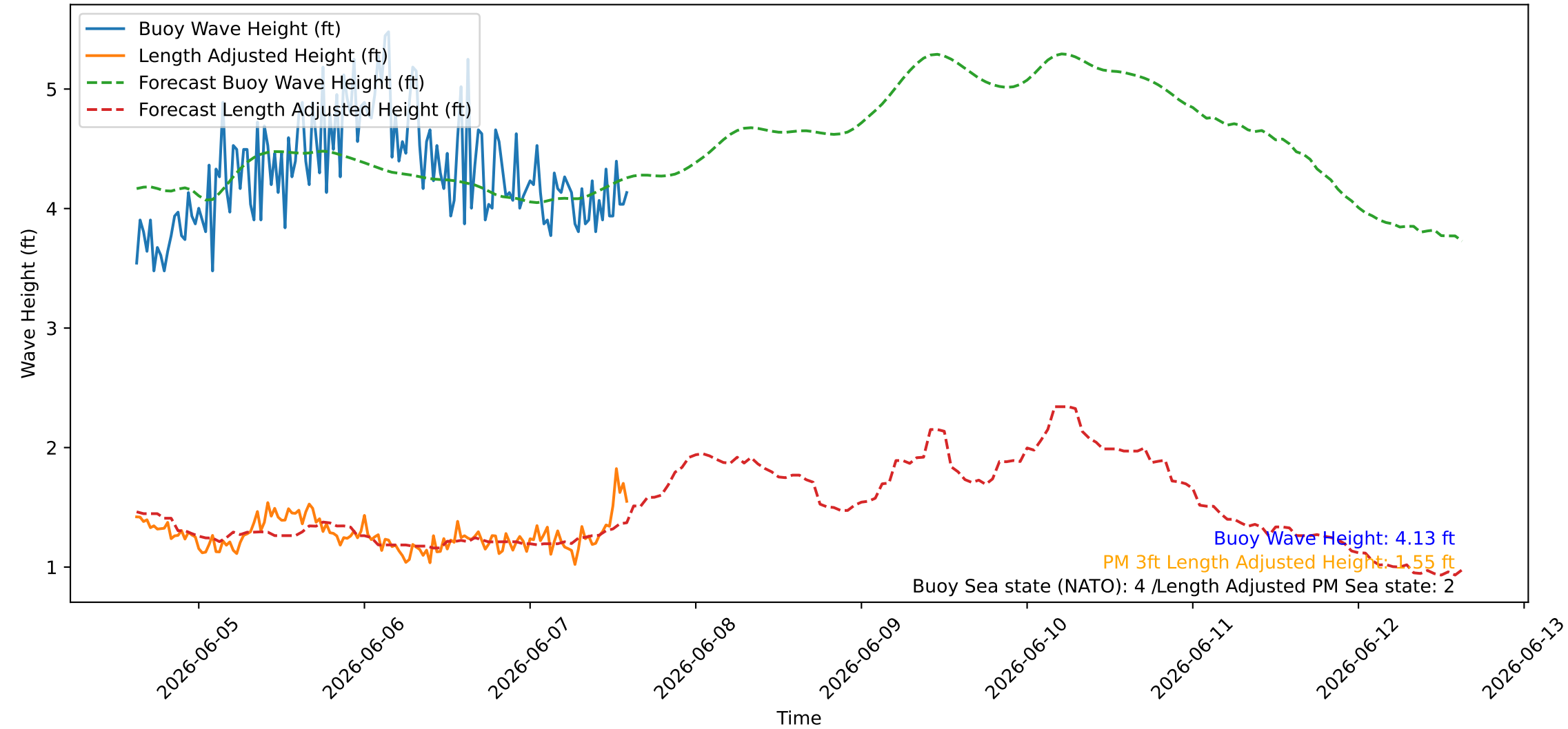
Wave Heights over Time for Oceanside Harbor at 2026-06-07 14:50:26
