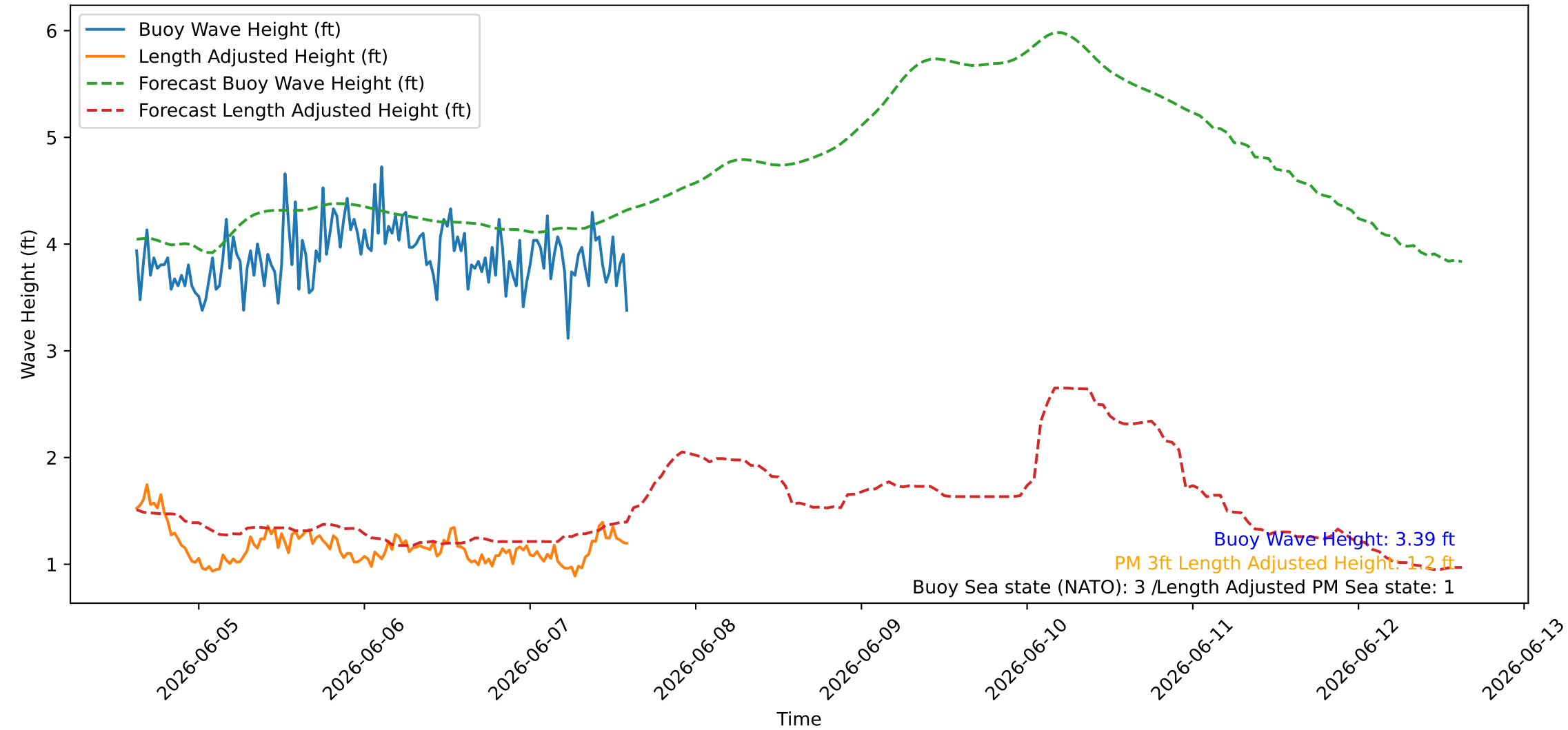
Wave Heights over Time for Green Beach at 2026-06-07 14:51:10
