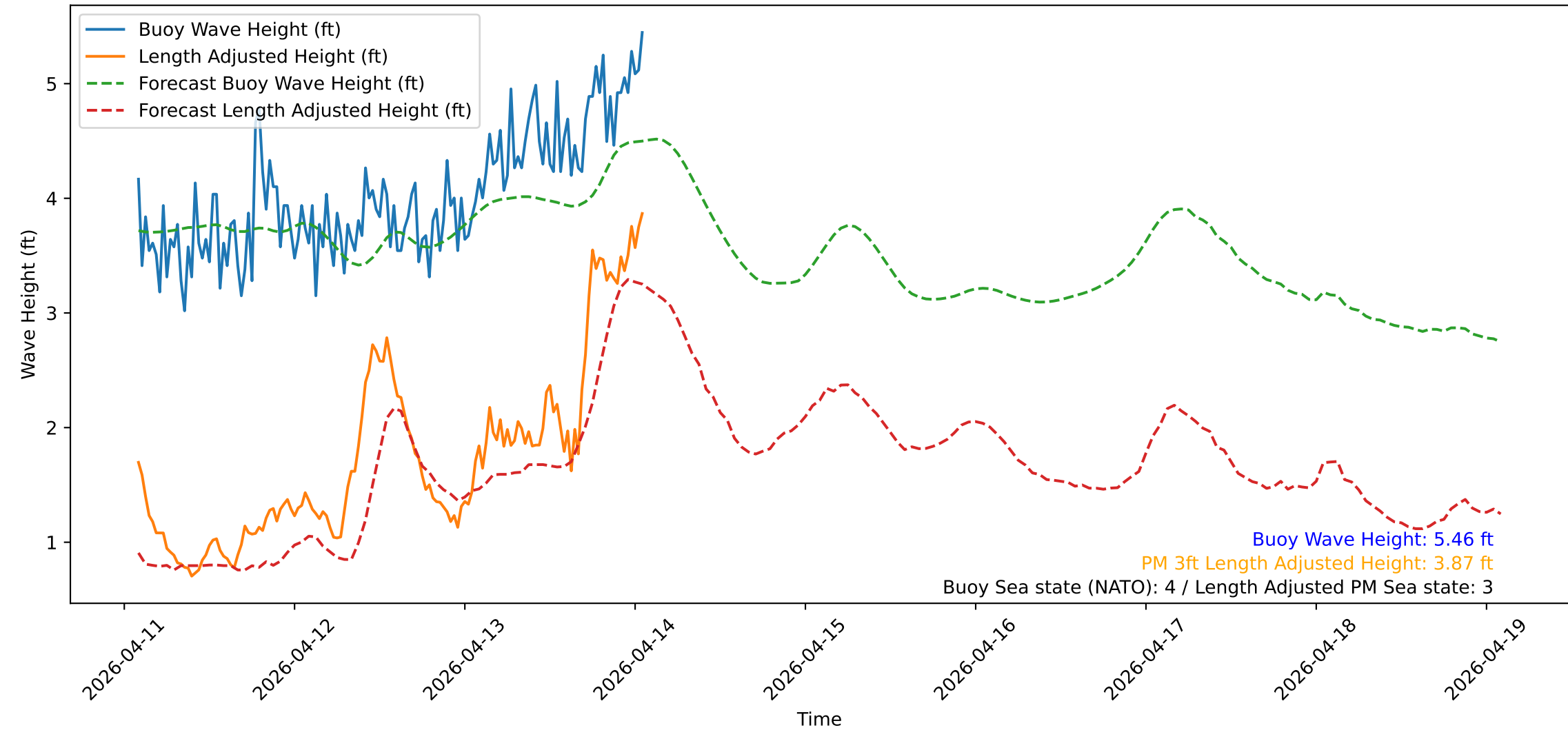
Wave Heights over Time for Oceanside Harbor at 2026-04-14 01:50:31
