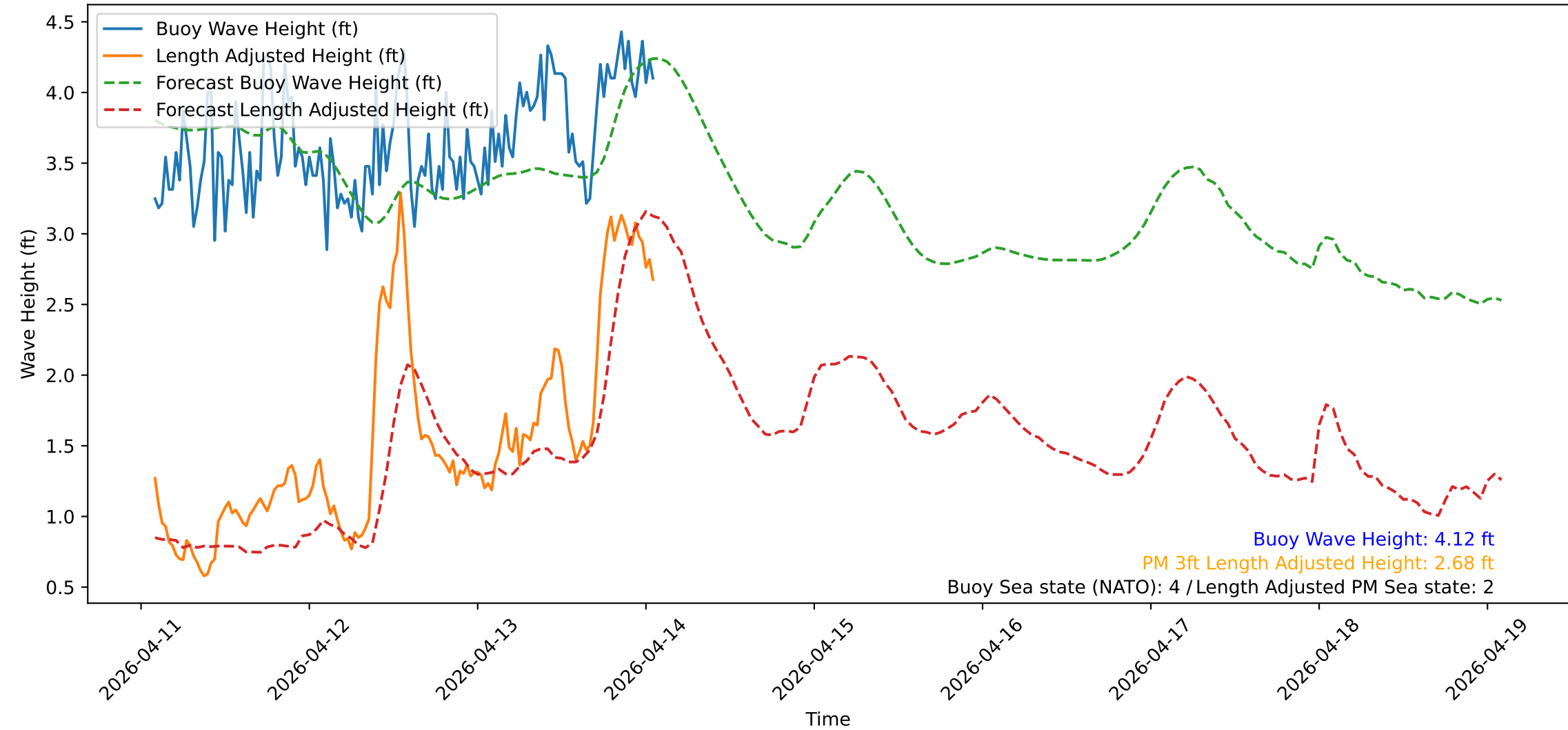
Wave Heights over Time for Red Beach at 2026-04-14 01:50:51
