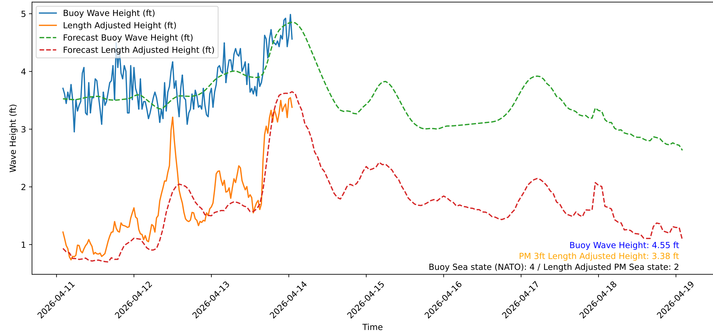
Wave Heights over Time for Green Beach at 2026-04-14 01:51:14
