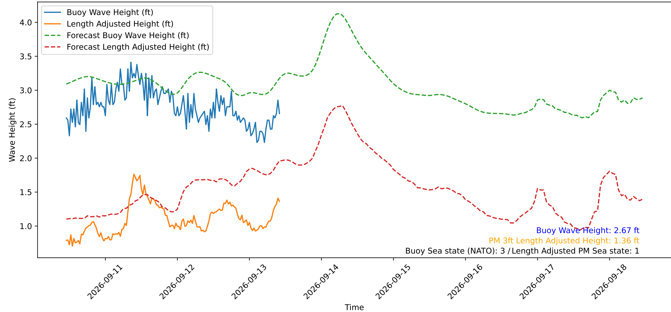
Wave Heights over Time for Red Beach at 2026-09-13 10:50:50
