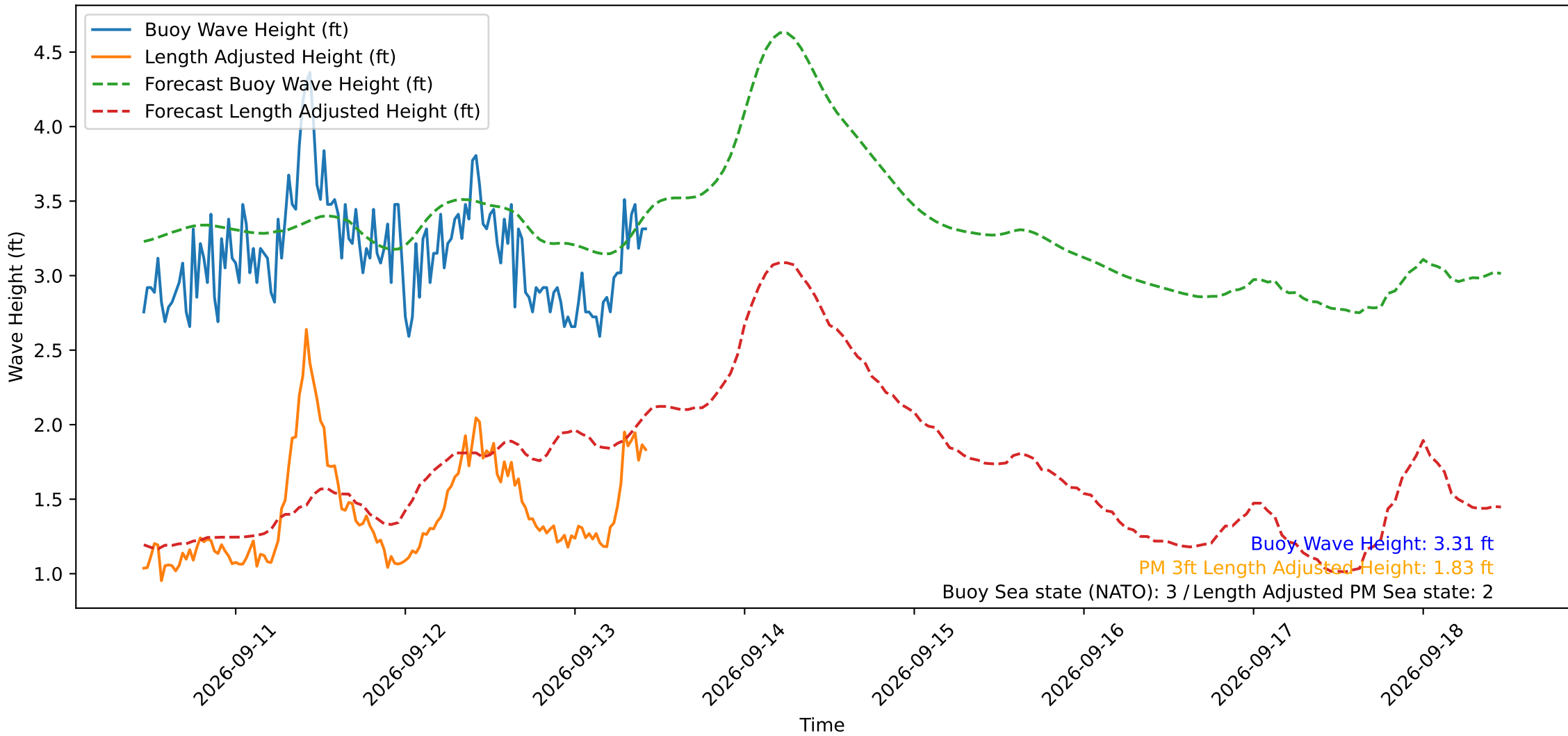
Wave Heights over Time for Oceanside Harbor at 2026-09-13 10:50:29
