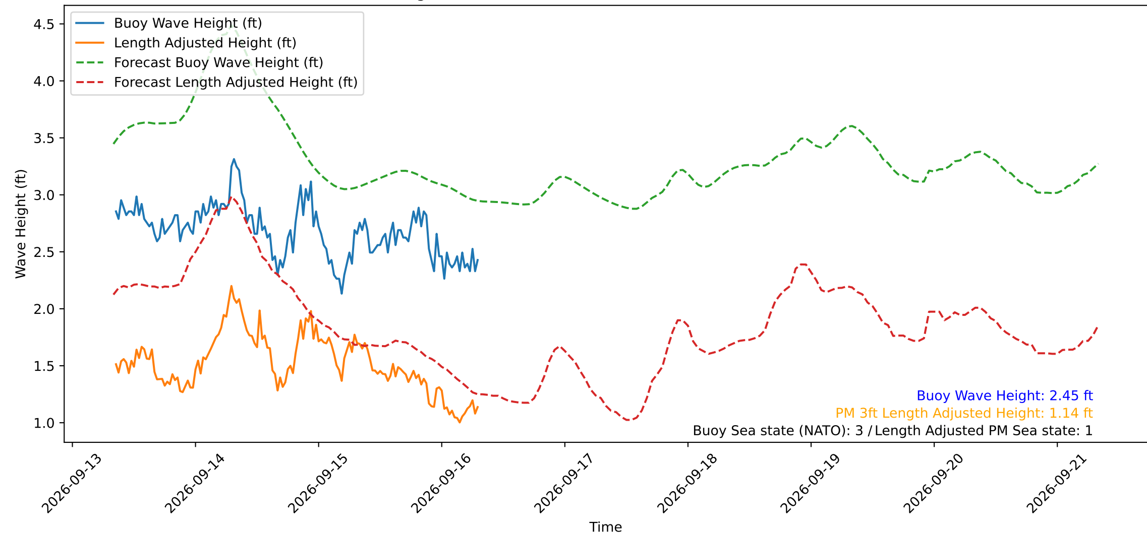
Wave Heights over Time for Green Beach at 2026-09-16 08:01:12
