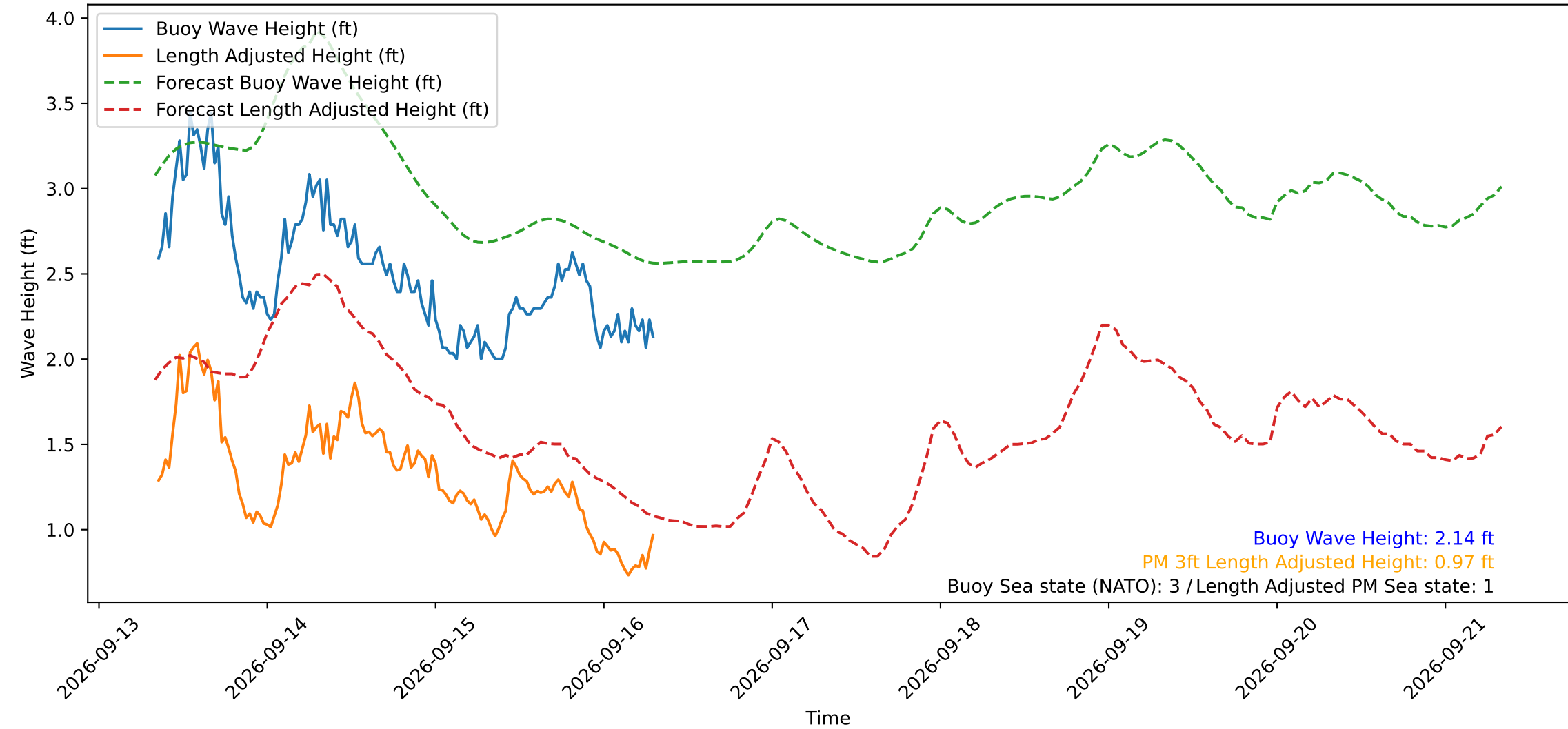
Wave Heights over Time for Red Beach at 2026-09-16 08:00:49
