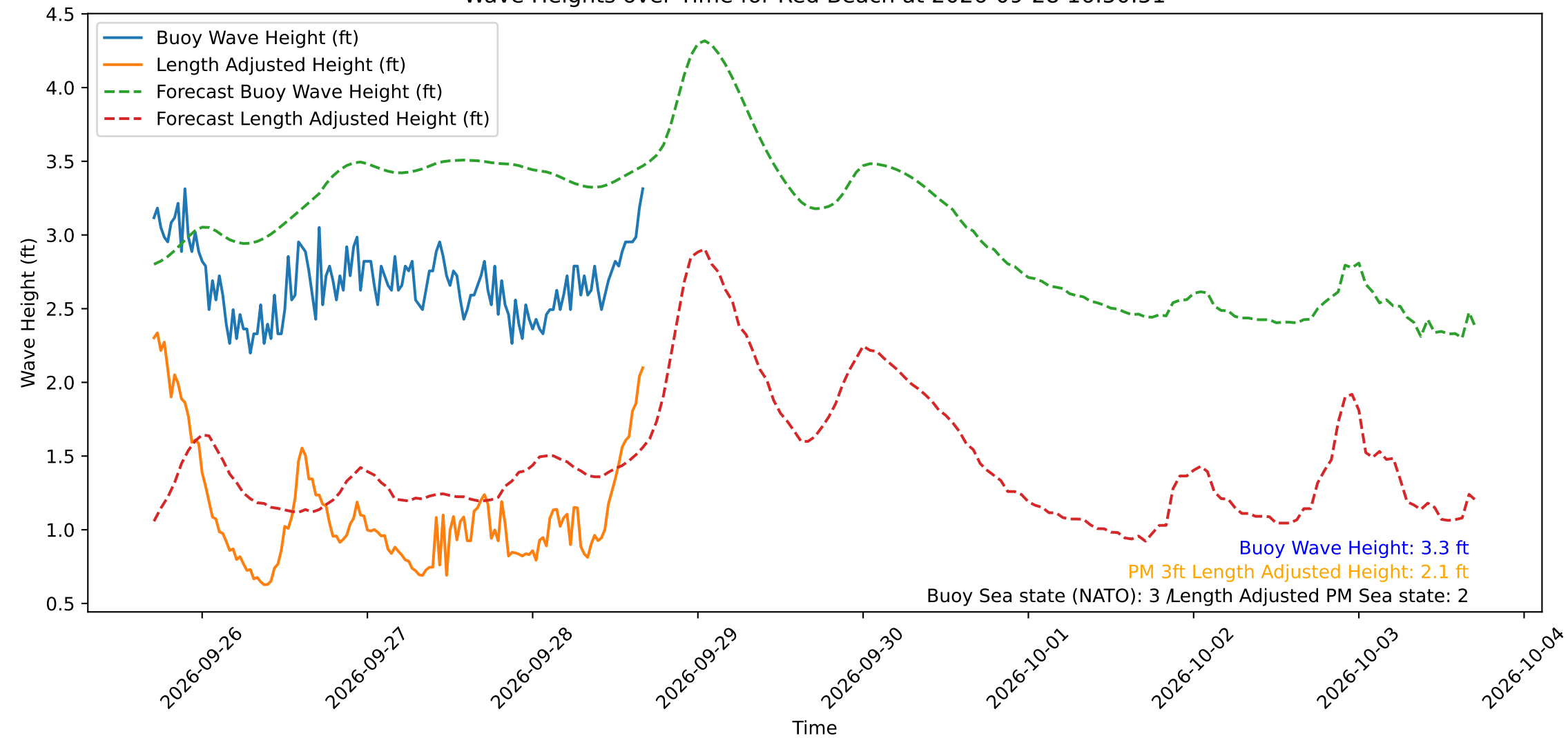
Wave Heights over Time for Red Beach at 2026-09-28 16:50:51
