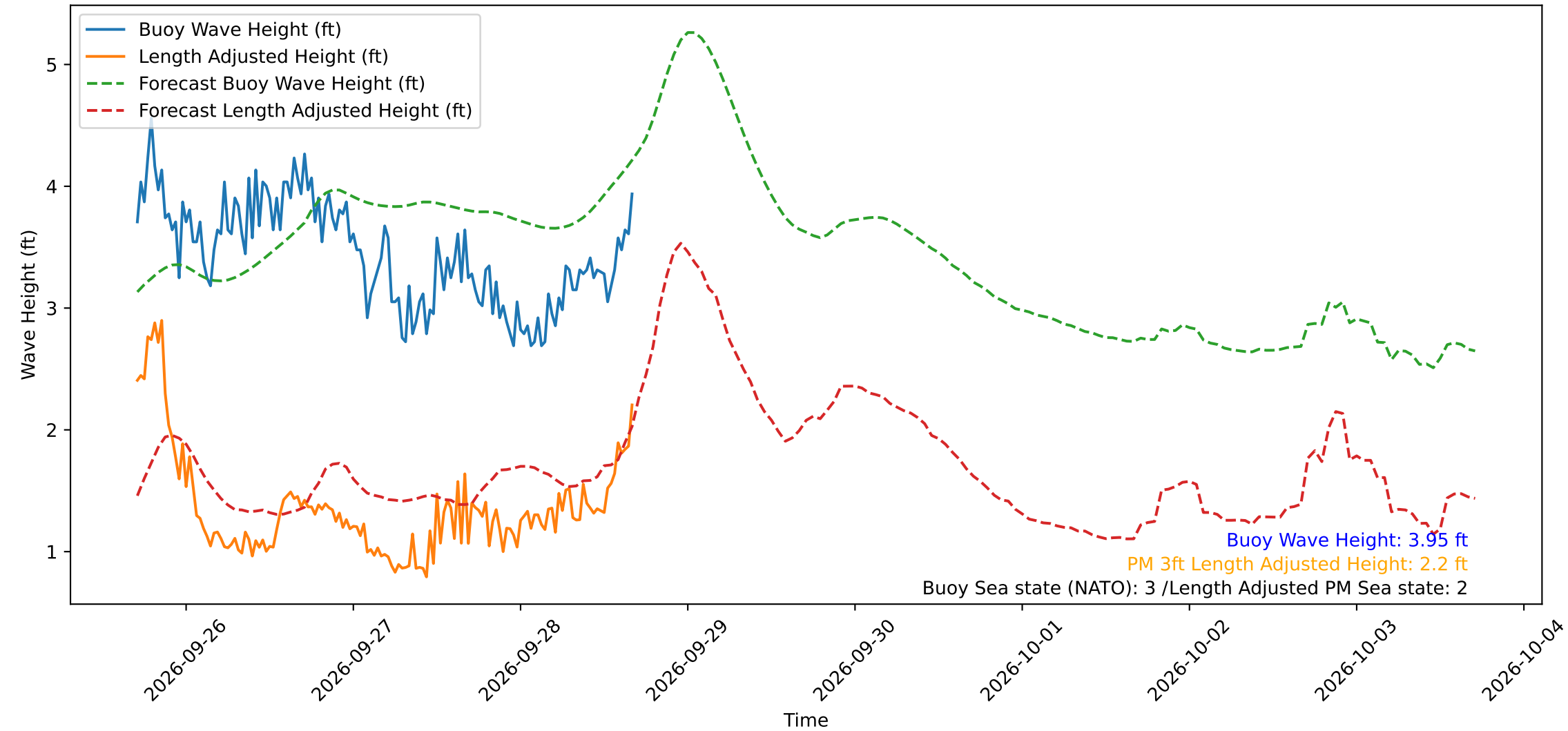
Wave Heights over Time for Green Beach at 2026-09-28 16:51:15
