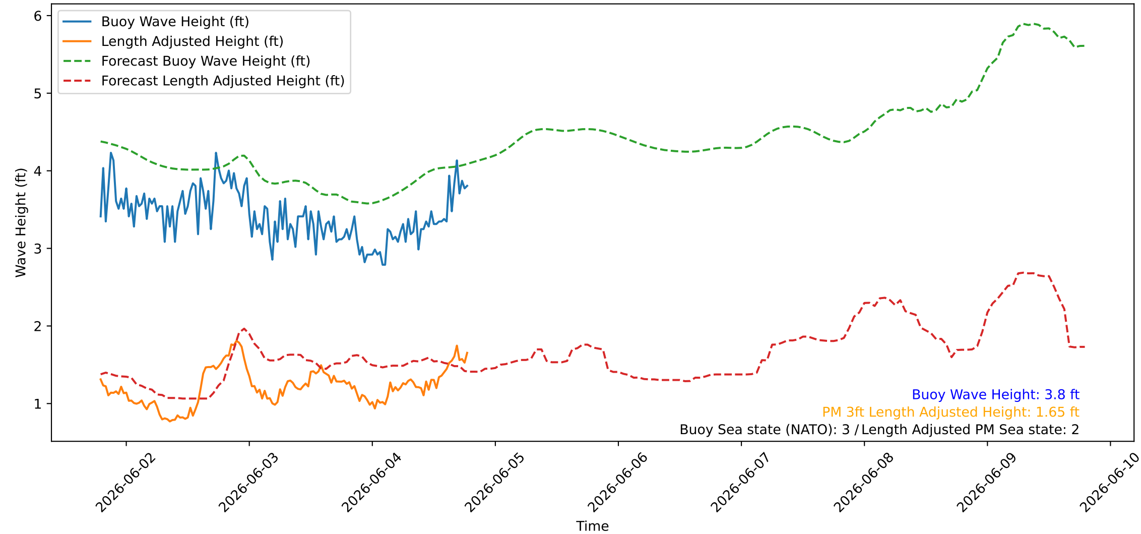
Wave Heights over Time for Green Beach at 2026-06-04 19:11:07
