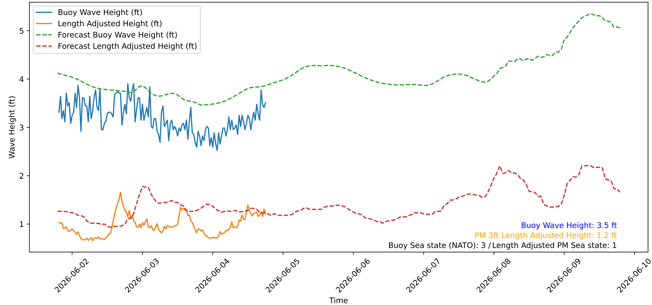
Wave Heights over Time for Red Beach at 2026-06-04 19:10:45
