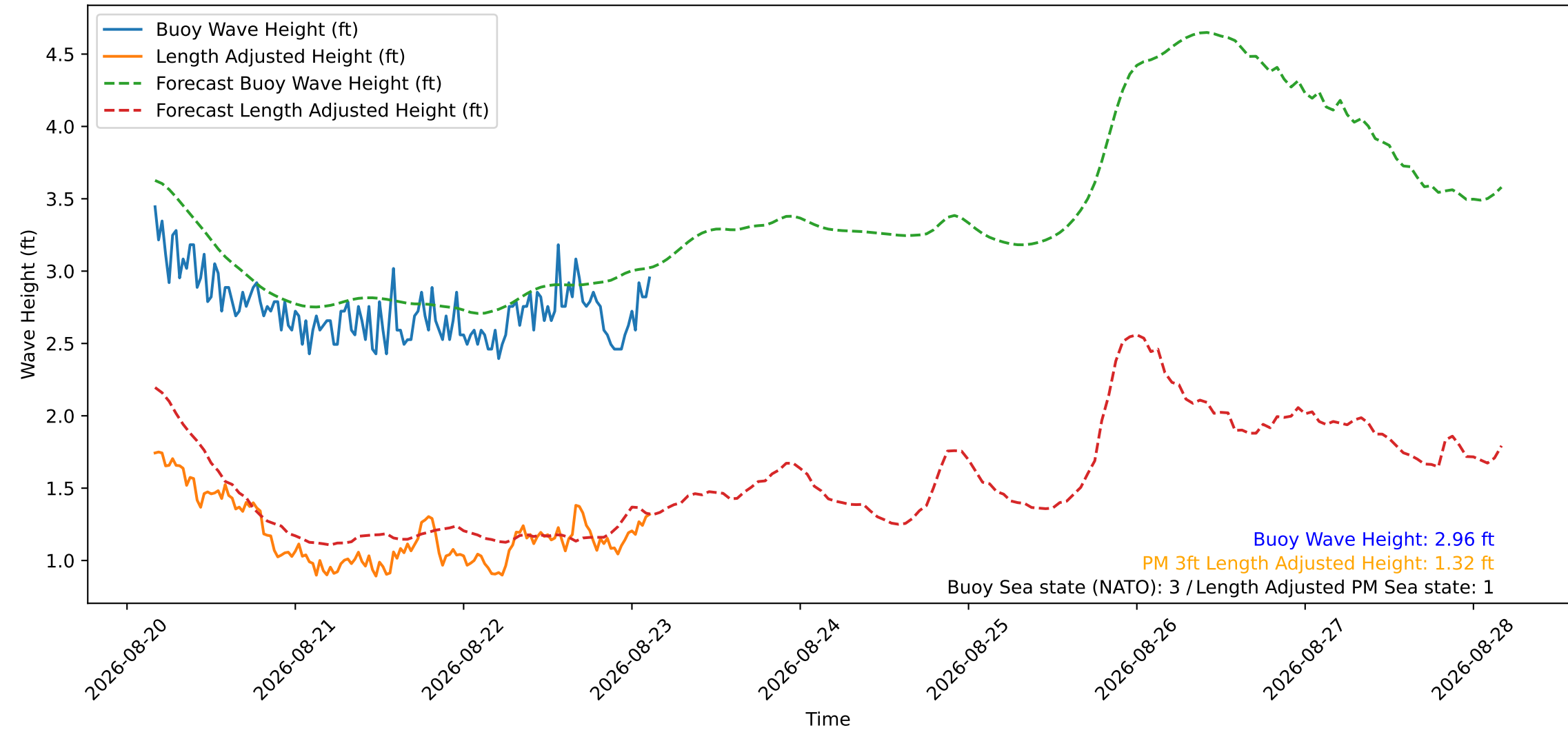
Wave Heights over Time for Green Beach at 2026-08-23 03:31:11
