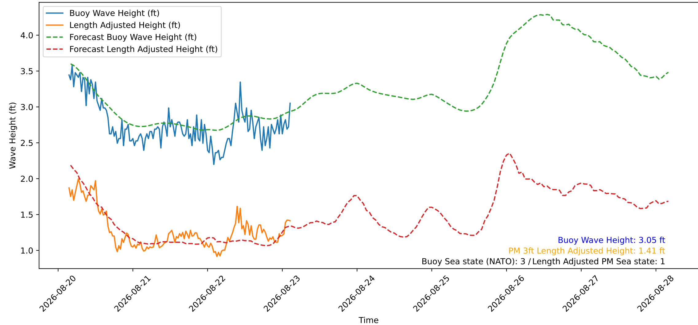
Wave Heights over Time for Oceanside Harbor at 2026-08-23 03:30:30
