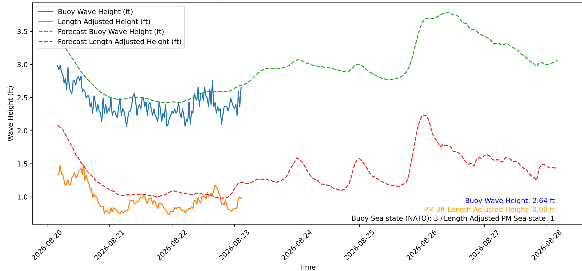
Wave Heights over Time for Red Beach at 2026-08-23 03:30:49
