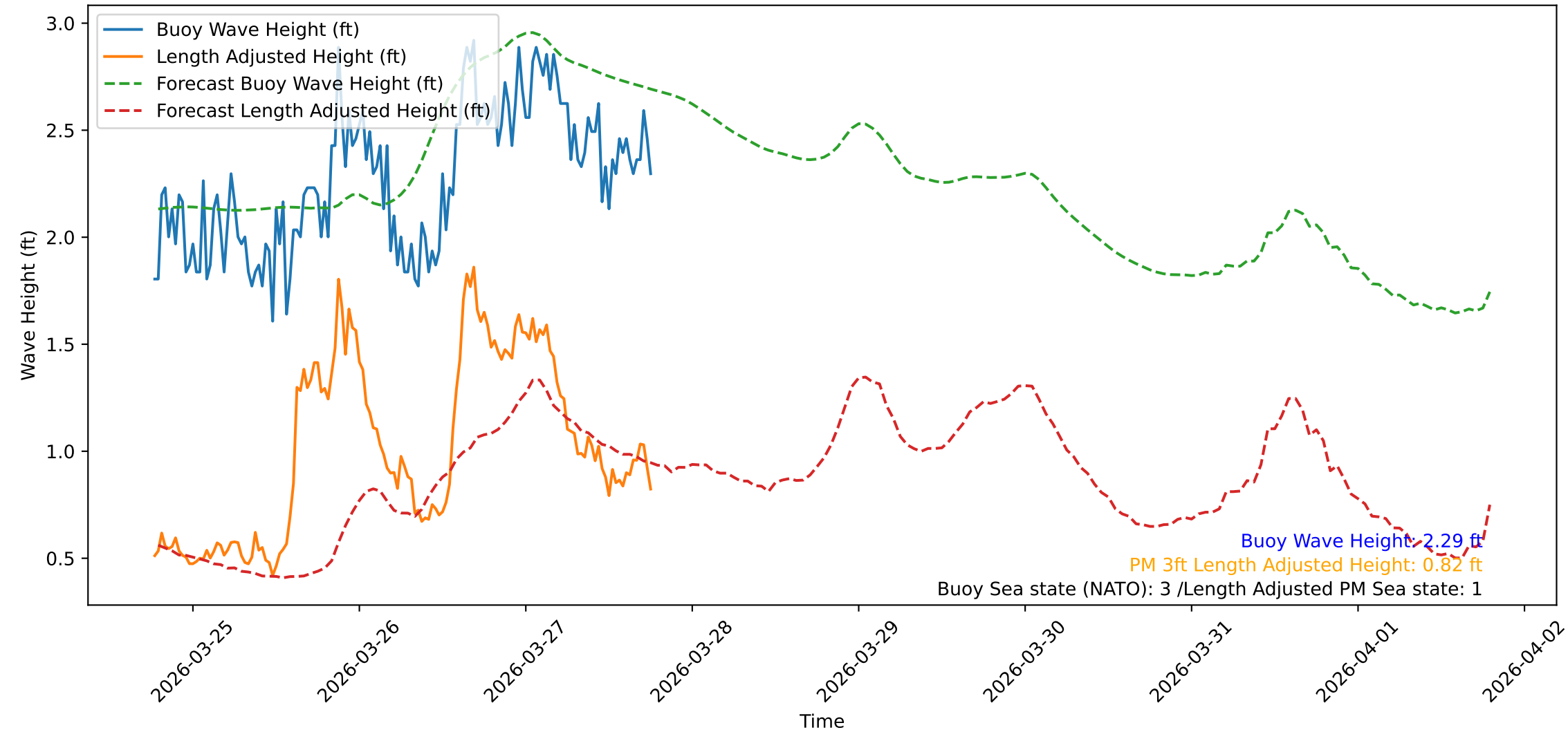
Wave Heights over Time for Oceanside Harbor at 2026-03-27 18:40:30
