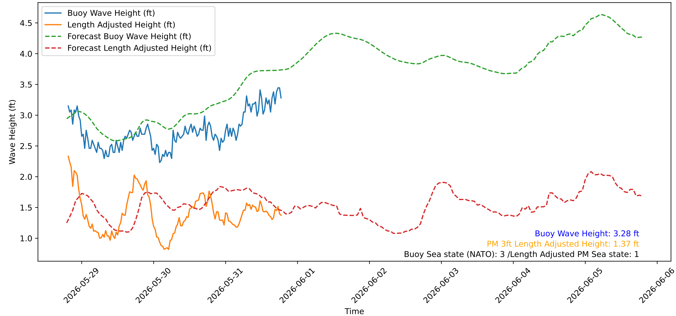
Wave Heights over Time for Red Beach at 2026-05-31 19:20:47
