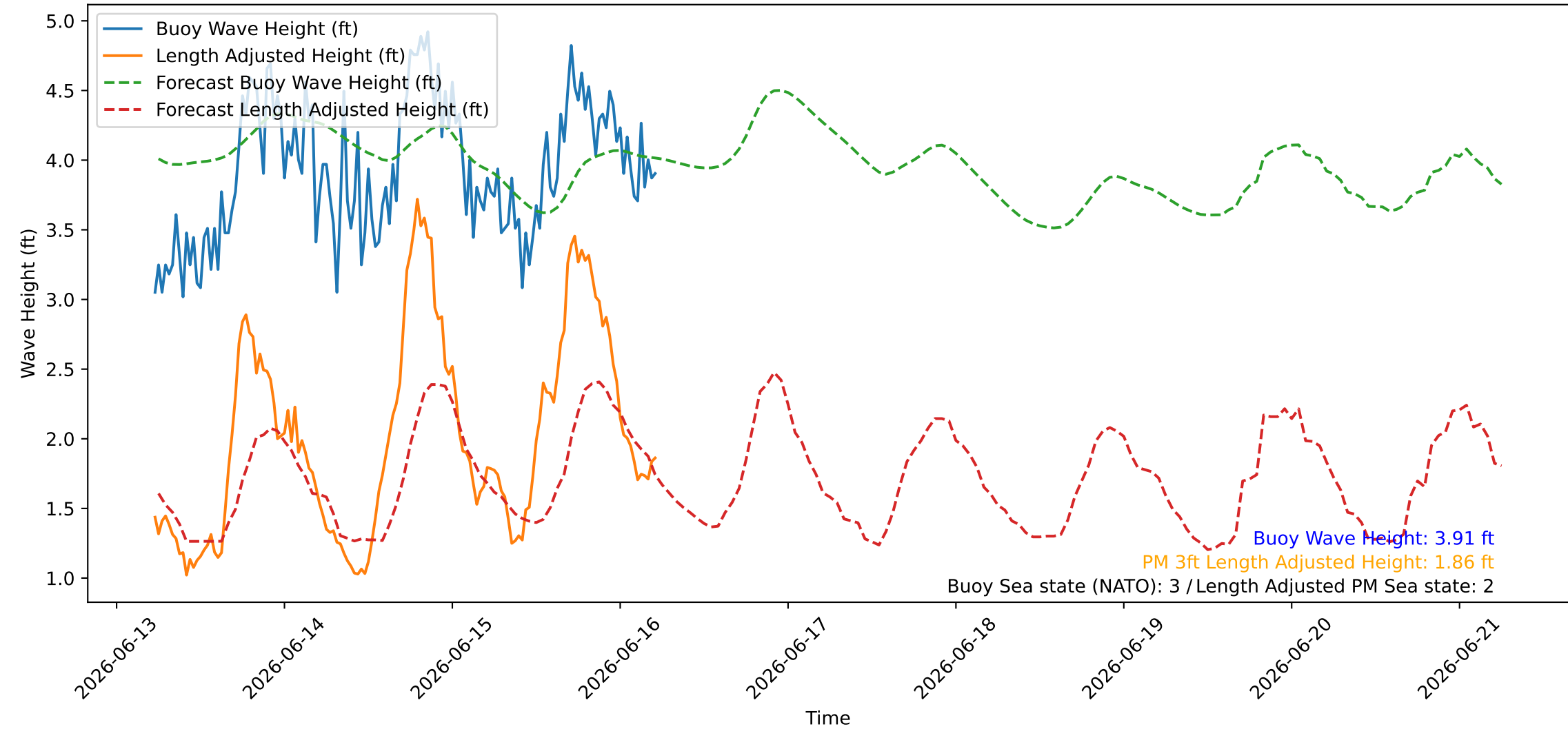
Wave Heights over Time for Green Beach at 2026-06-16 05:41:07
