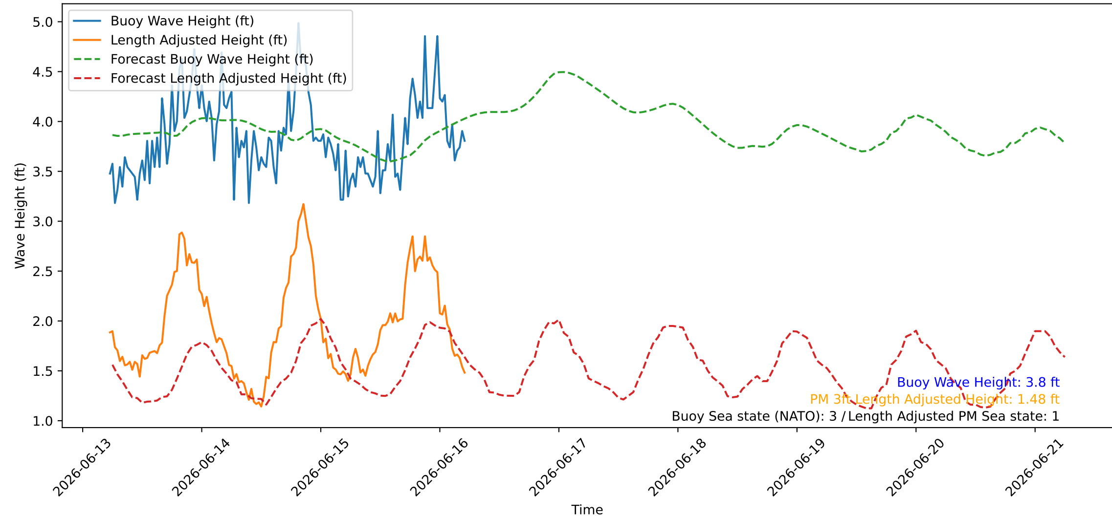
Wave Heights over Time for Oceanside Harbor at 2026-06-16 05:40:25
