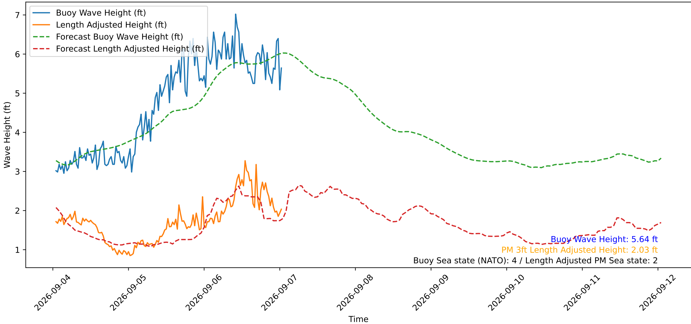
Wave Heights over Time for Oceanside Harbor at 2026-09-07 01:10:29
