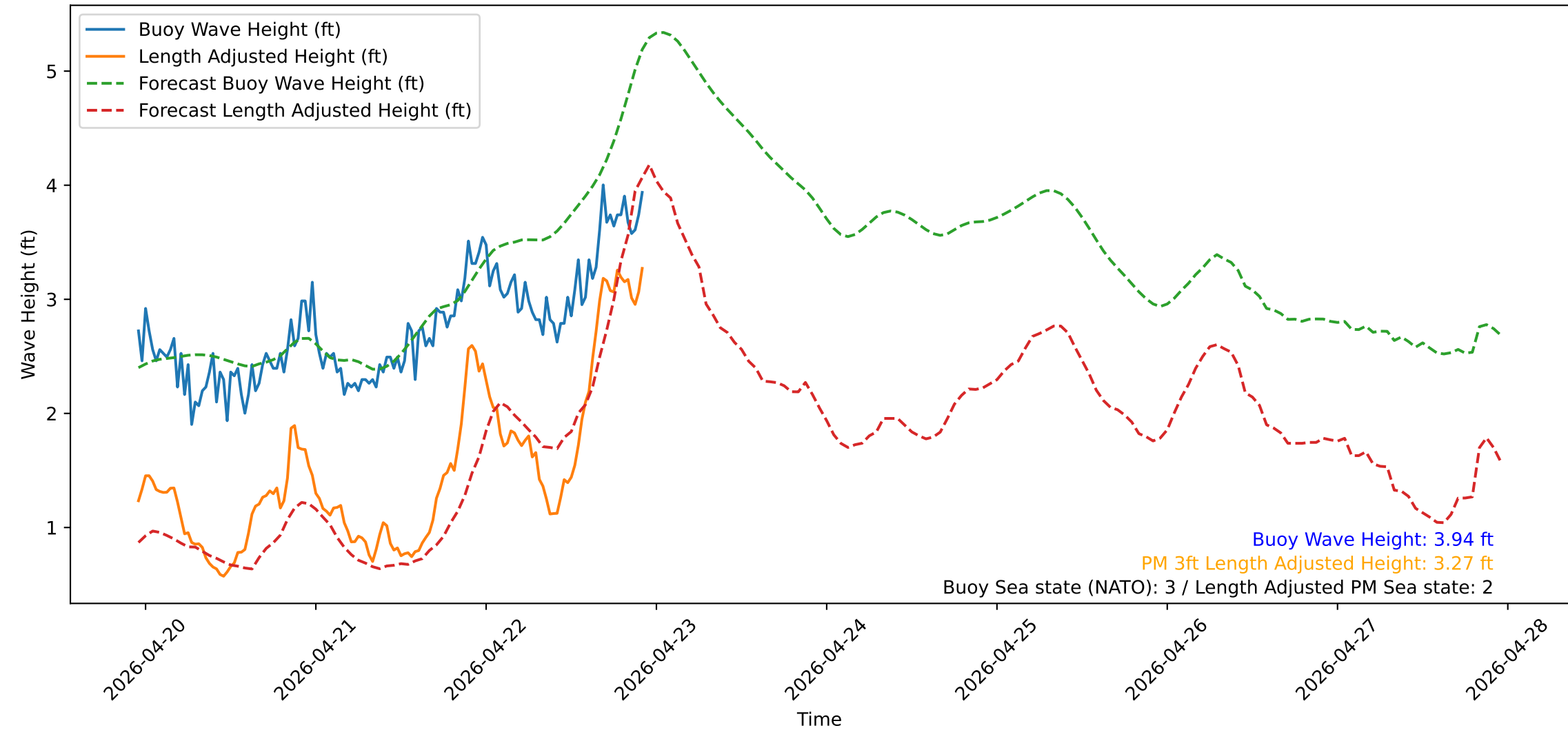
Wave Heights over Time for Green Beach at 2026-04-22 23:11:13
