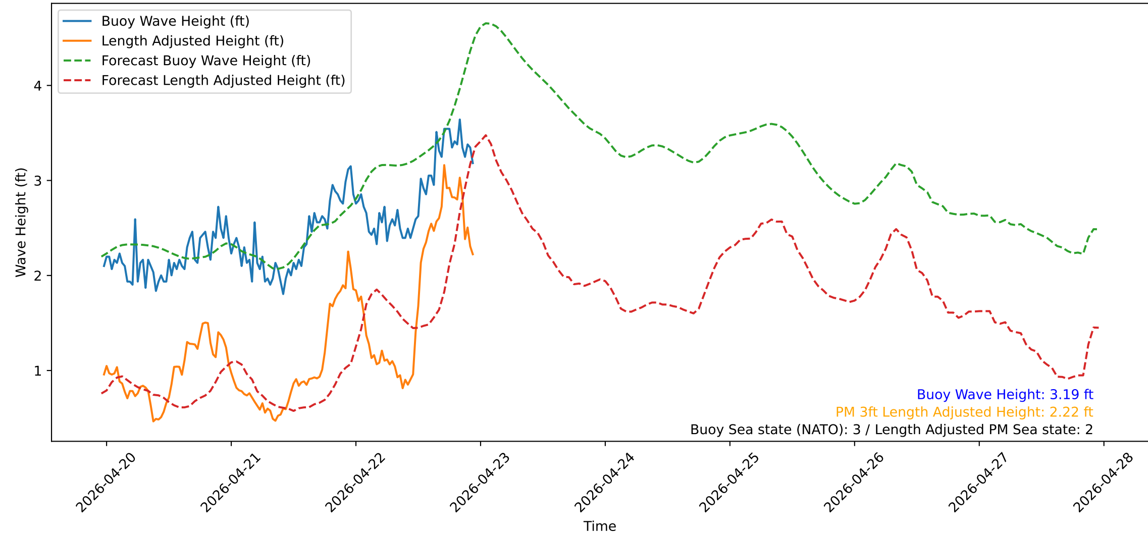
Wave Heights over Time for Red Beach at 2026-04-22 23:10:50
