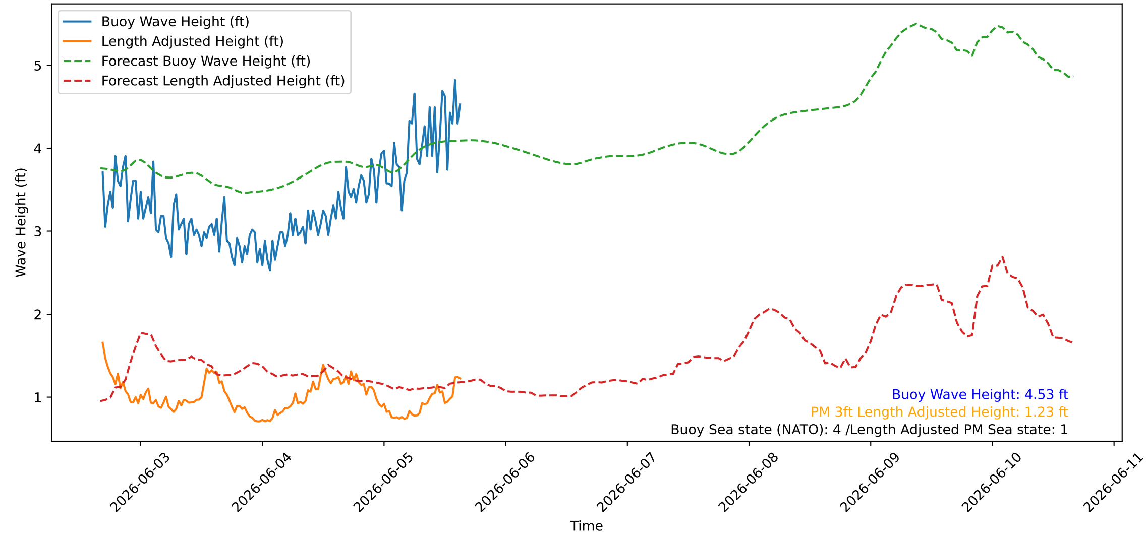
Wave Heights over Time for Red Beach at 2026-06-05 16:00:45
