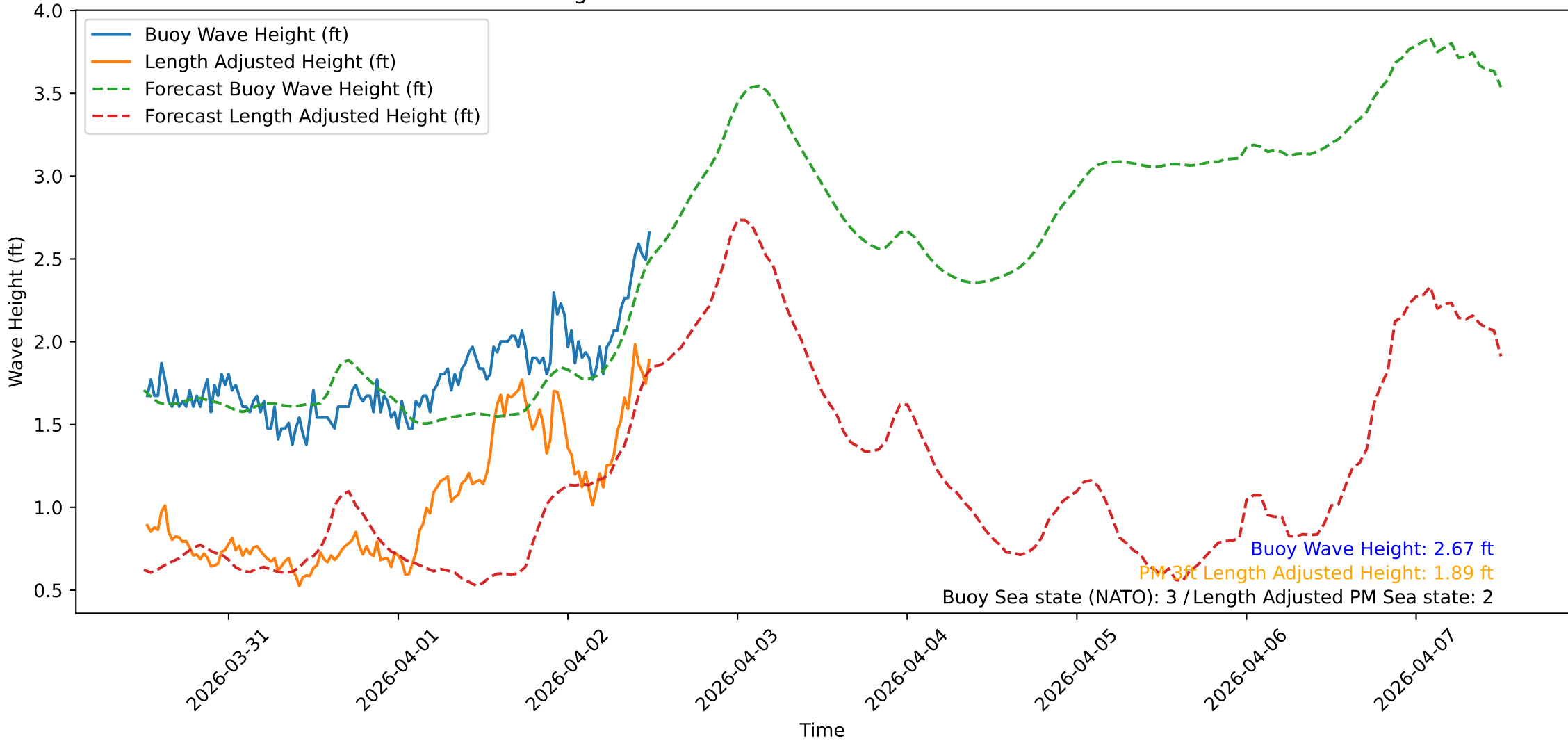
Wave Heights over Time for Red Beach at 2026-04-02 12:20:47
