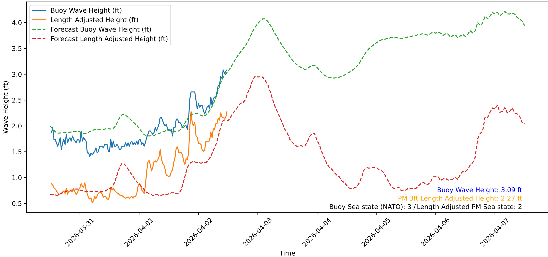
Wave Heights over Time for Green Beach at 2026-04-02 12:21:10
