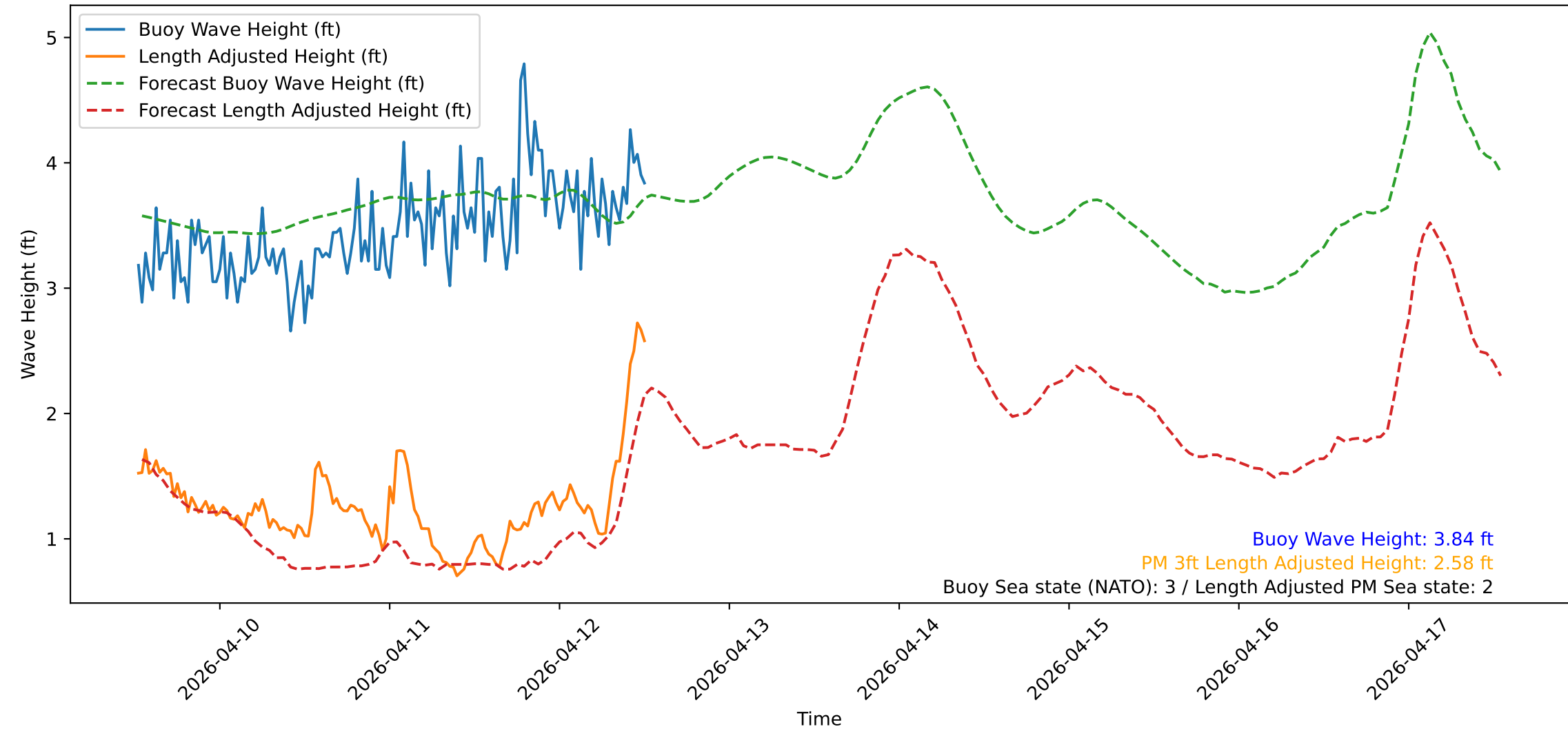
Wave Heights over Time for Oceanside Harbor at 2026-04-12 12:40:30
