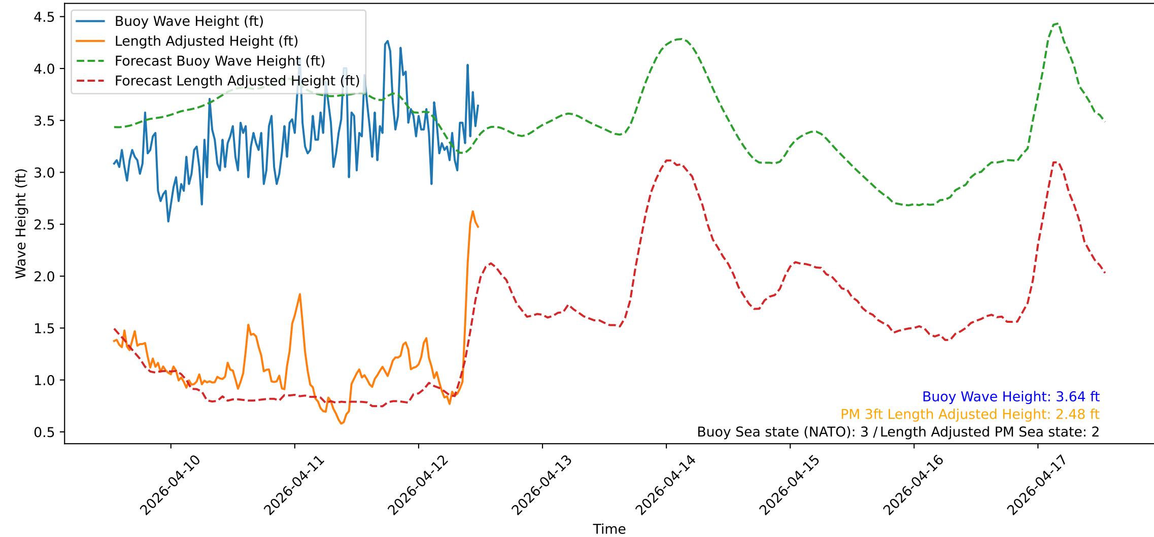
Wave Heights over Time for Red Beach at 2026-04-12 12:40:49
