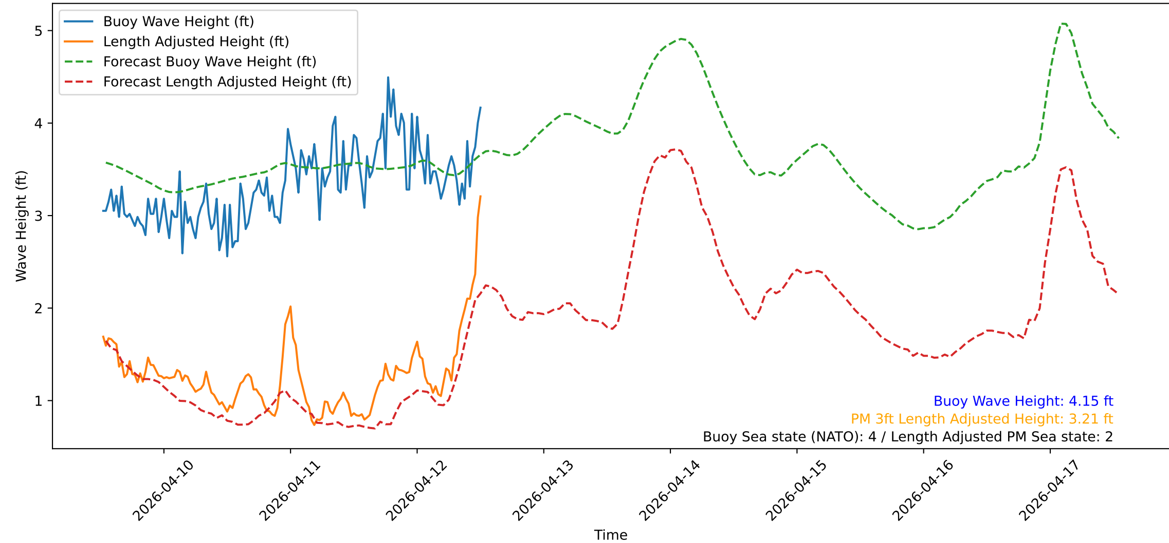
Wave Heights over Time for Green Beach at 2026-04-12 12:41:12
