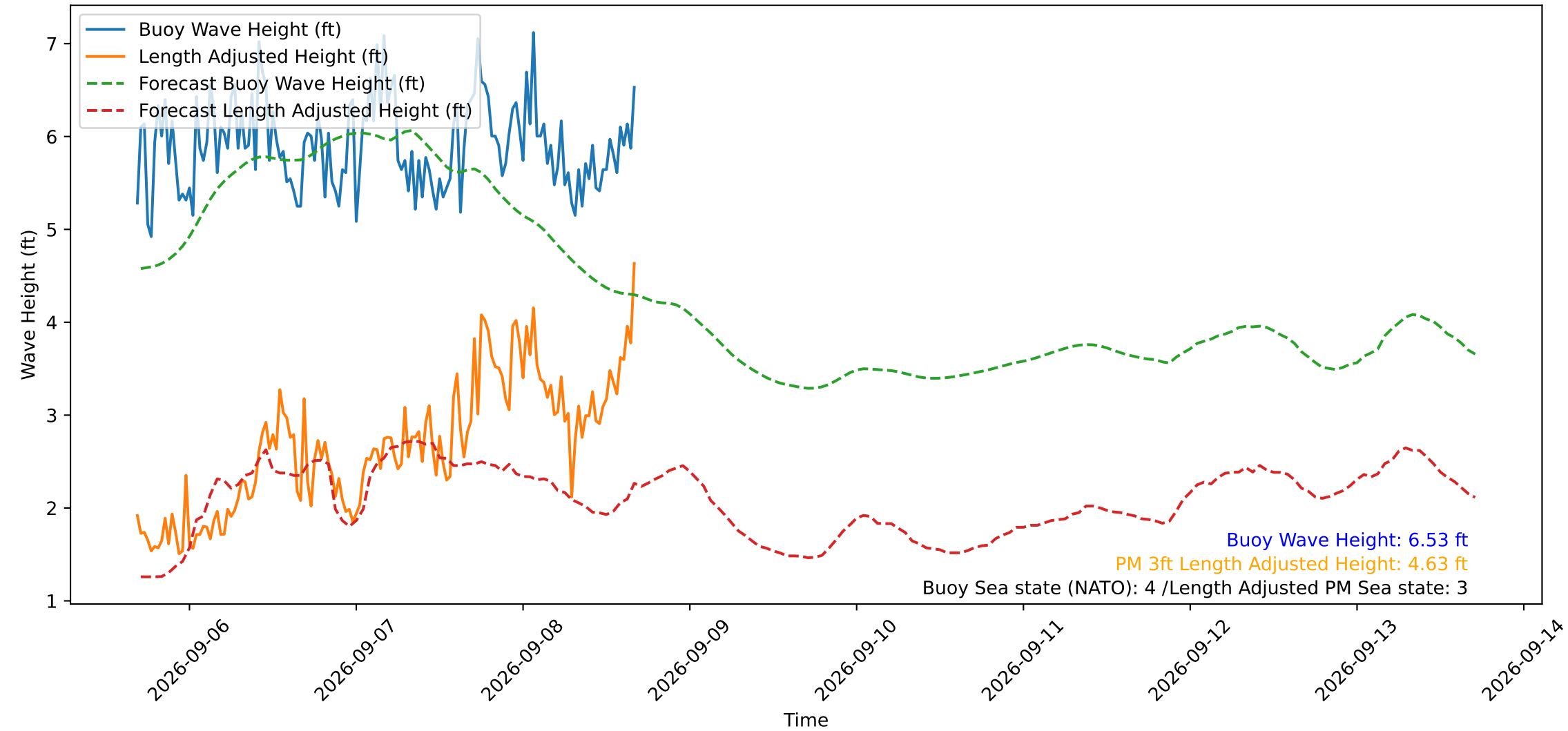
Wave Heights over Time for Oceanside Harbor at 2026-09-08 16:40:29
