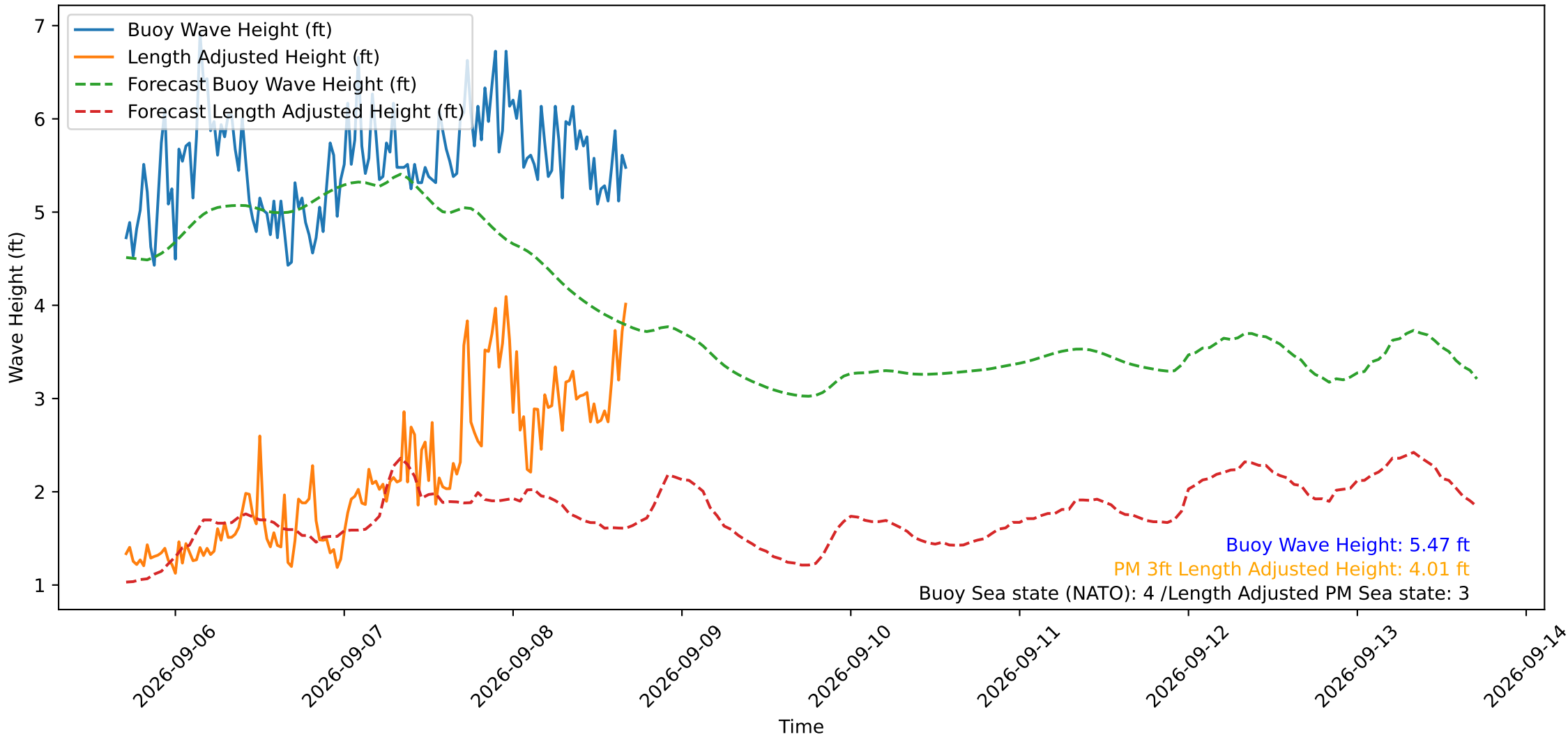
Wave Heights over Time for Red Beach at 2026-09-08 16:40:49
