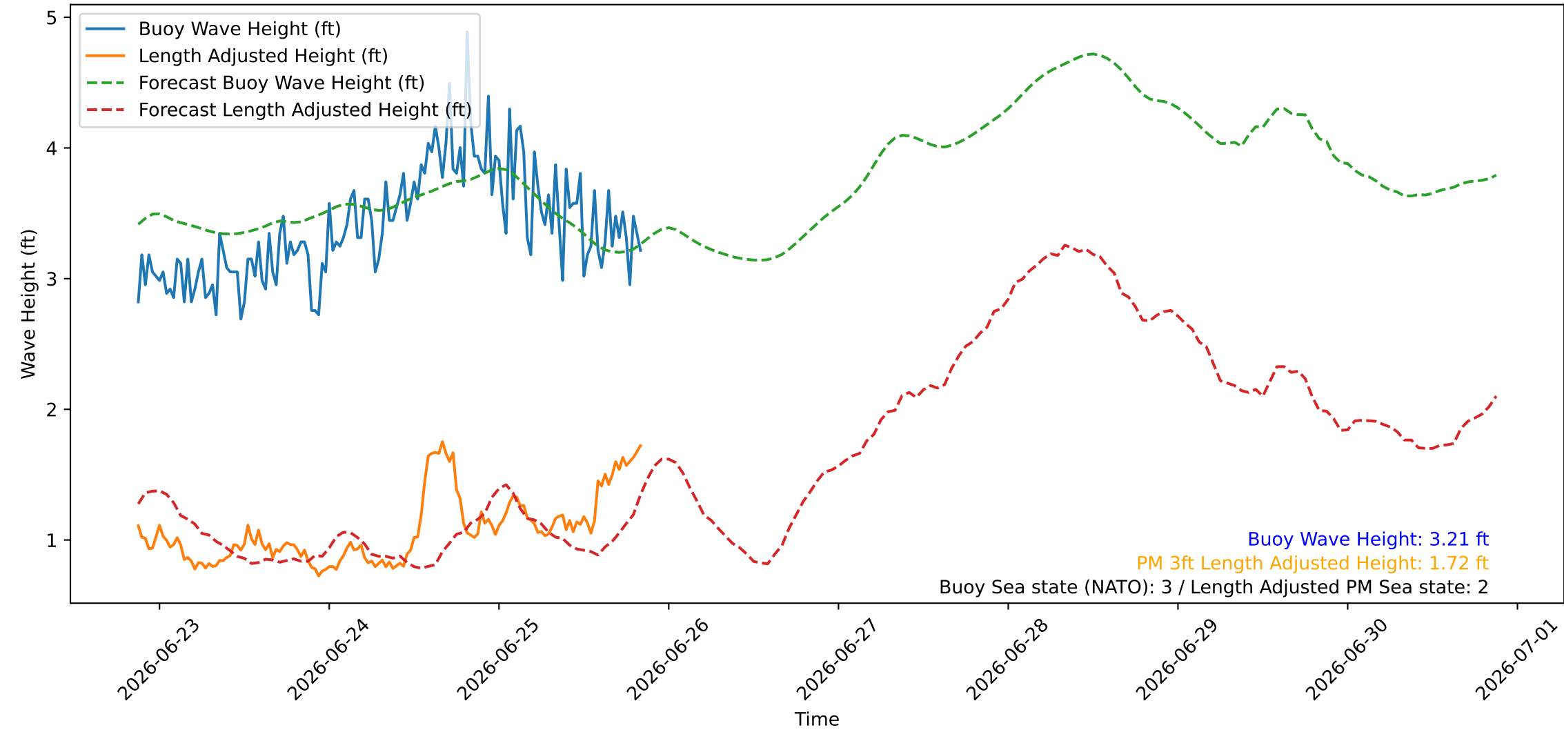
Wave Heights over Time for Oceanside Harbor at 2026-06-25 20:50:26
