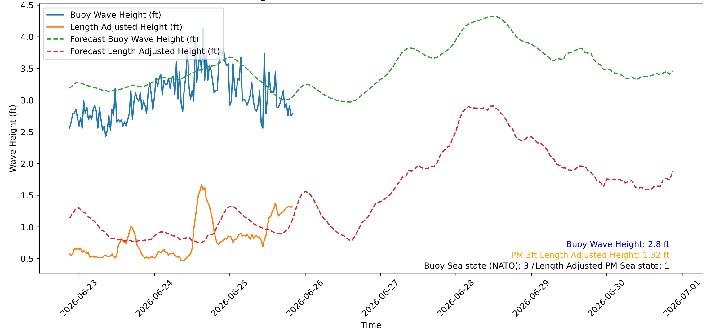
Wave Heights over Time for Red Beach at 2026-06-25 20:50:46
