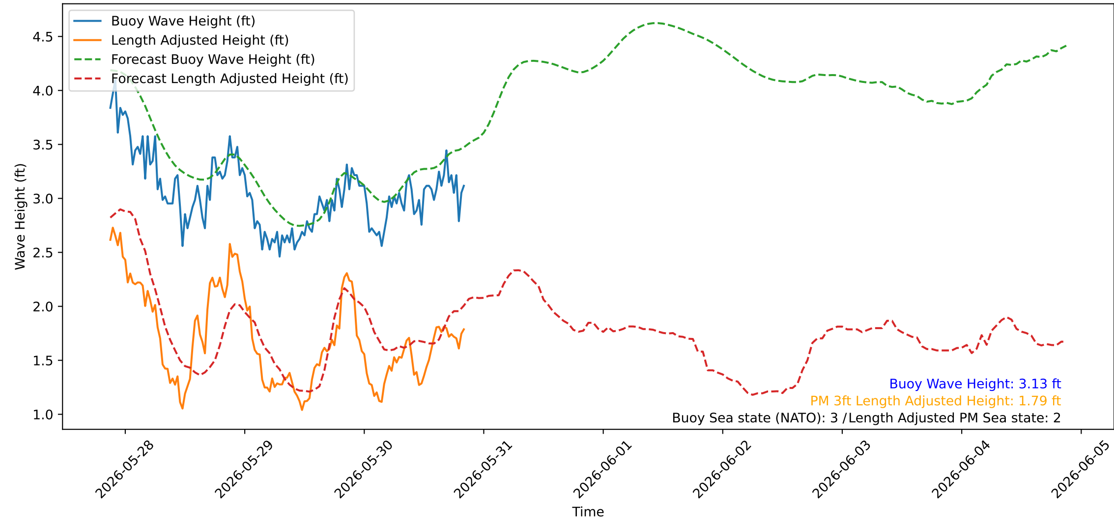
Wave Heights over Time for Green Beach at 2026-05-30 21:01:06
