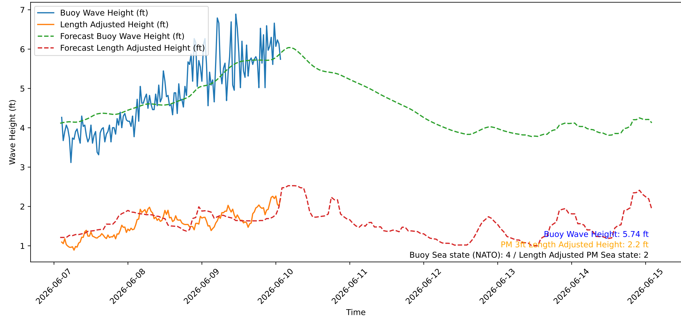
Wave Heights over Time for Green Beach at 2026-06-10 02:21:11
