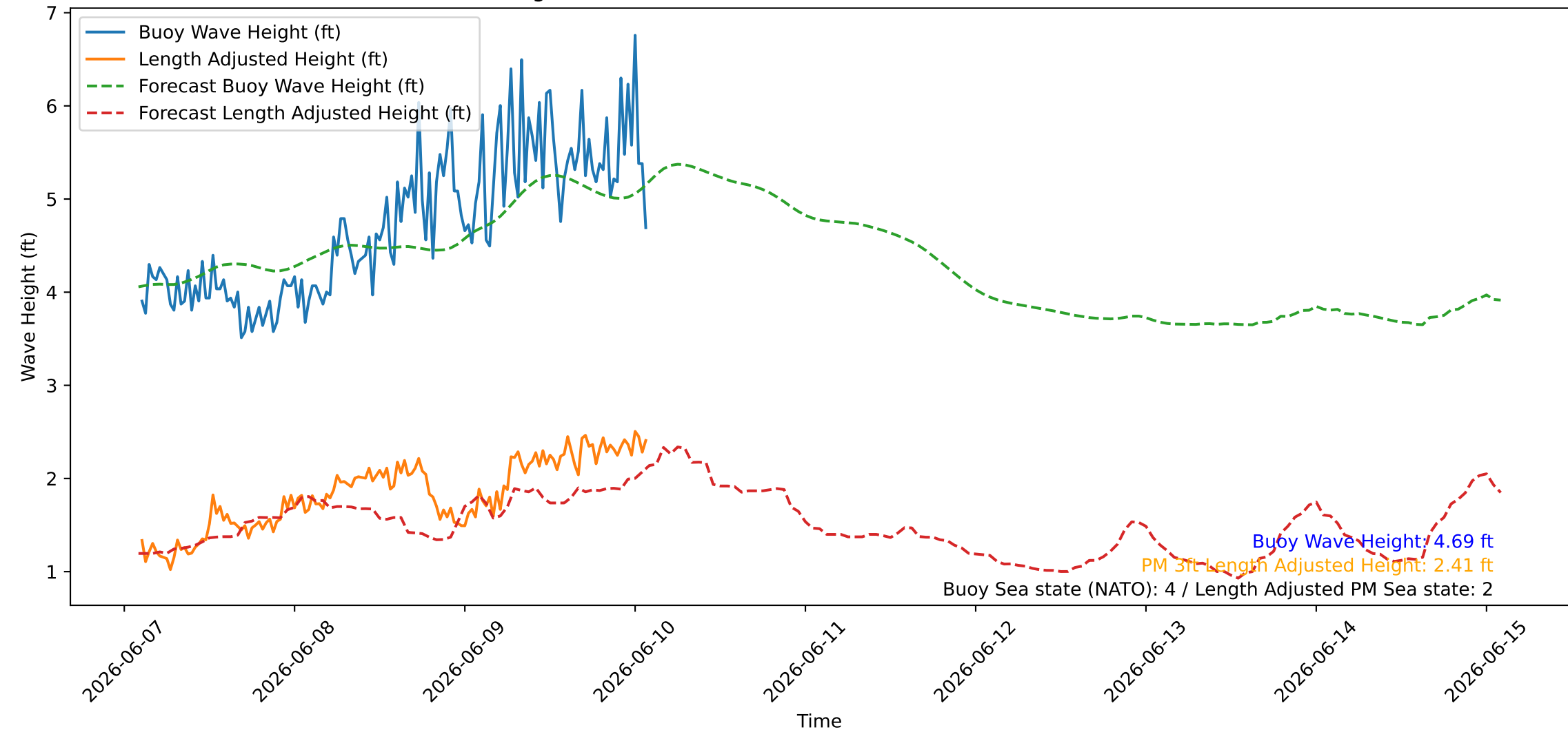
Wave Heights over Time for Oceanside Harbor at 2026-06-10 02:20:27
