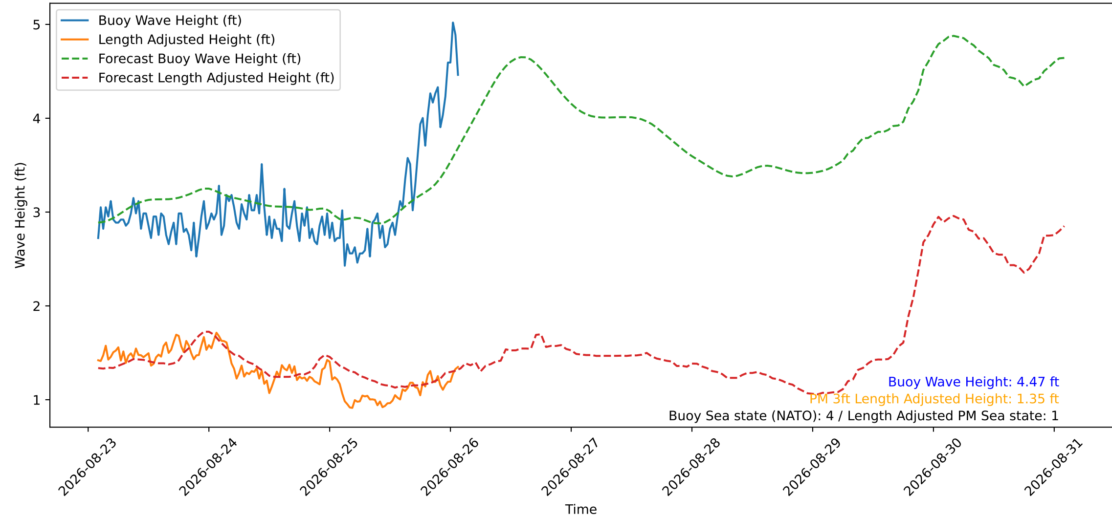
Wave Heights over Time for Oceanside Harbor at 2026-08-26 02:10:29
