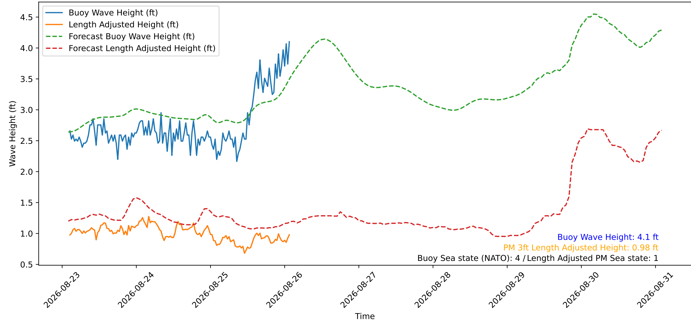
Wave Heights over Time for Red Beach at 2026-08-26 02:10:48
