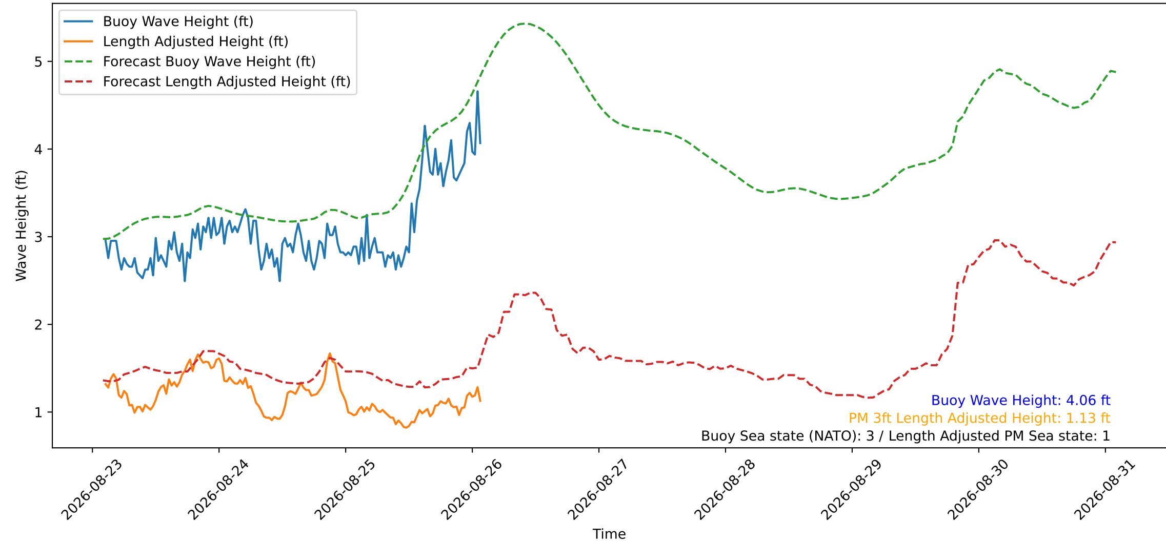
Wave Heights over Time for Green Beach at 2026-08-26 02:11:10
