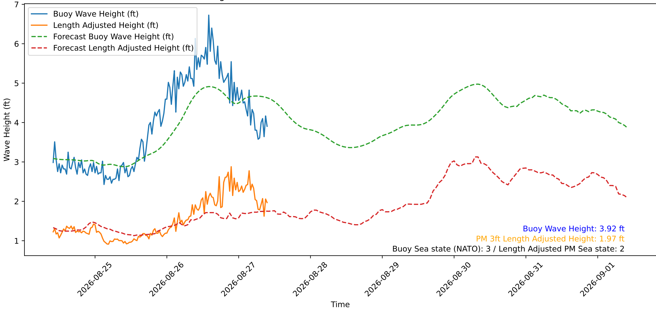
Wave Heights over Time for Oceanside Harbor at 2026-08-27 10:10:55
