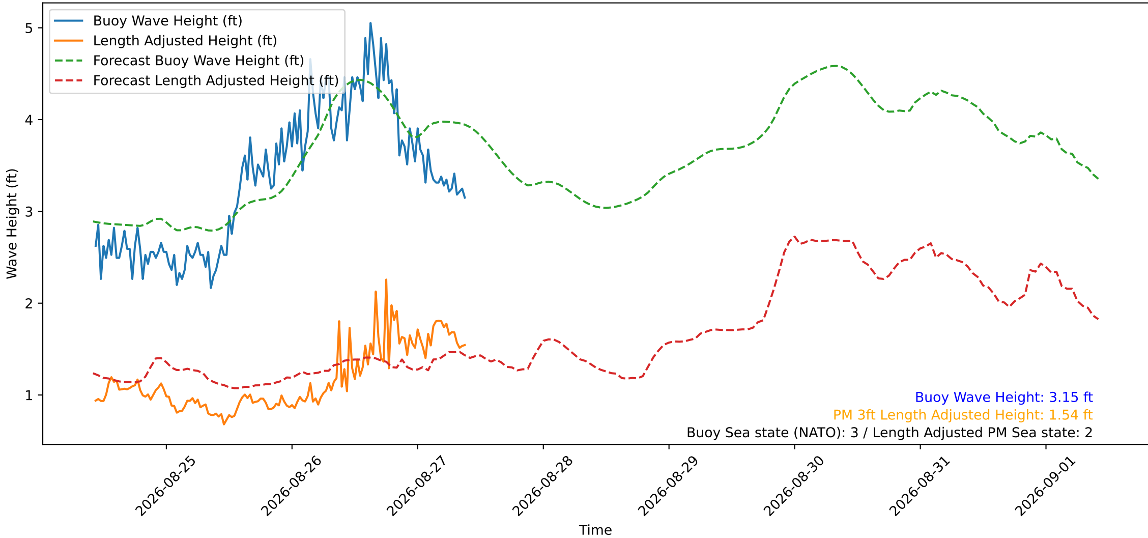
Wave Heights over Time for Red Beach at 2026-08-27 10:11:15
