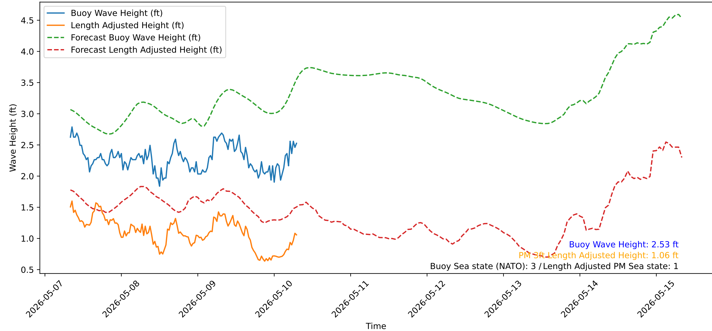
Wave Heights over Time for Green Beach at 2026-05-10 08:01:18
