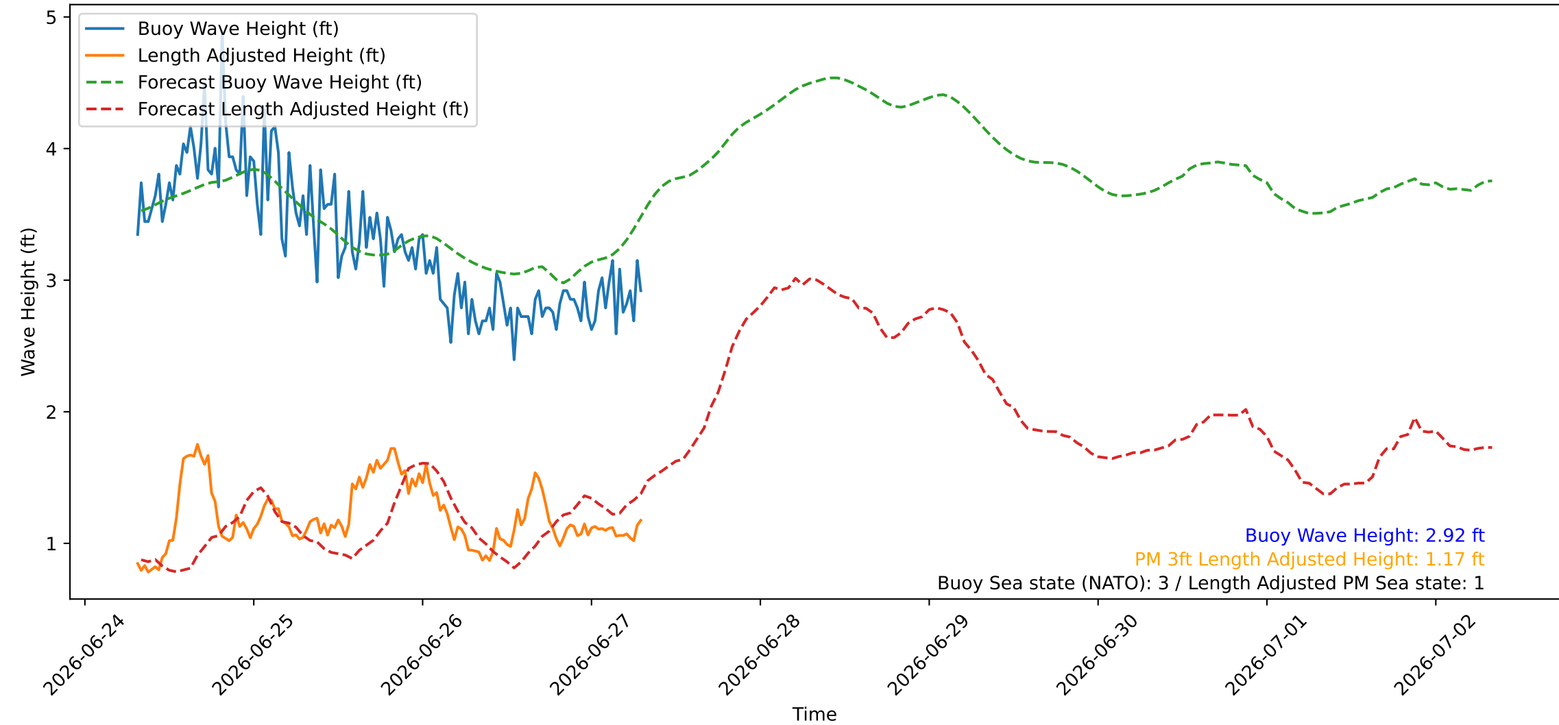
Wave Heights over Time for Oceanside Harbor at 2026-06-27 07:40:26
