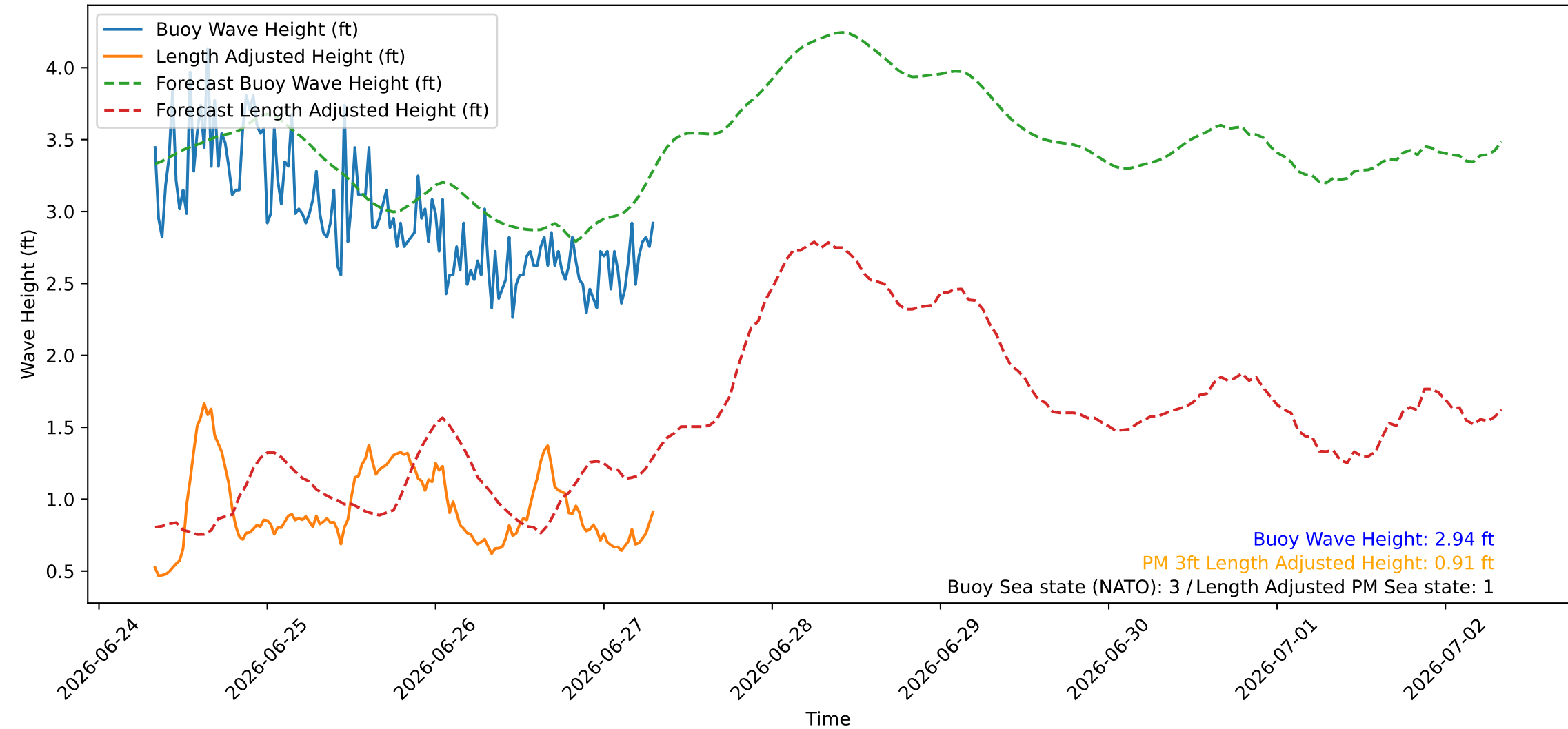
Wave Heights over Time for Red Beach at 2026-06-27 07:40:45
