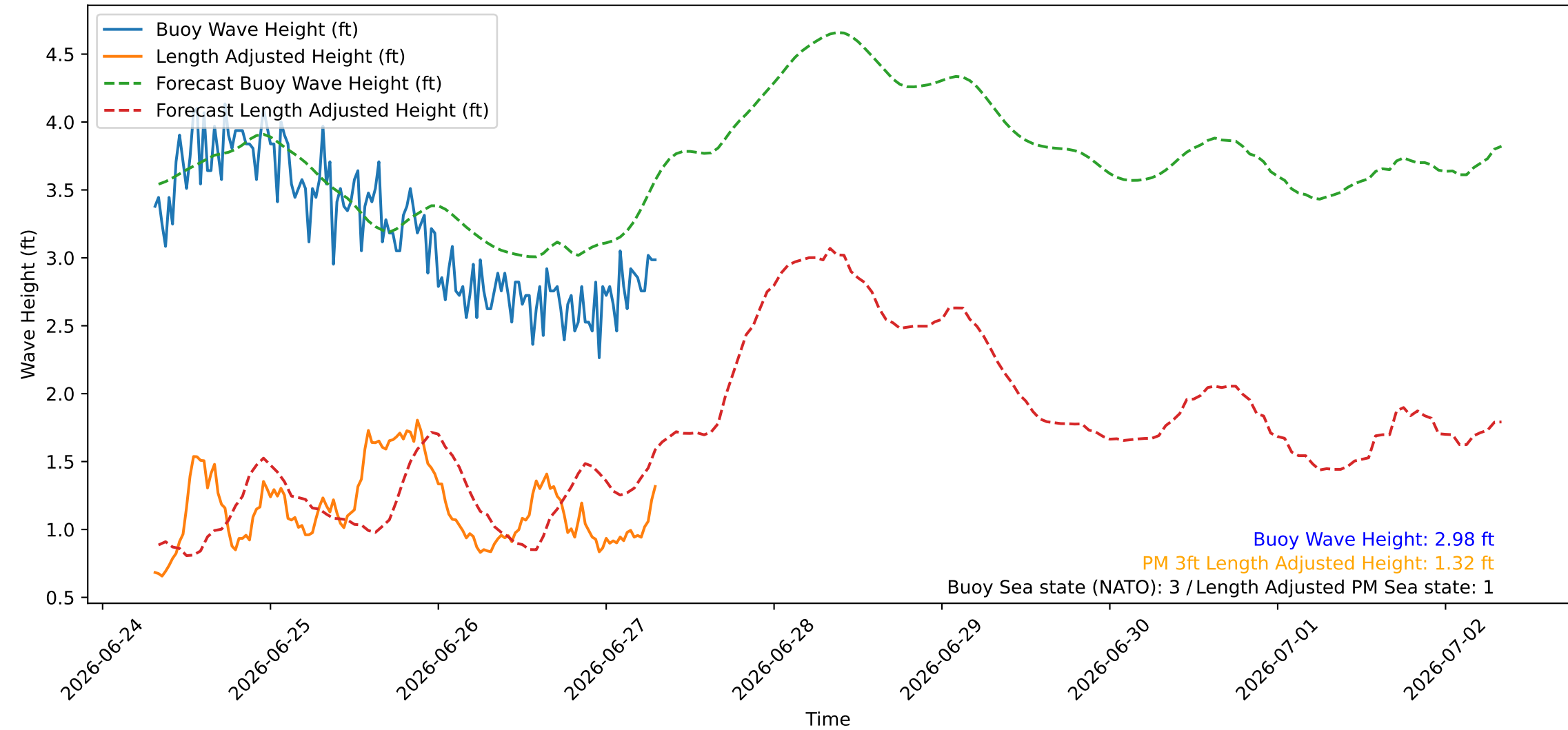
Wave Heights over Time for Green Beach at 2026-06-27 07:41:08
