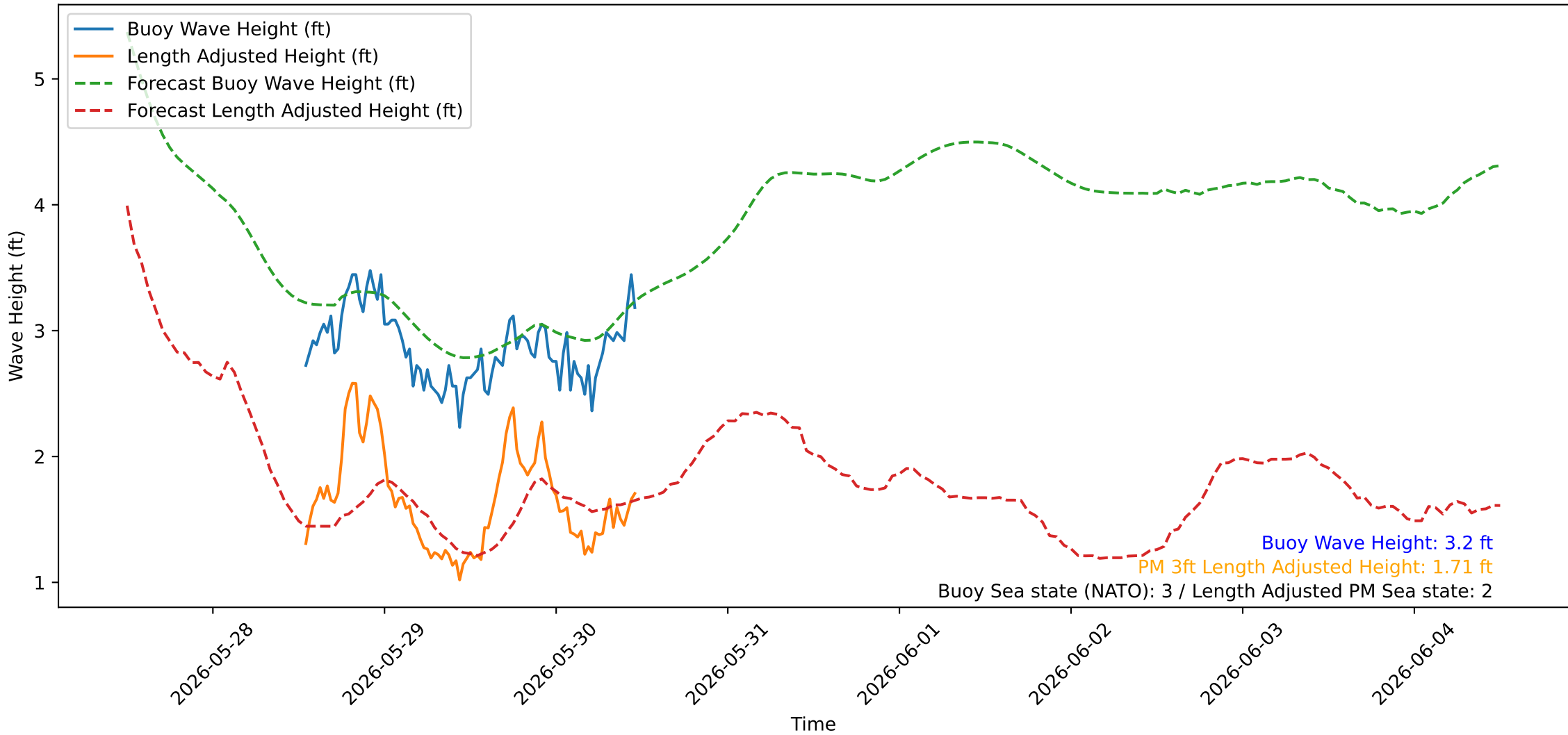
Wave Heights over Time for Oceanside Harbor at 2026-05-30 11:40:23
