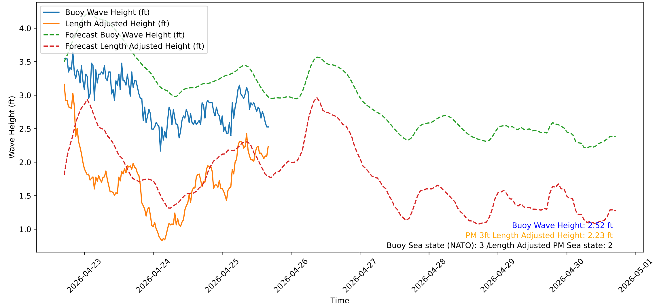
Wave Heights over Time for Red Beach at 2026-04-25 16:50:52
