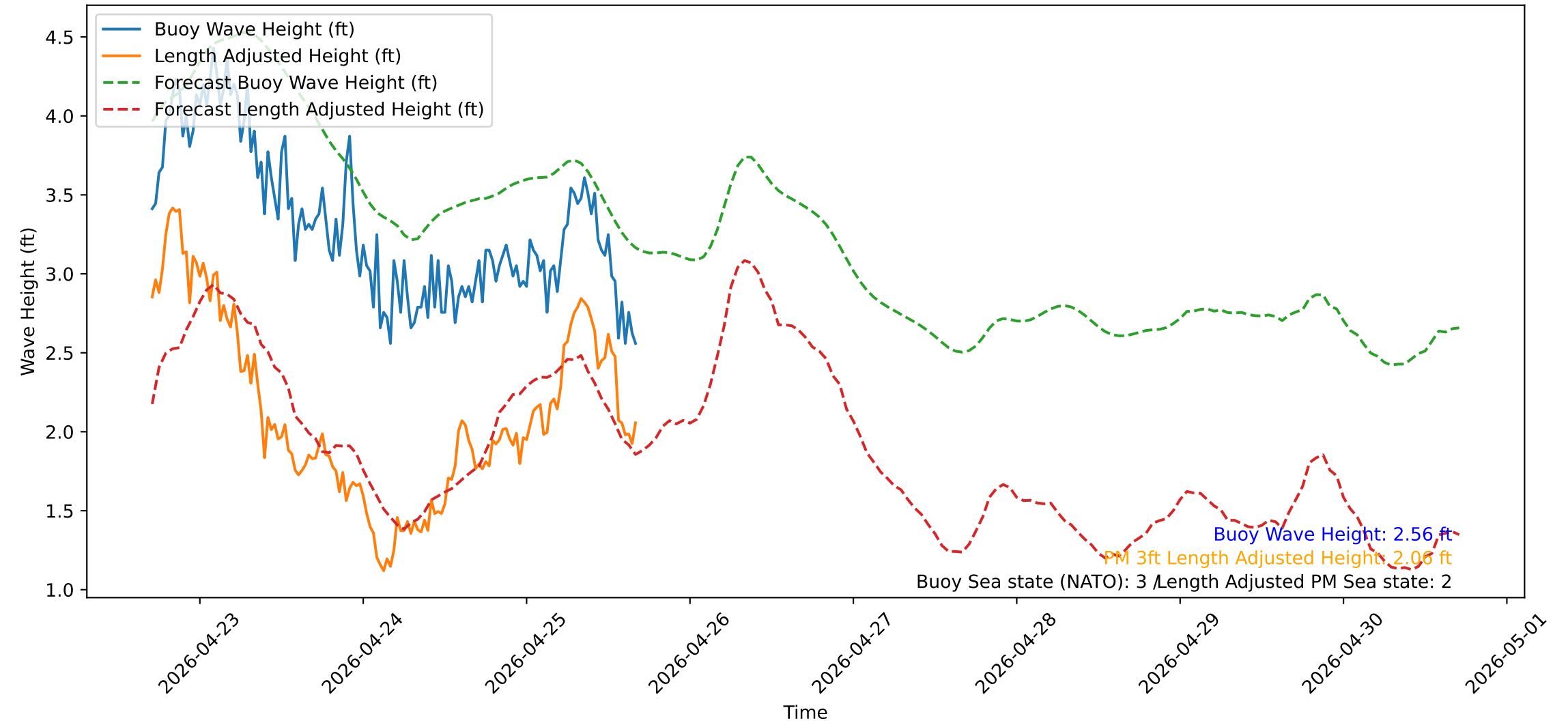
Wave Heights over Time for Oceanside Harbor at 2026-04-25 16:50:32
