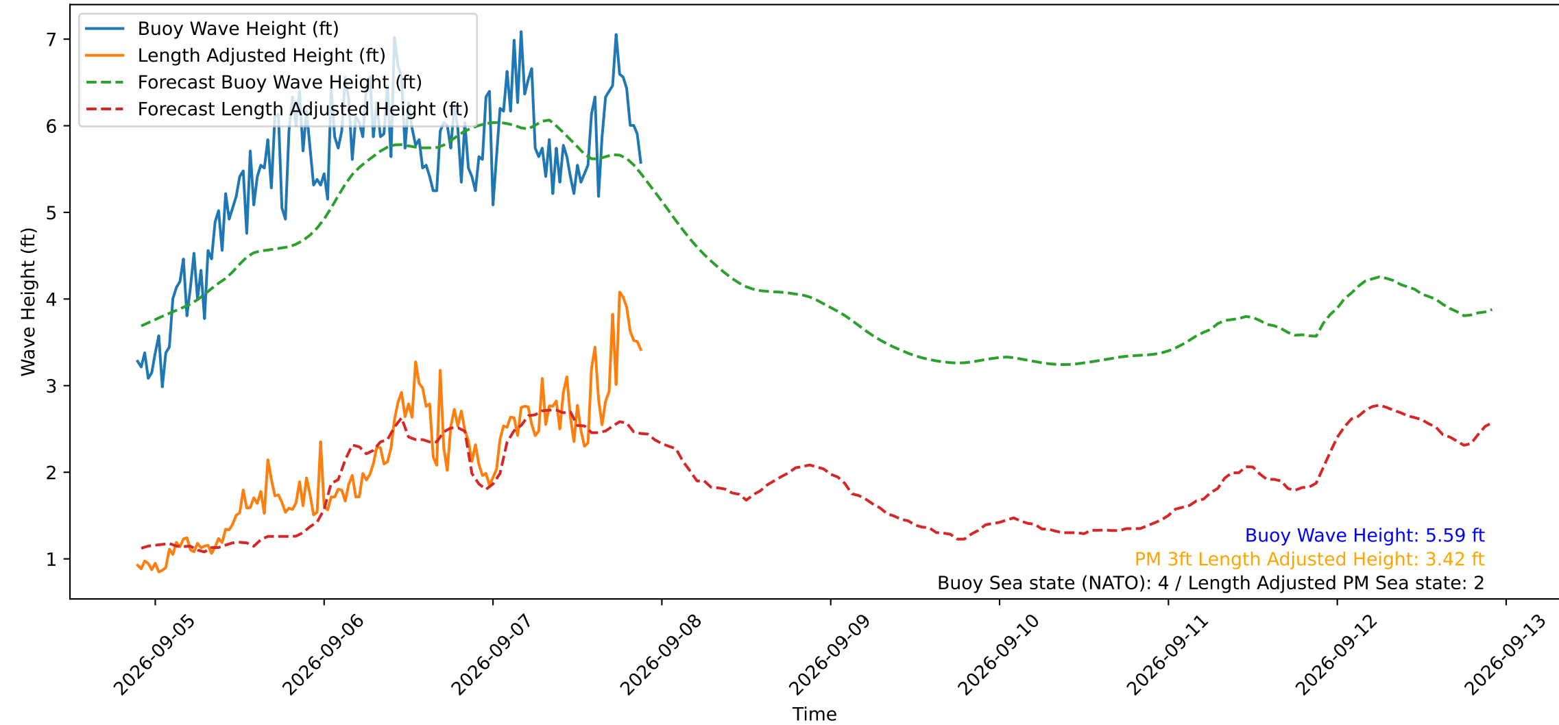
Wave Heights over Time for Oceanside Harbor at 2026-09-07 21:40:29
