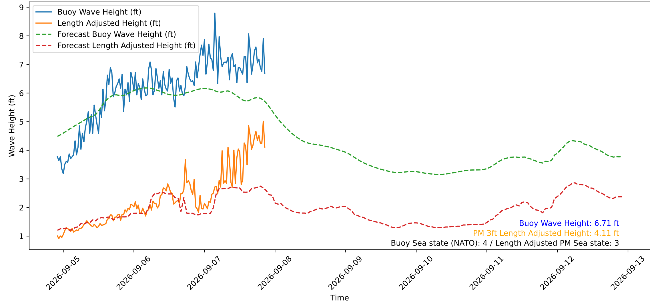
Wave Heights over Time for Green Beach at 2026-09-07 21:41:12
