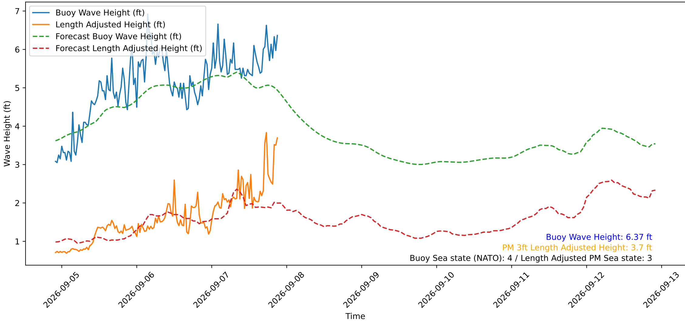
Wave Heights over Time for Red Beach at 2026-09-07 21:40:49
