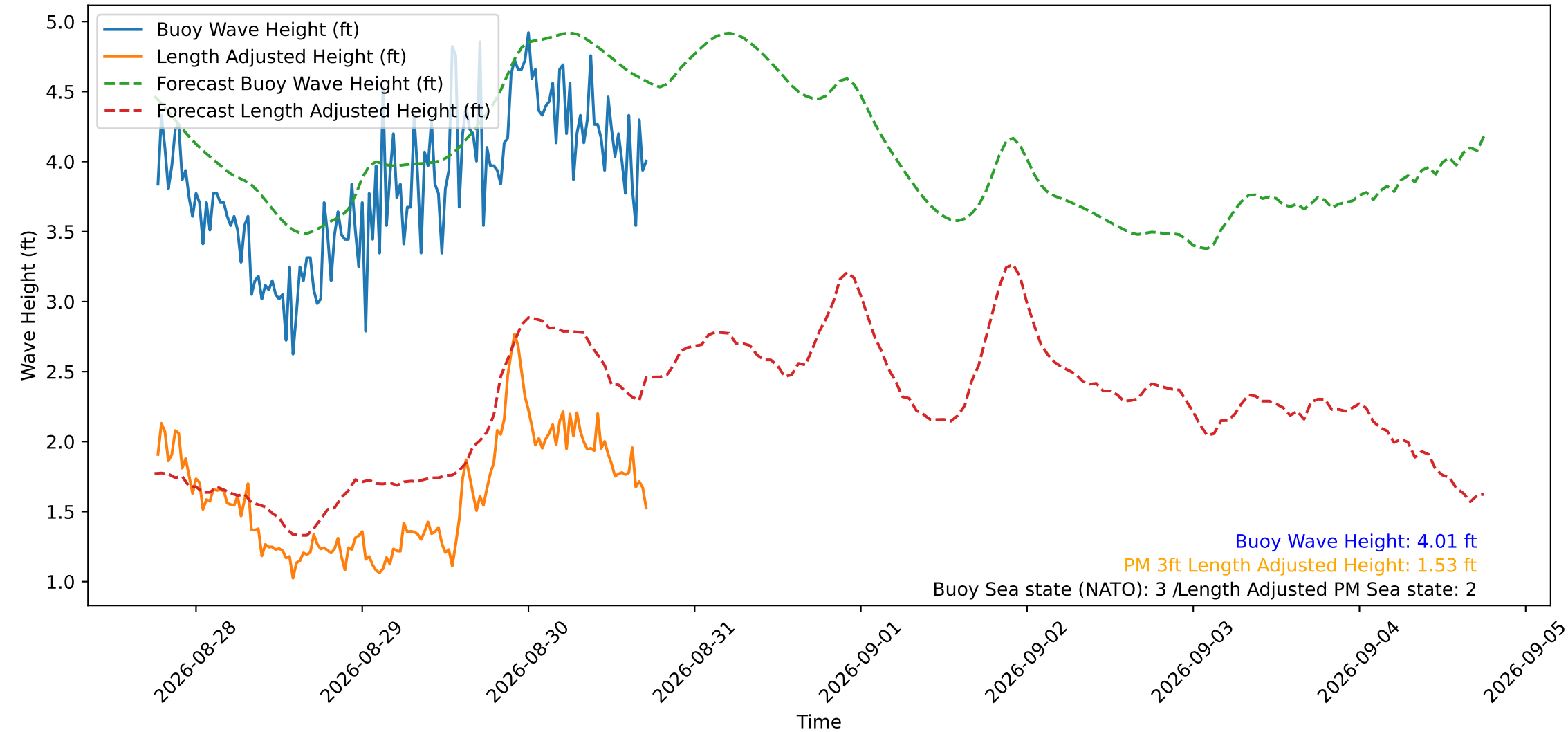
Wave Heights over Time for Green Beach at 2026-08-30 18:01:12
