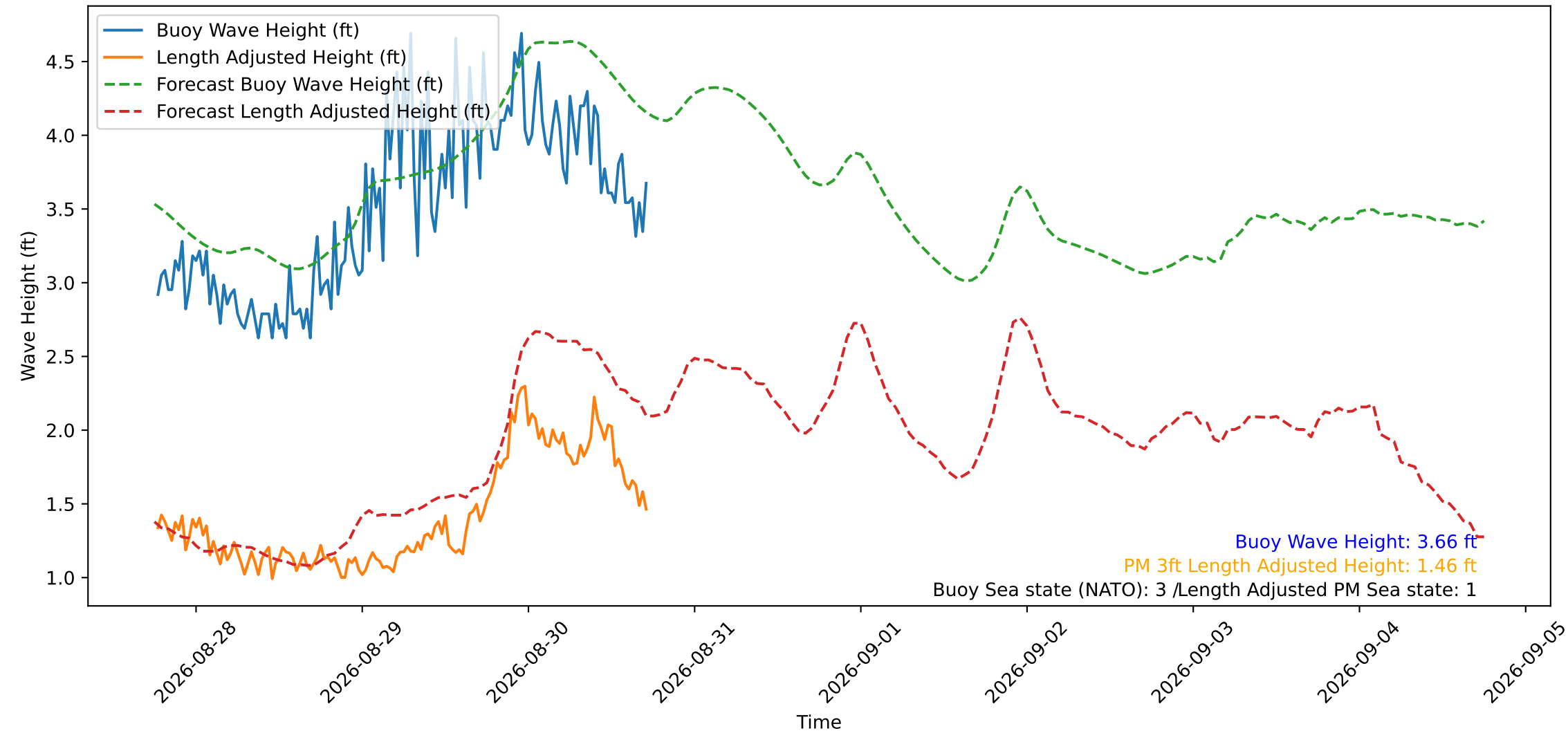
Wave Heights over Time for Red Beach at 2026-08-30 18:00:49
