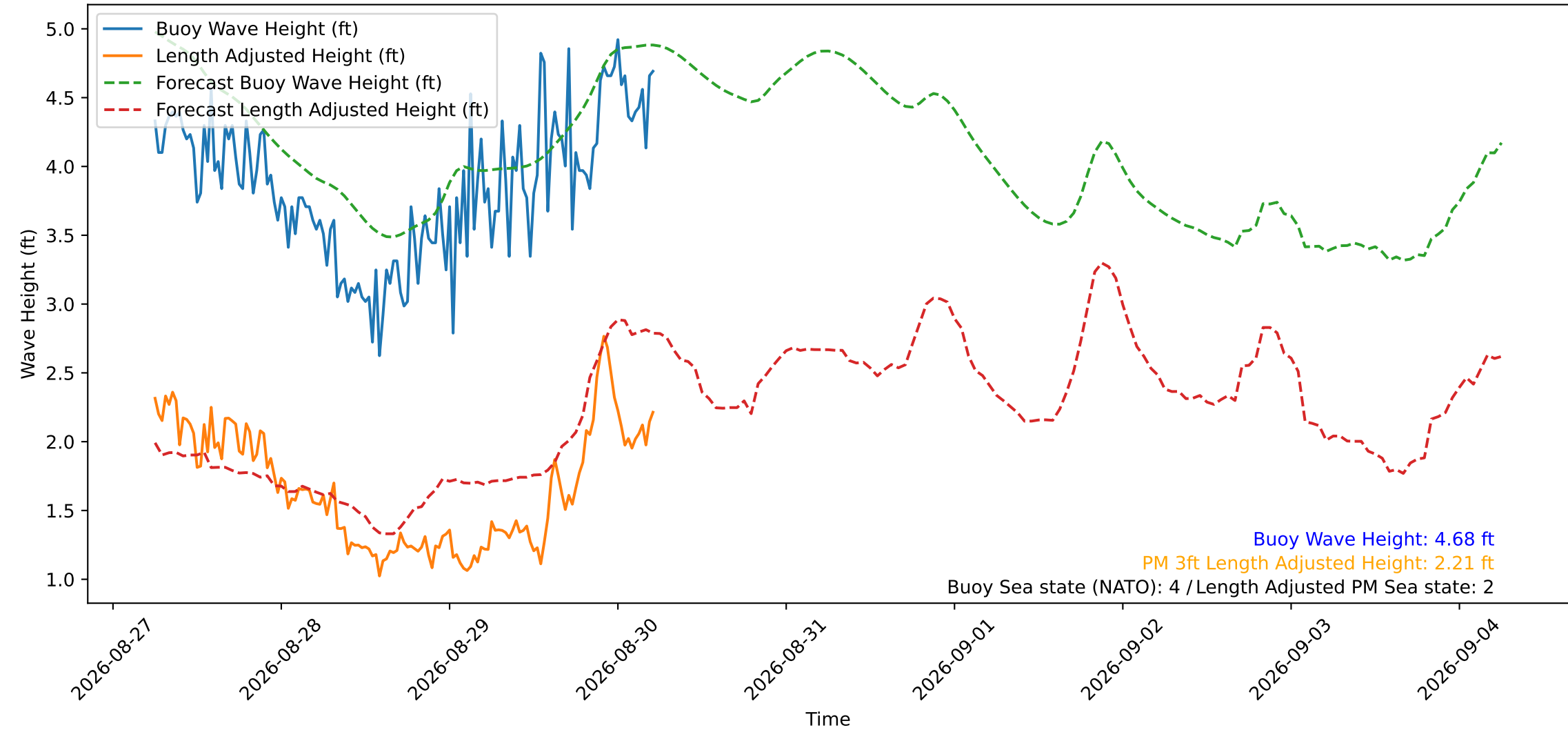
Wave Heights over Time for Green Beach at 2026-08-30 05:51:15
