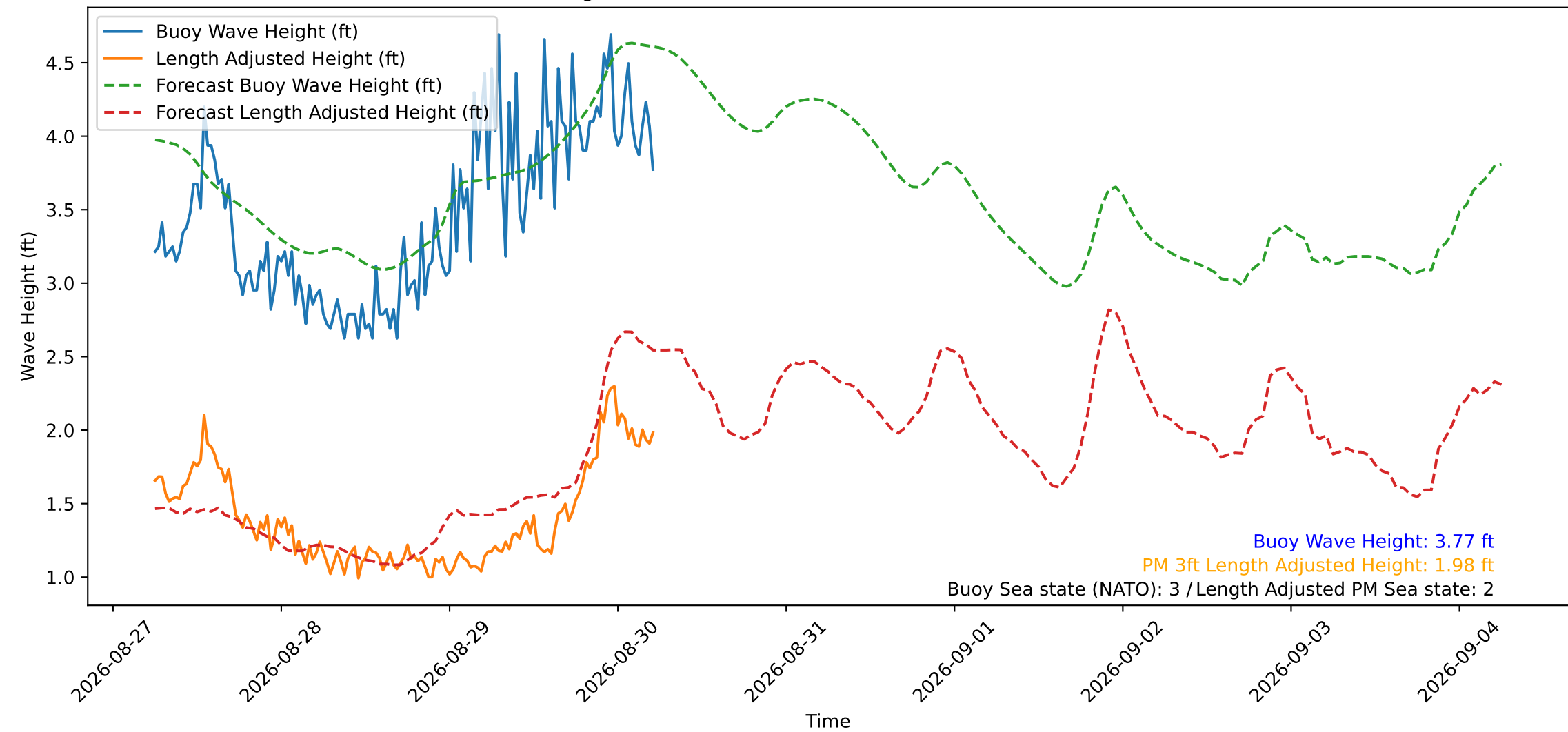
Wave Heights over Time for Red Beach at 2026-08-30 05:50:50
