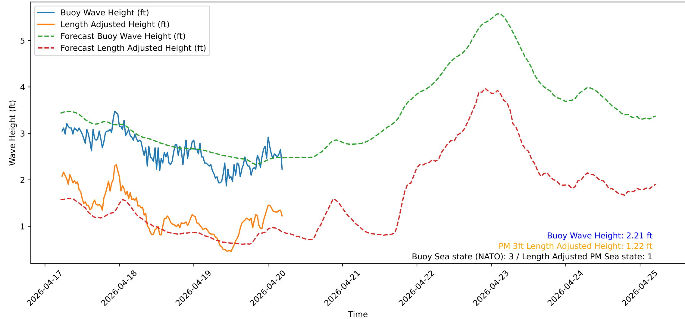
Wave Heights over Time for Green Beach at 2026-04-20 05:21:17
