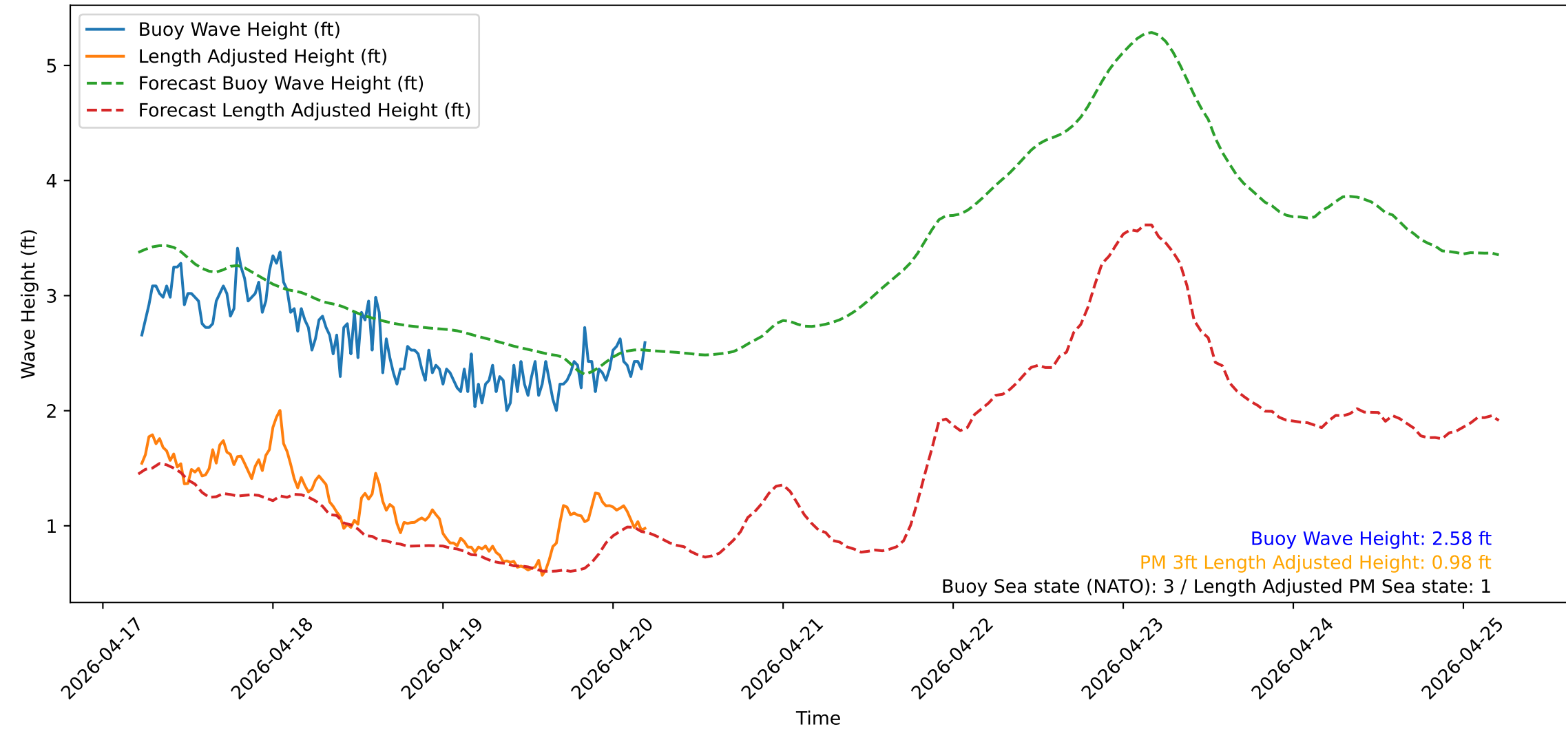
Wave Heights over Time for Oceanside Harbor at 2026-04-20 05:20:31
