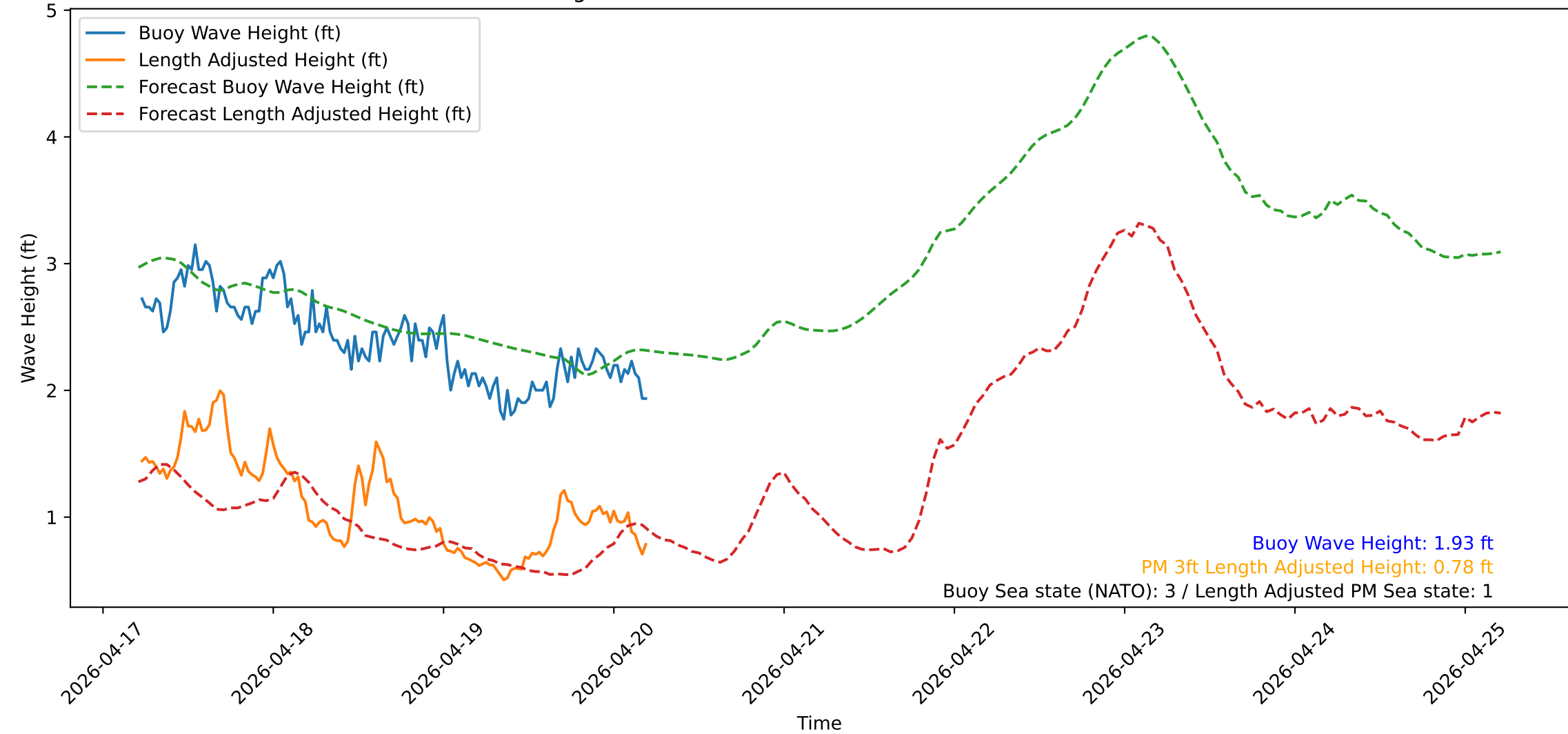
Wave Heights over Time for Red Beach at 2026-04-20 05:20:51
