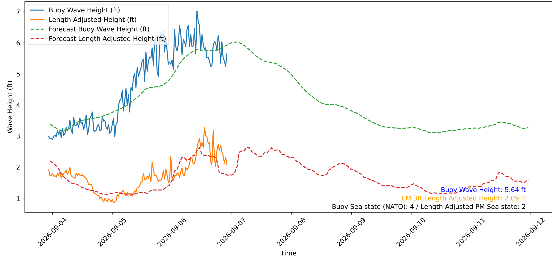
Wave Heights over Time for Oceanside Harbor at 2026-09-06 22:40:30
