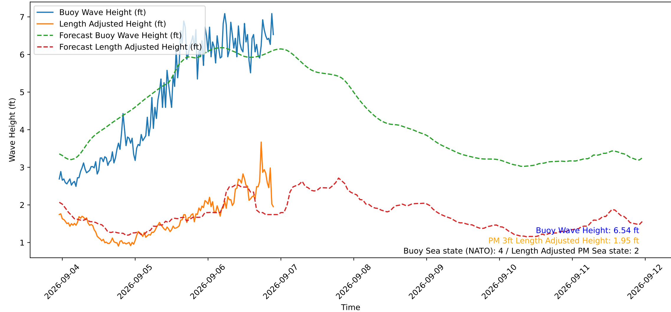
Wave Heights over Time for Green Beach at 2026-09-06 22:41:13
