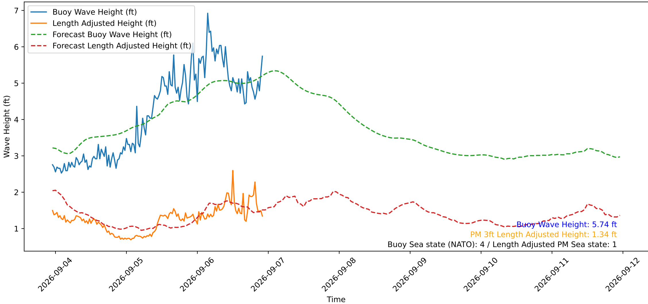
Wave Heights over Time for Red Beach at 2026-09-06 22:40:50
