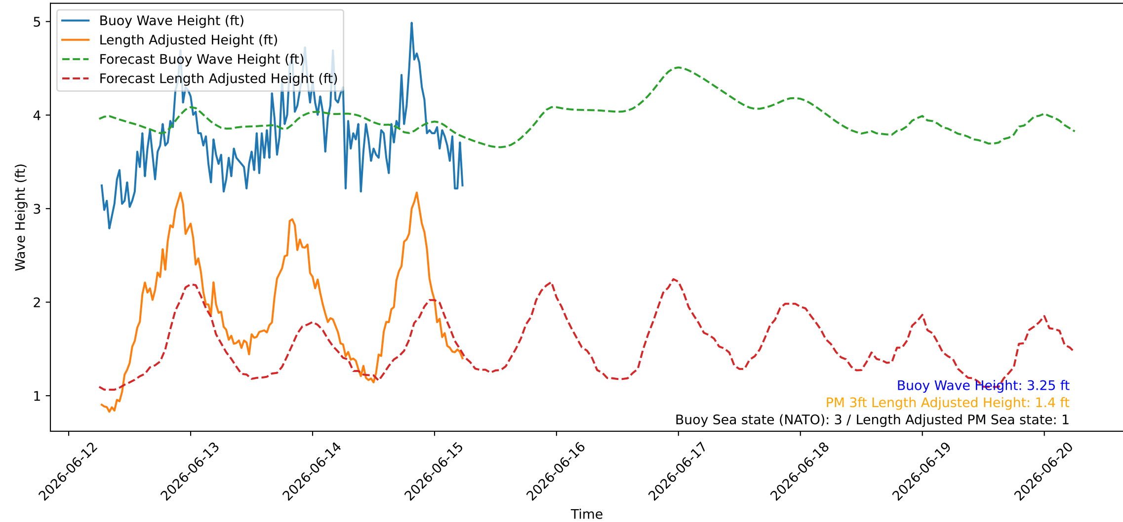
Wave Heights over Time for Oceanside Harbor at 2026-06-15 06:20:26
