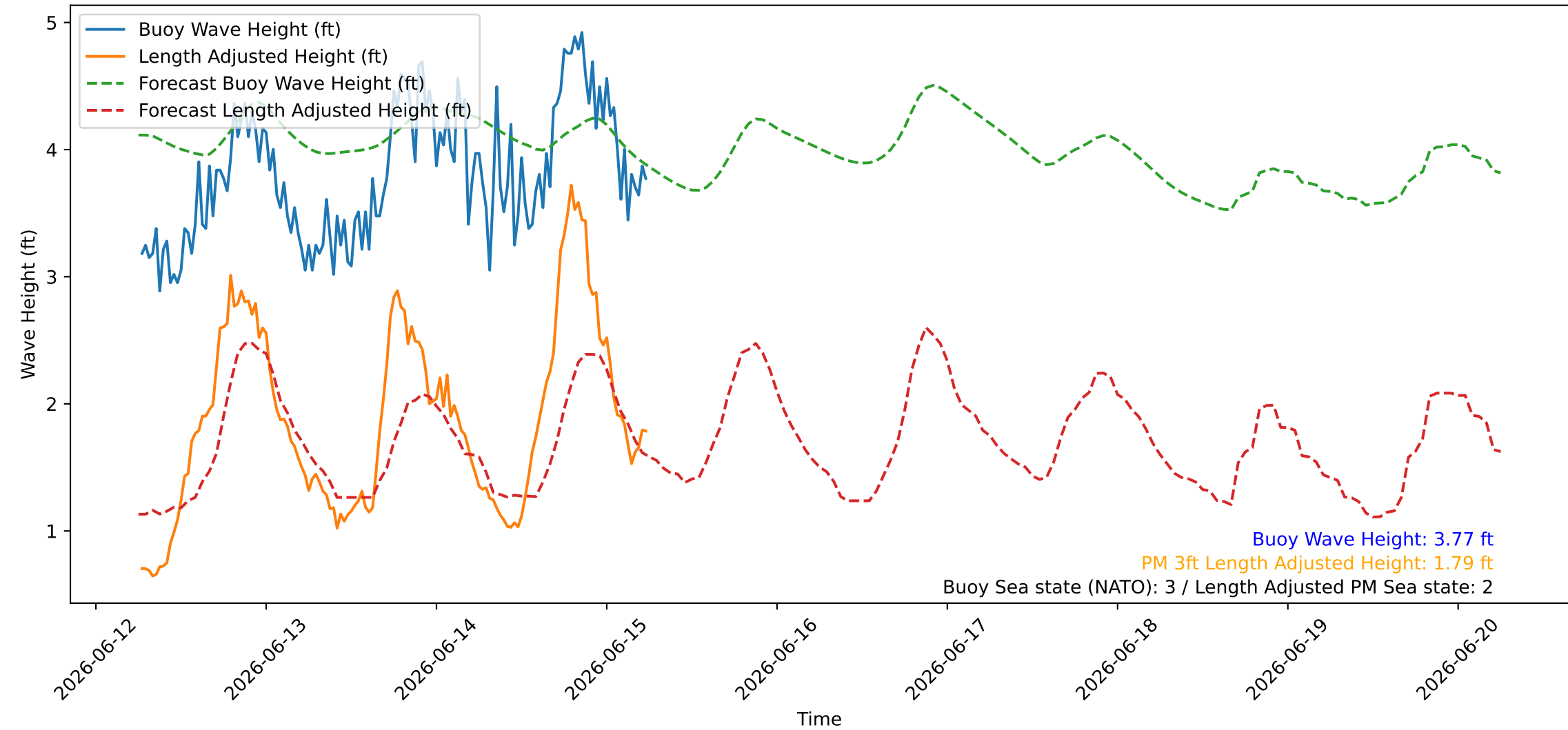
Wave Heights over Time for Green Beach at 2026-06-15 06:21:09
