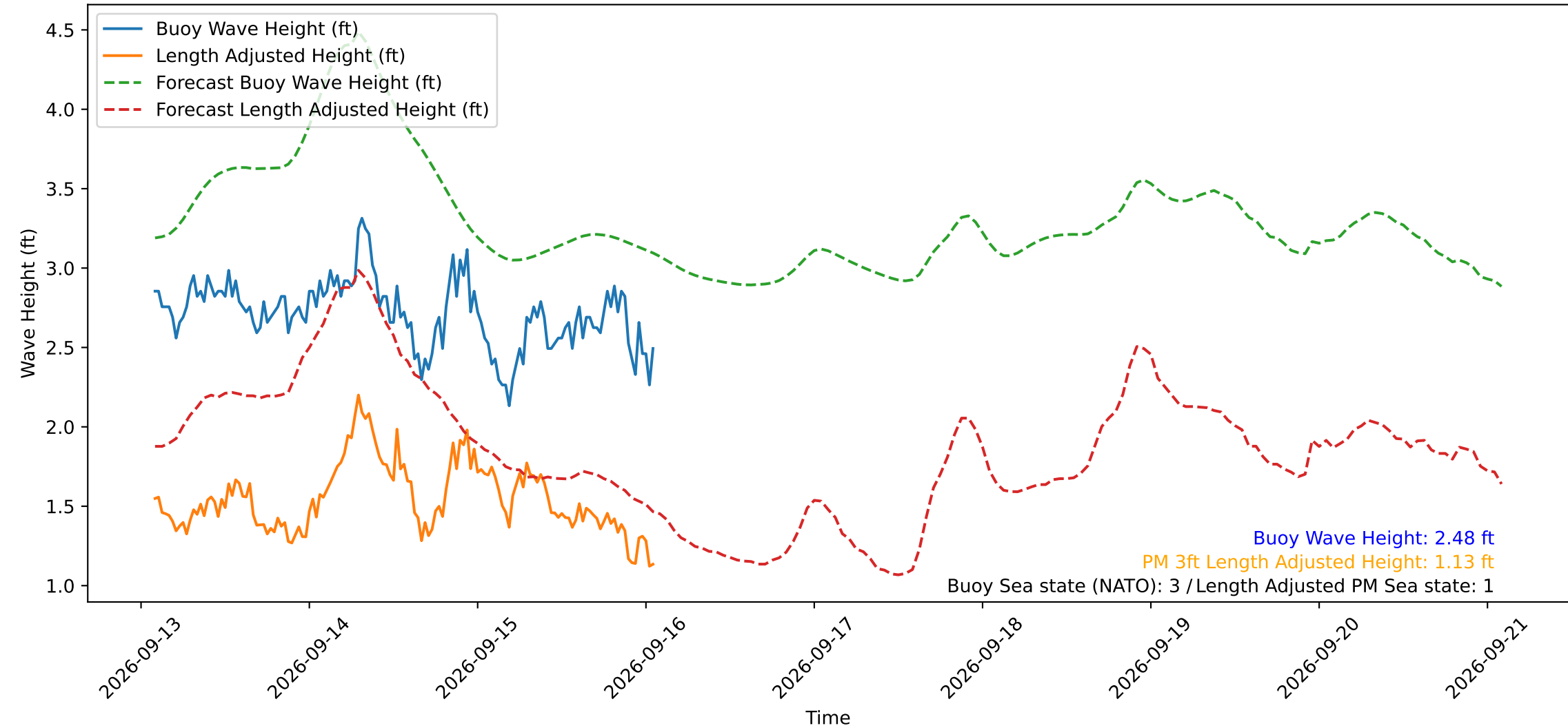
Wave Heights over Time for Green Beach at 2026-09-16 01:51:14
