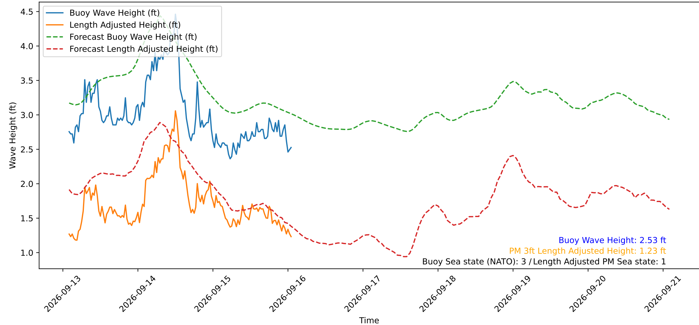
Wave Heights over Time for Oceanside Harbor at 2026-09-16 01:50:30
