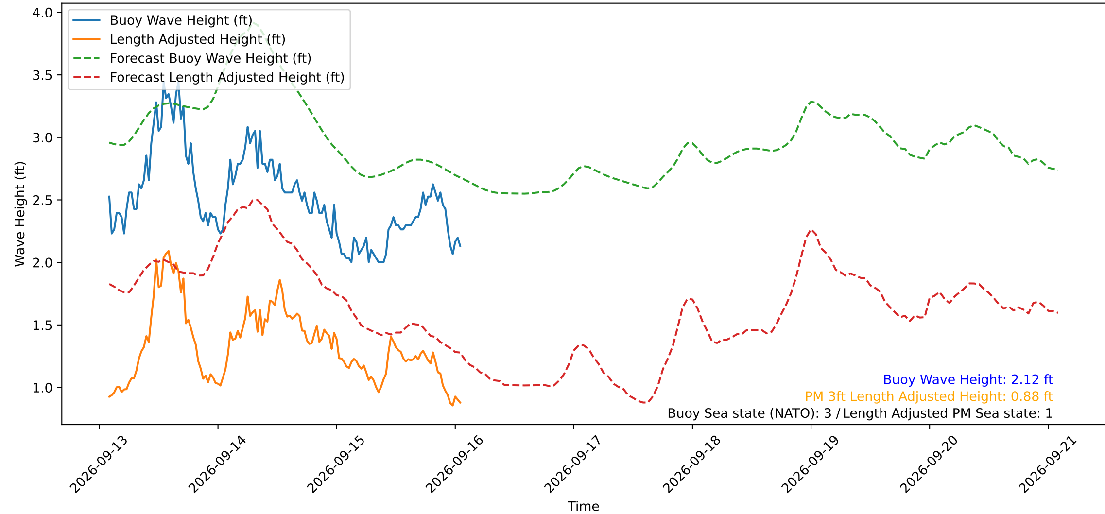
Wave Heights over Time for Red Beach at 2026-09-16 01:50:51
