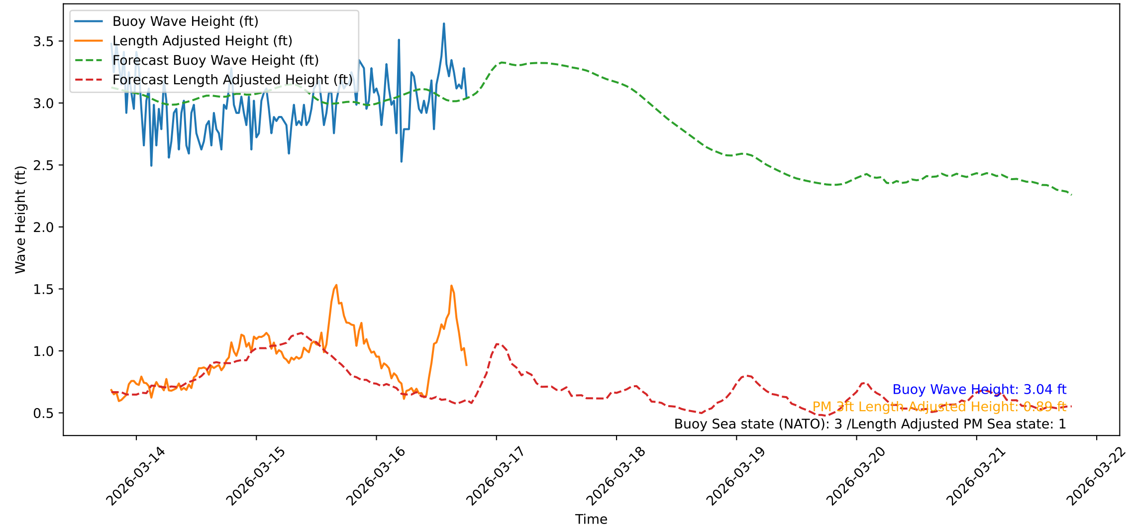
Wave Heights over Time for Red Beach at 2026-03-16 18:51:06
