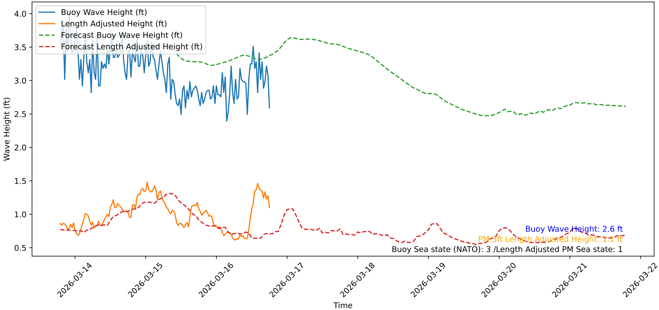
Wave Heights over Time for Oceanside Harbor at 2026-03-16 18:50:43
