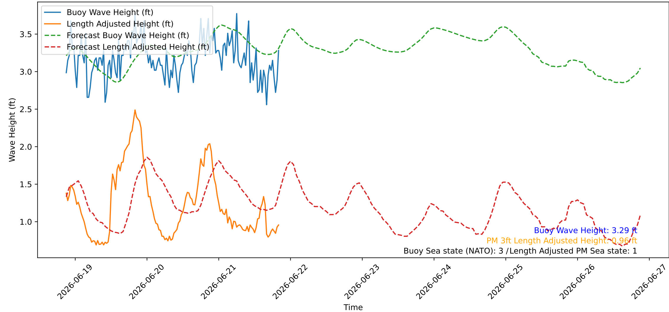
Wave Heights over Time for Red Beach at 2026-06-21 20:40:46
