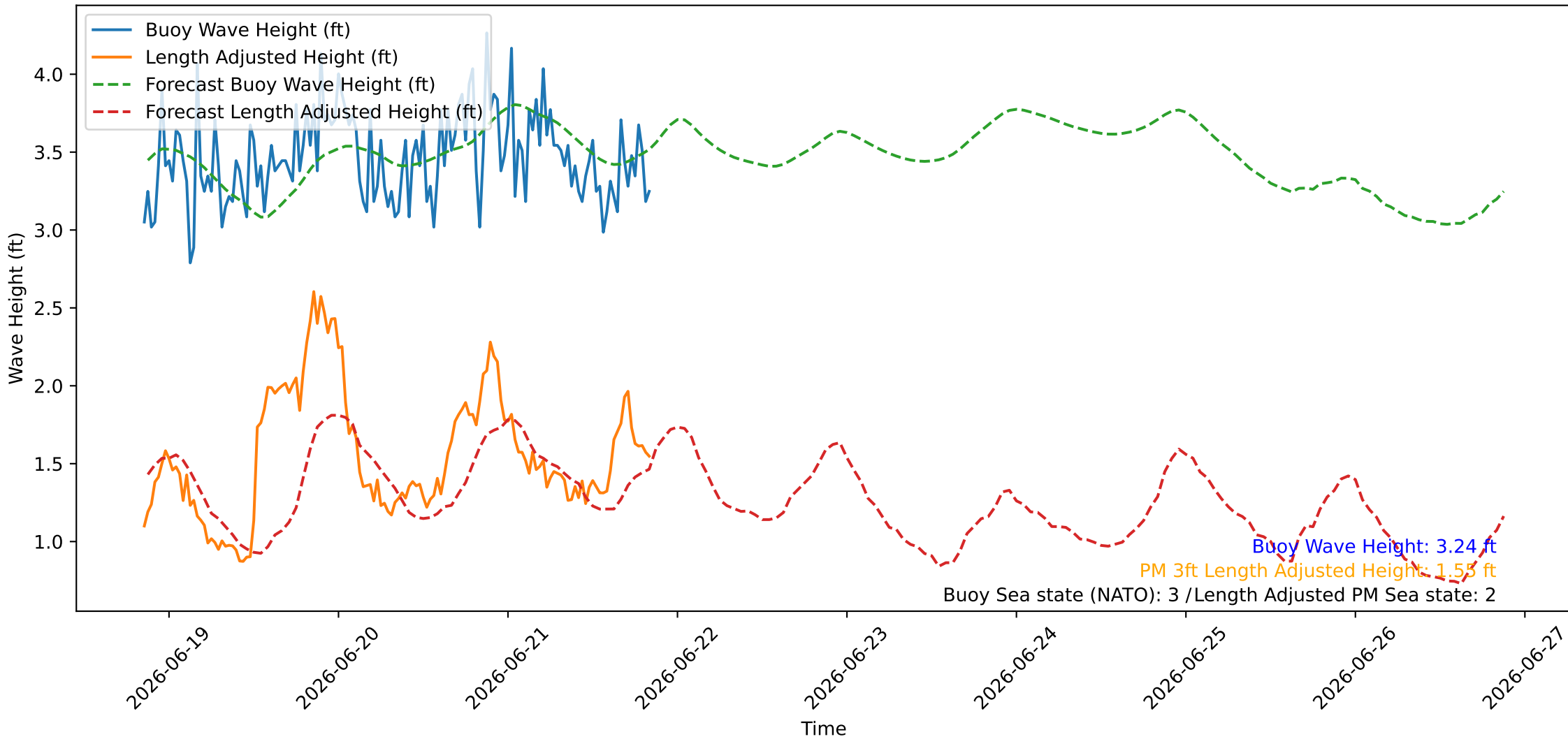
Wave Heights over Time for Oceanside Harbor at 2026-06-21 20:40:26
