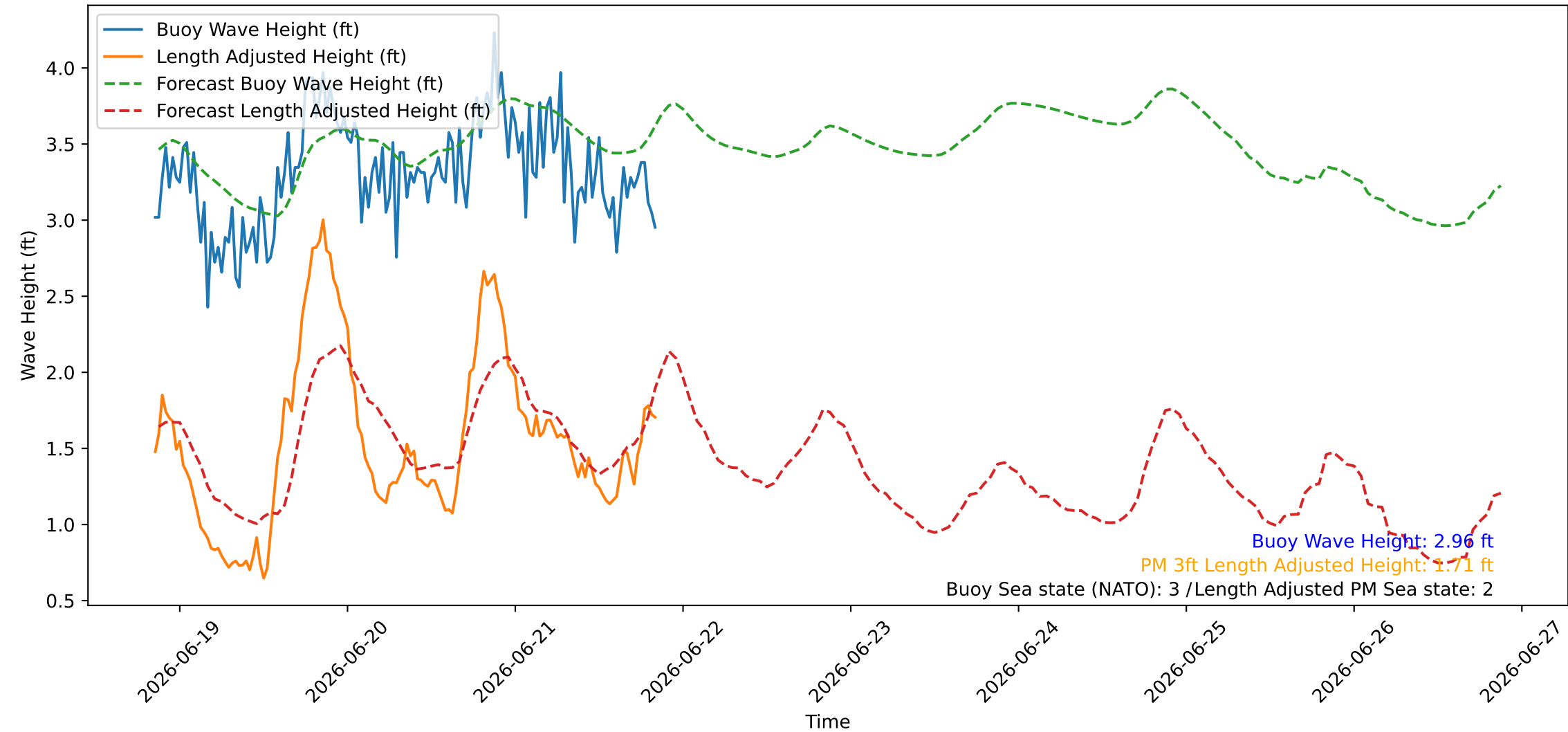
Wave Heights over Time for Green Beach at 2026-06-21 20:41:08
