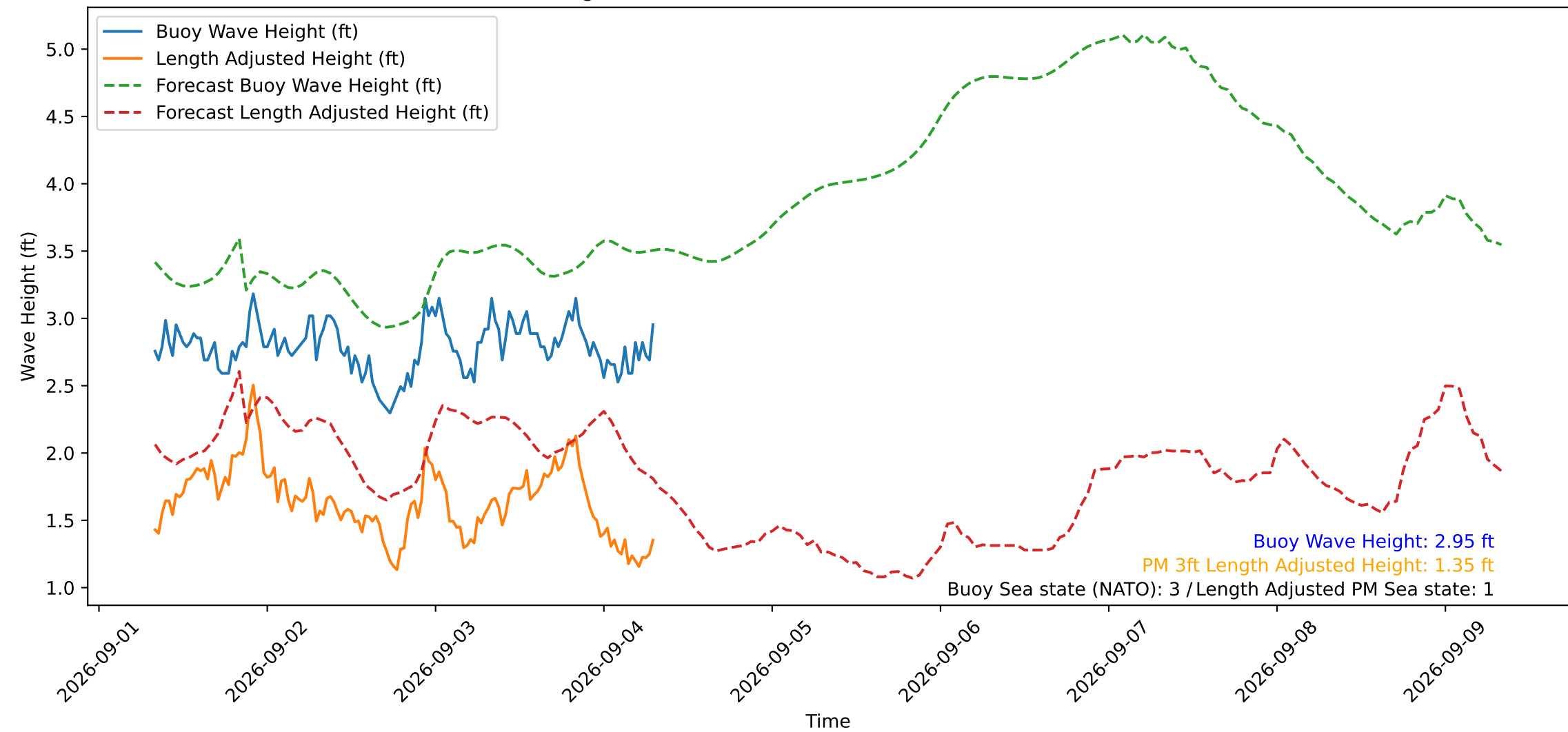
Wave Heights over Time for Red Beach at 2026-09-04 07:40:49
