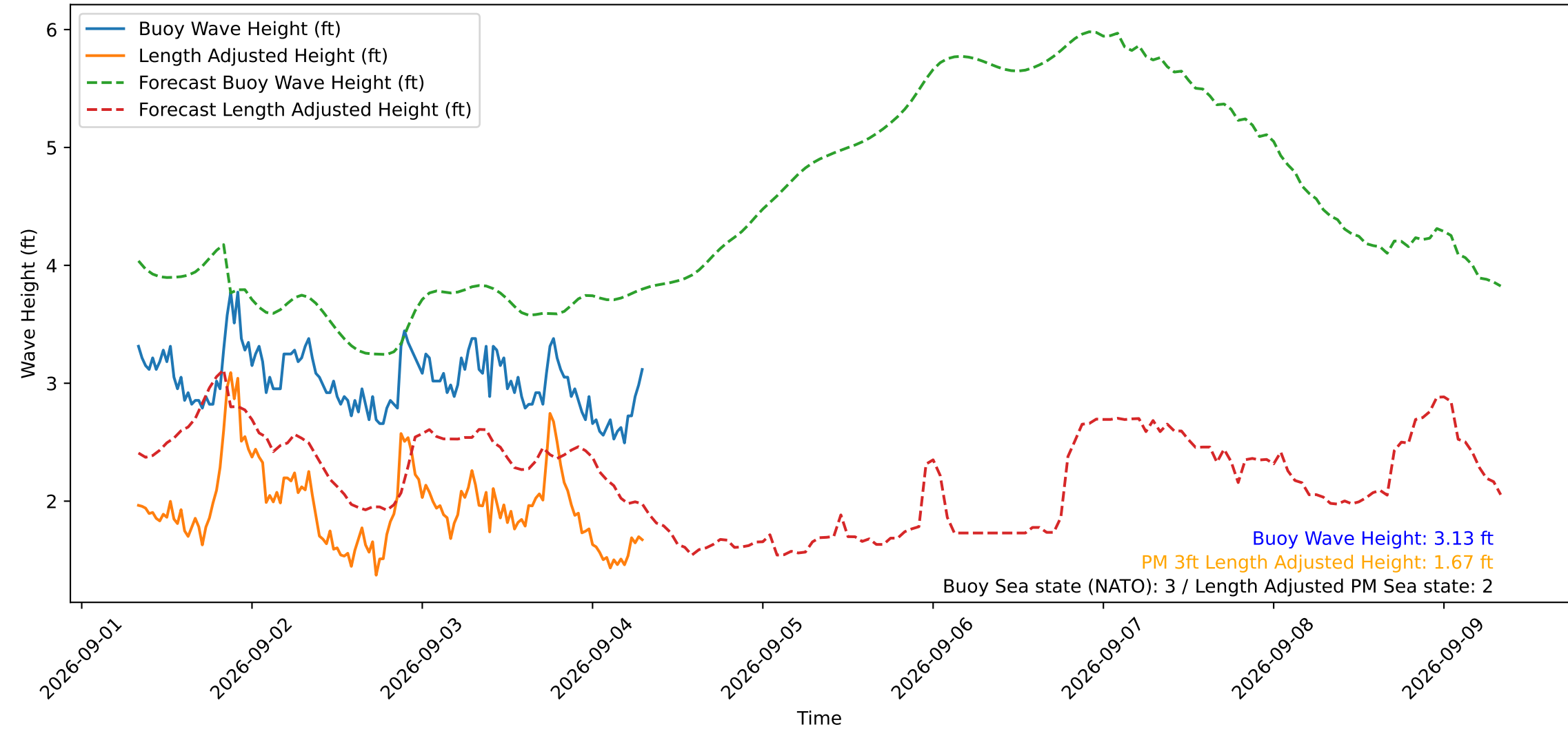
Wave Heights over Time for Green Beach at 2026-09-04 07:41:12
