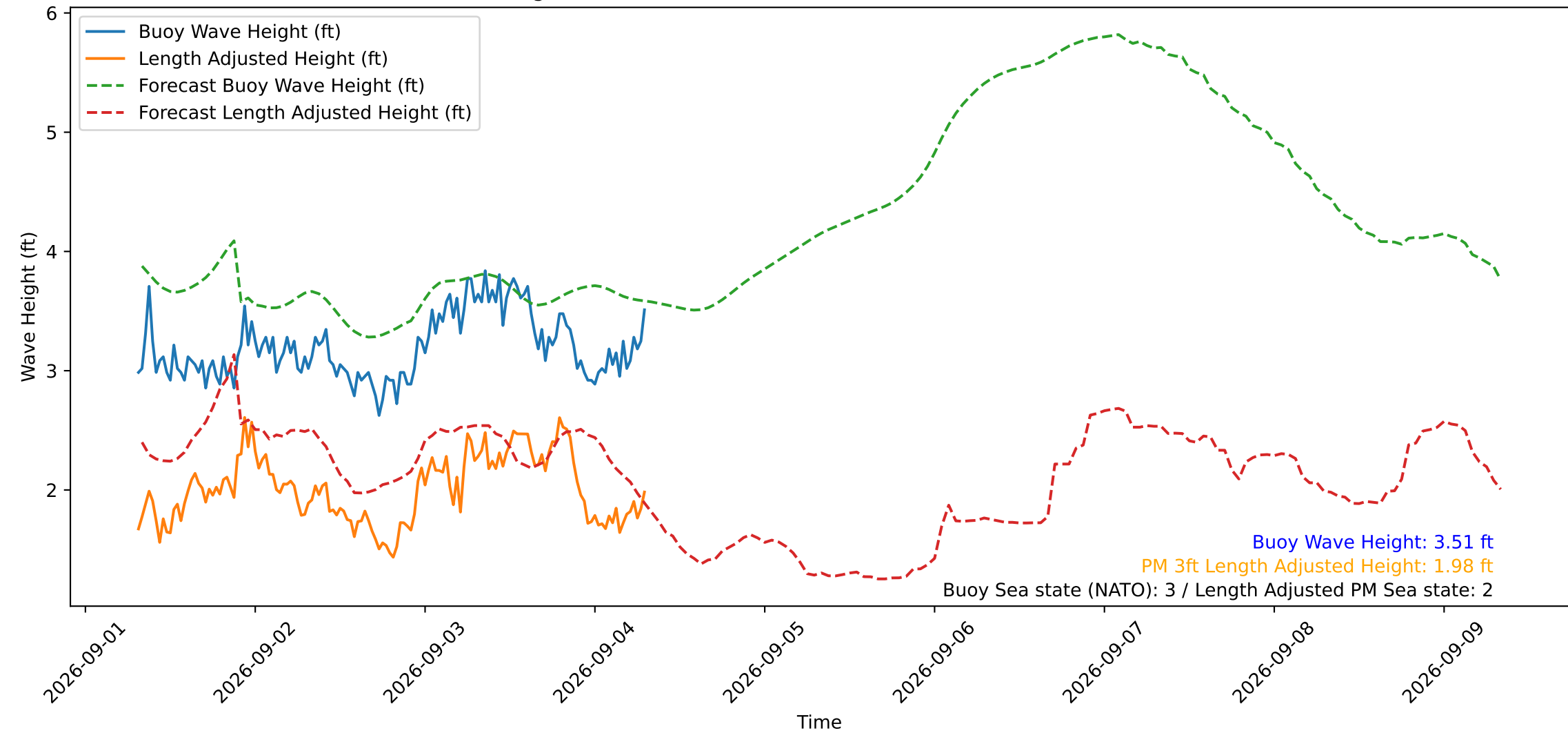
Wave Heights over Time for Oceanside Harbor at 2026-09-04 07:40:30
