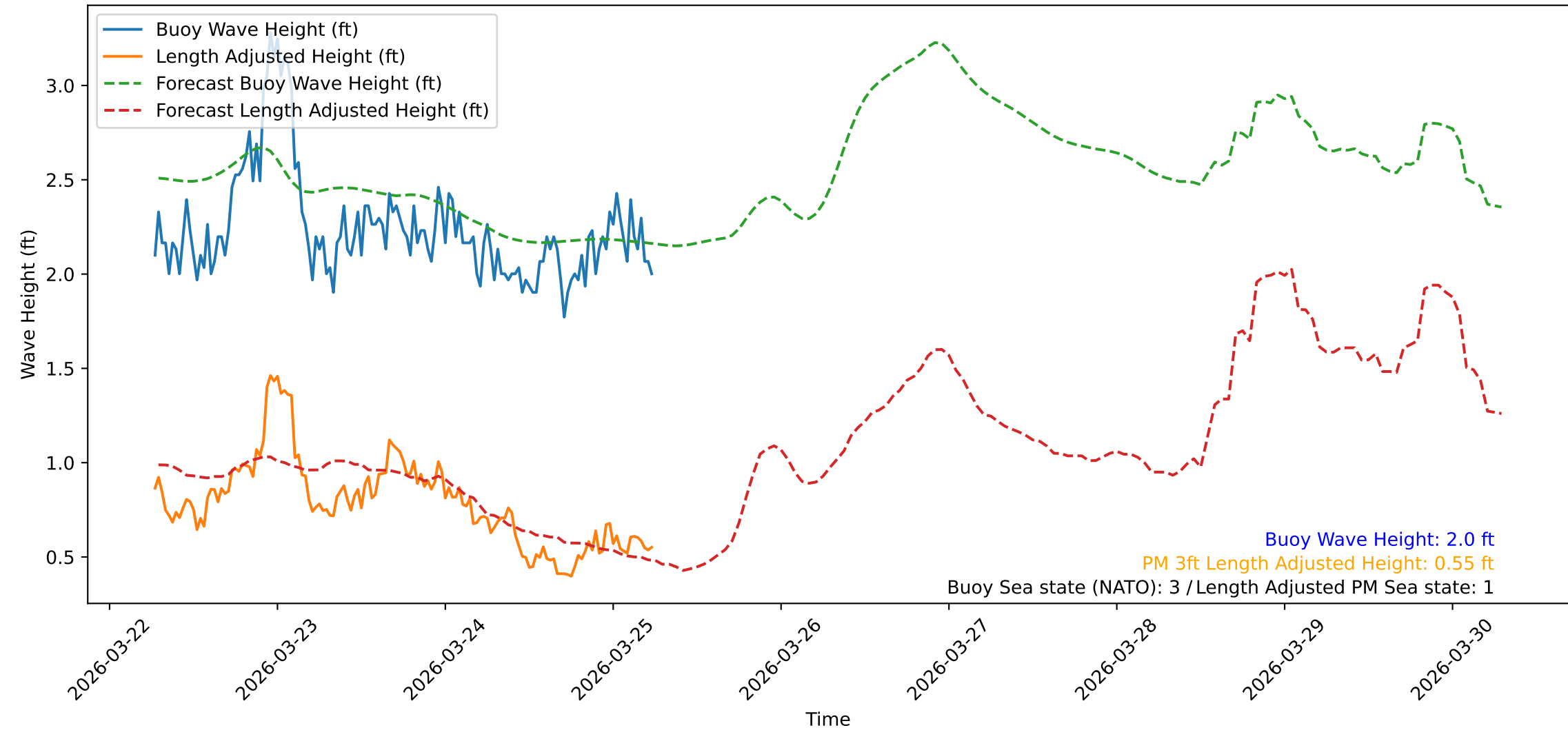
Wave Heights over Time for Green Beach at 2026-03-25 06:31:11
