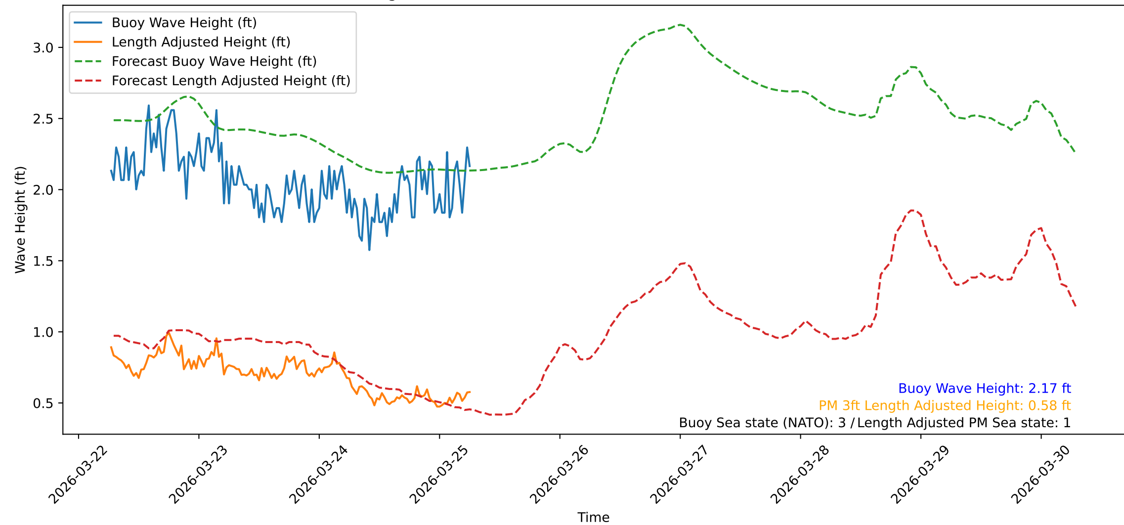
Wave Heights over Time for Oceanside Harbor at 2026-03-25 06:30:32
