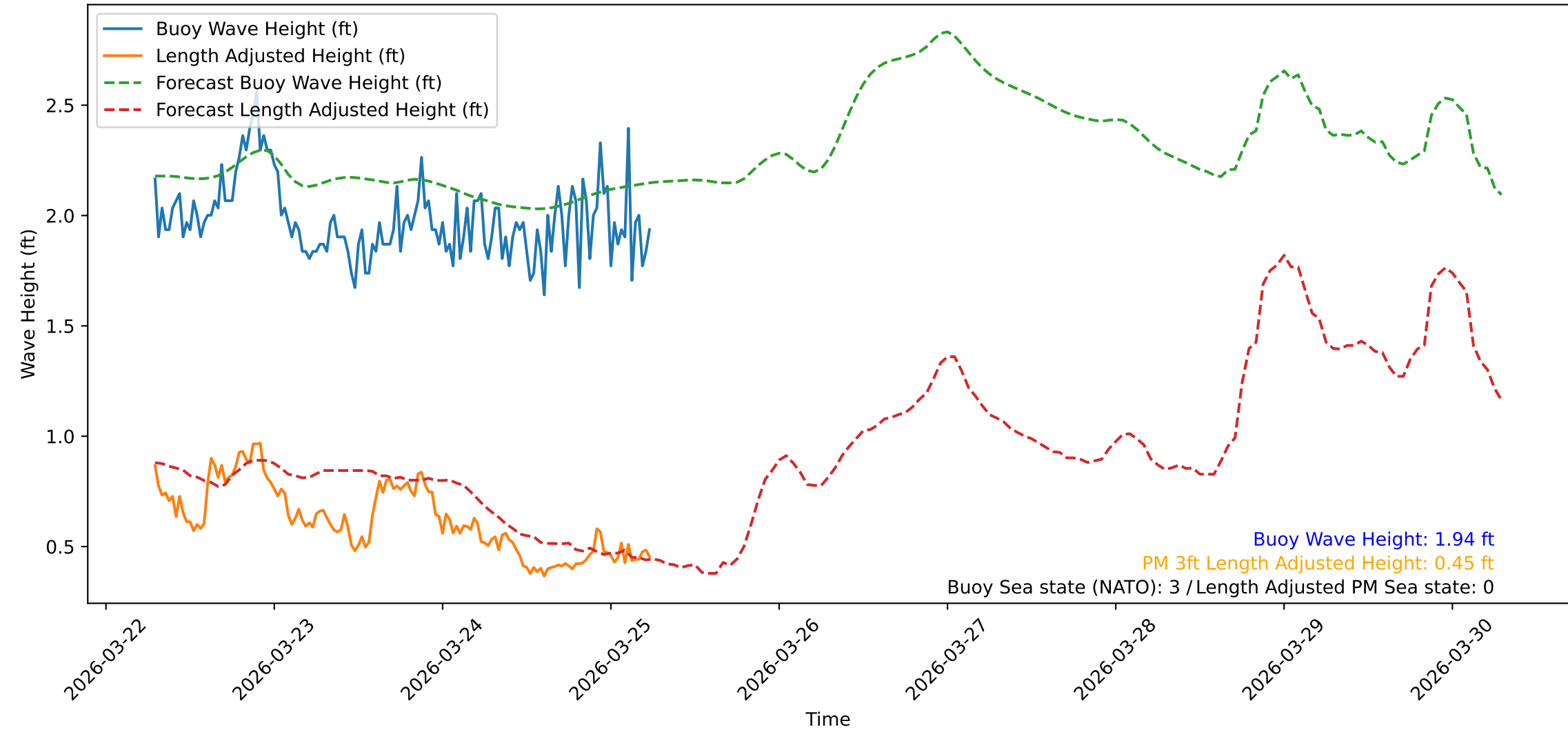
Wave Heights over Time for Red Beach at 2026-03-25 06:30:48
