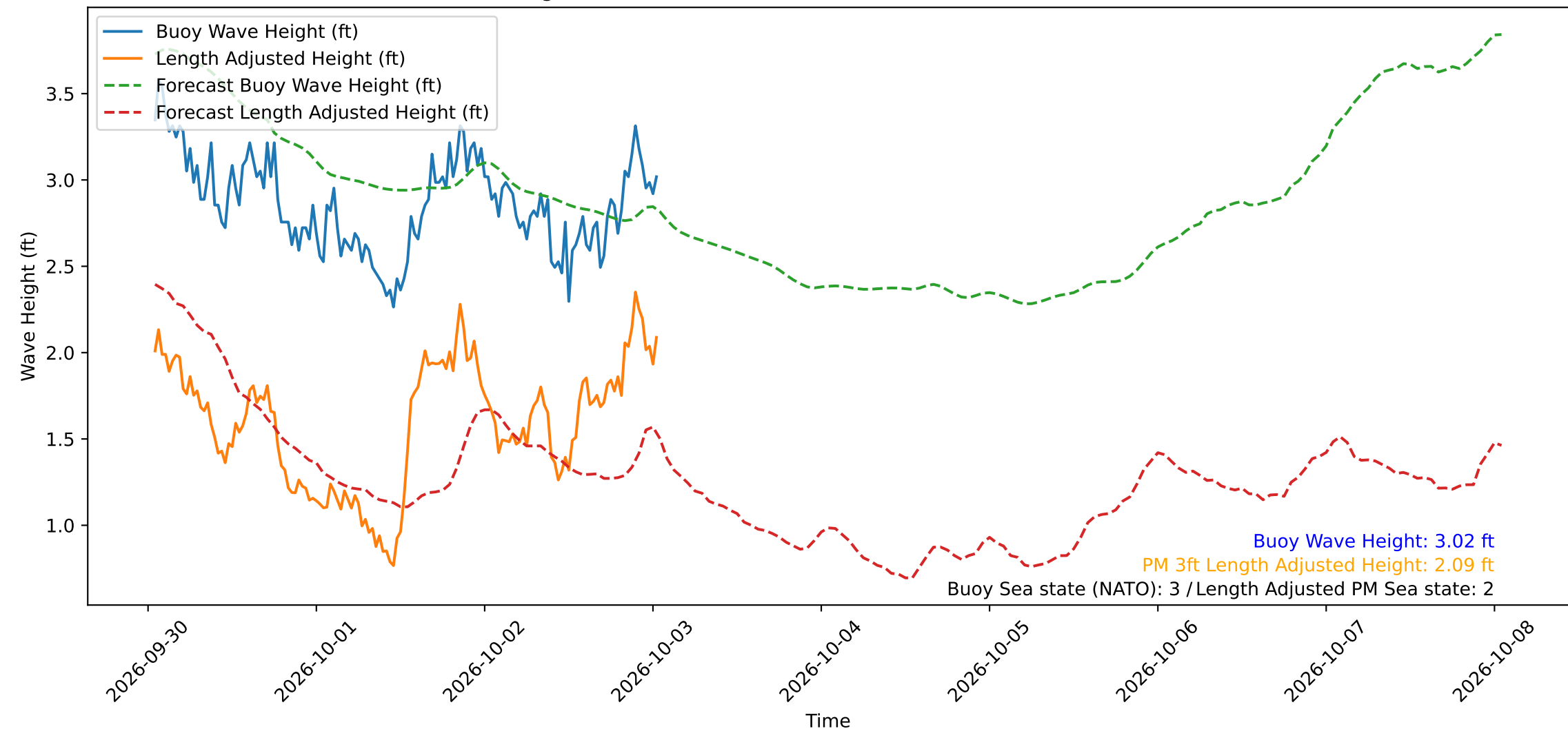
Wave Heights over Time for Oceanside Harbor at 2026-10-03 01:10:29
