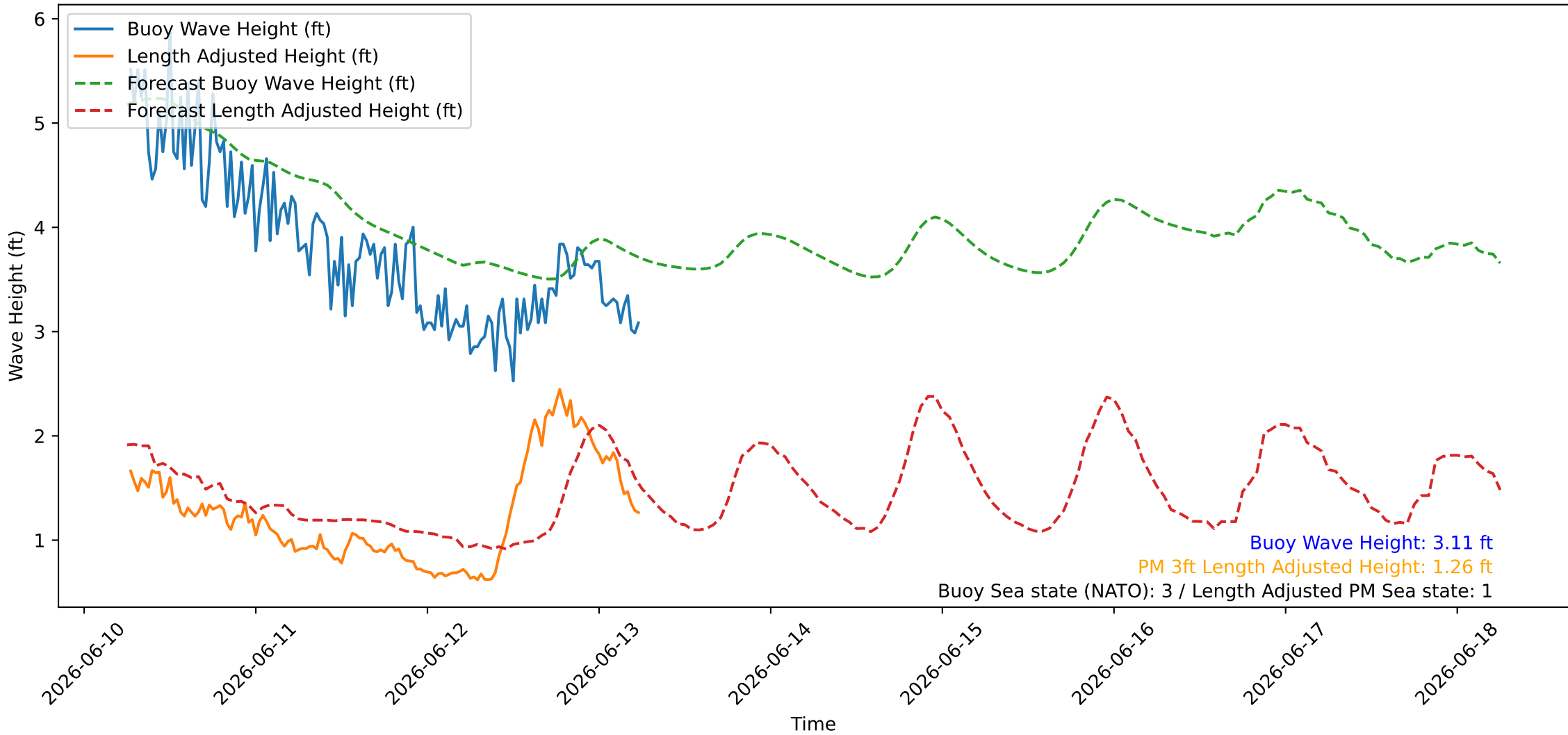
Wave Heights over Time for Red Beach at 2026-06-13 06:20:46
