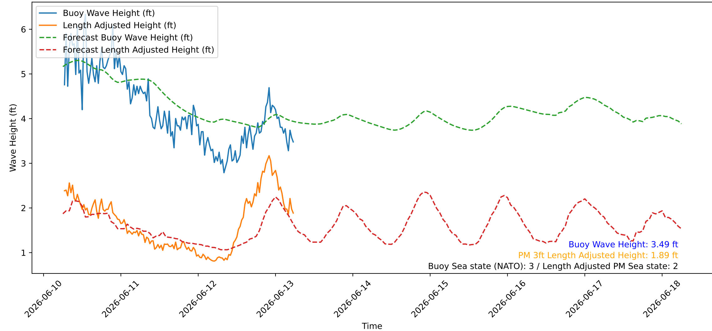
Wave Heights over Time for Oceanside Harbor at 2026-06-13 06:20:26
