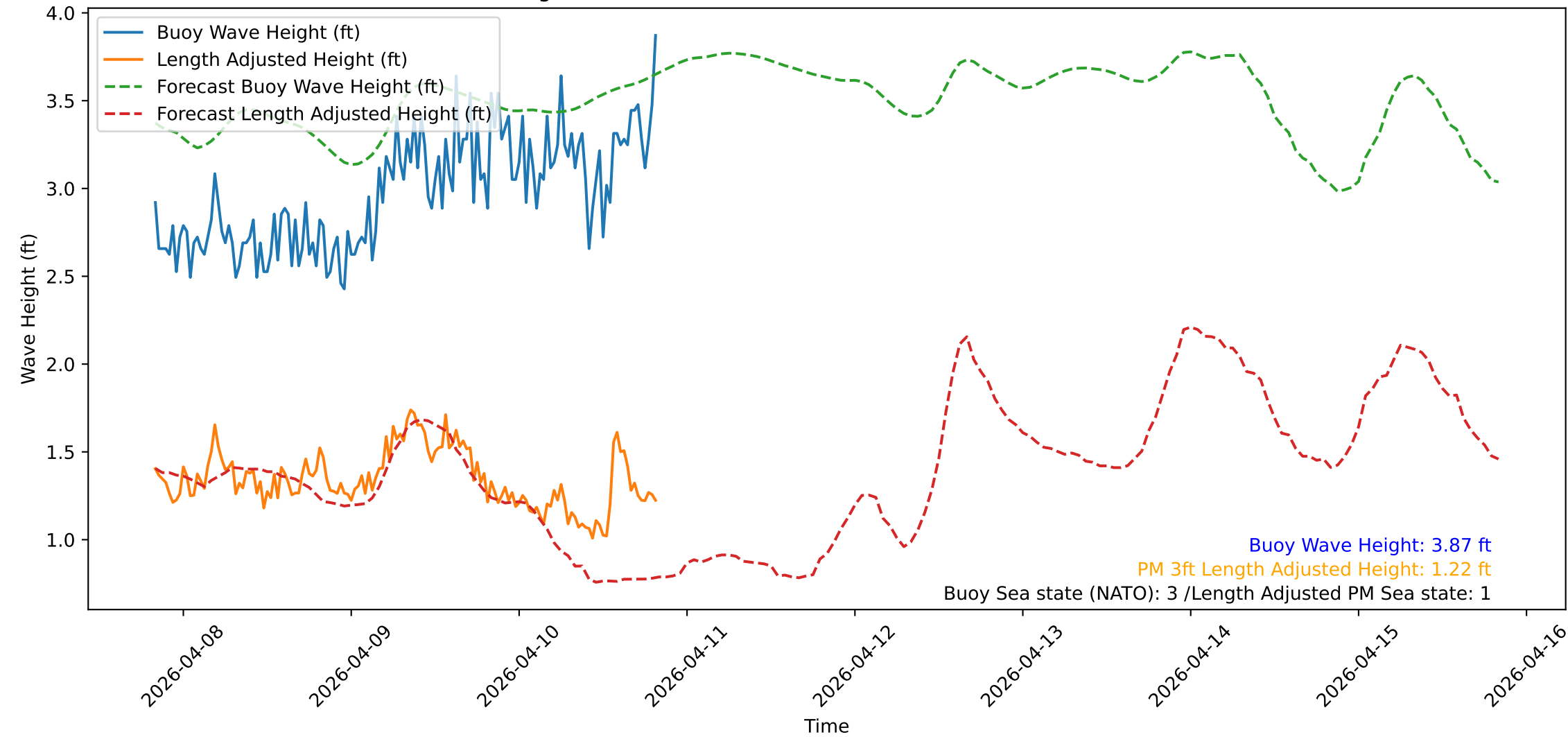
Wave Heights over Time for Oceanside Harbor at 2026-04-10 20:10:31
