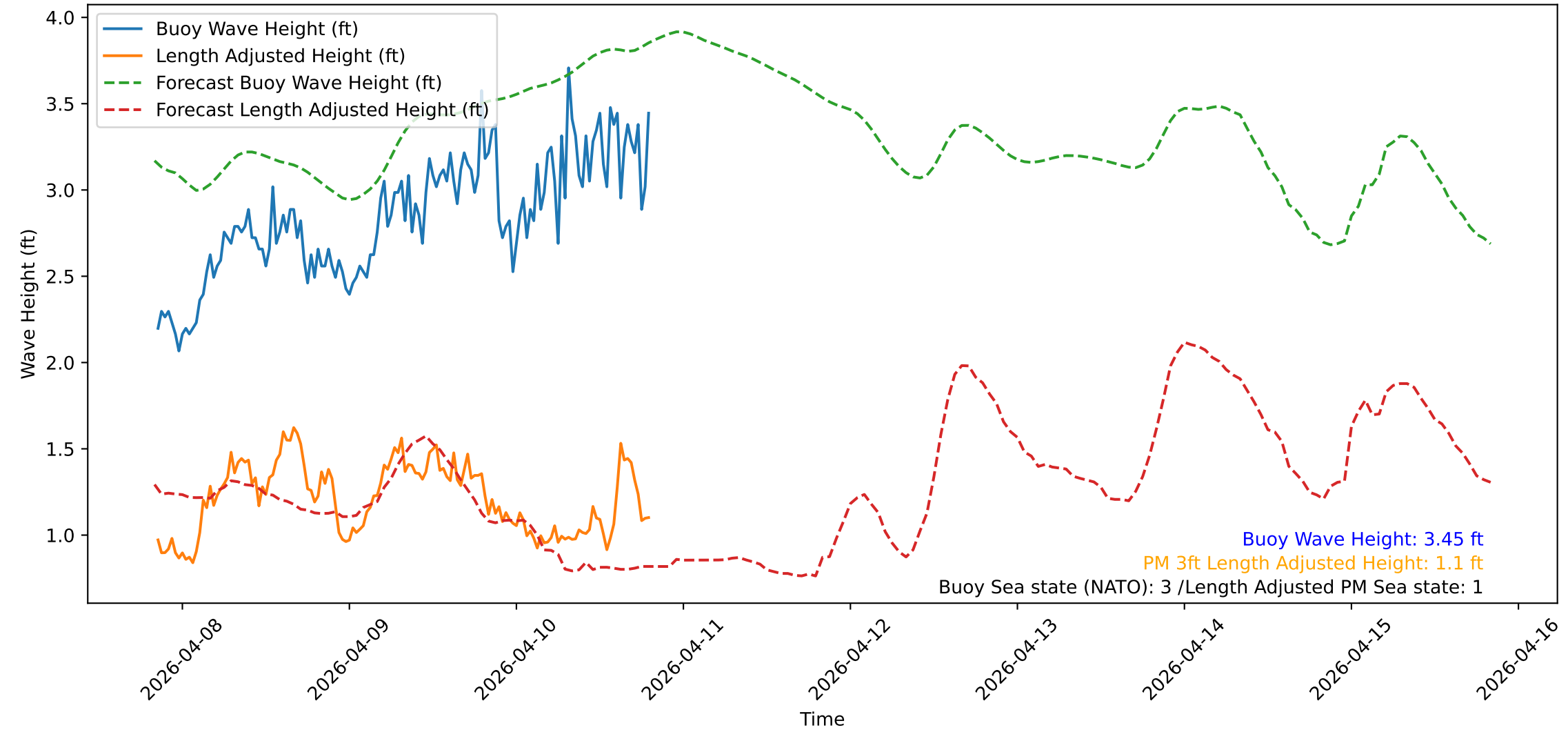
Wave Heights over Time for Red Beach at 2026-04-10 20:10:51
