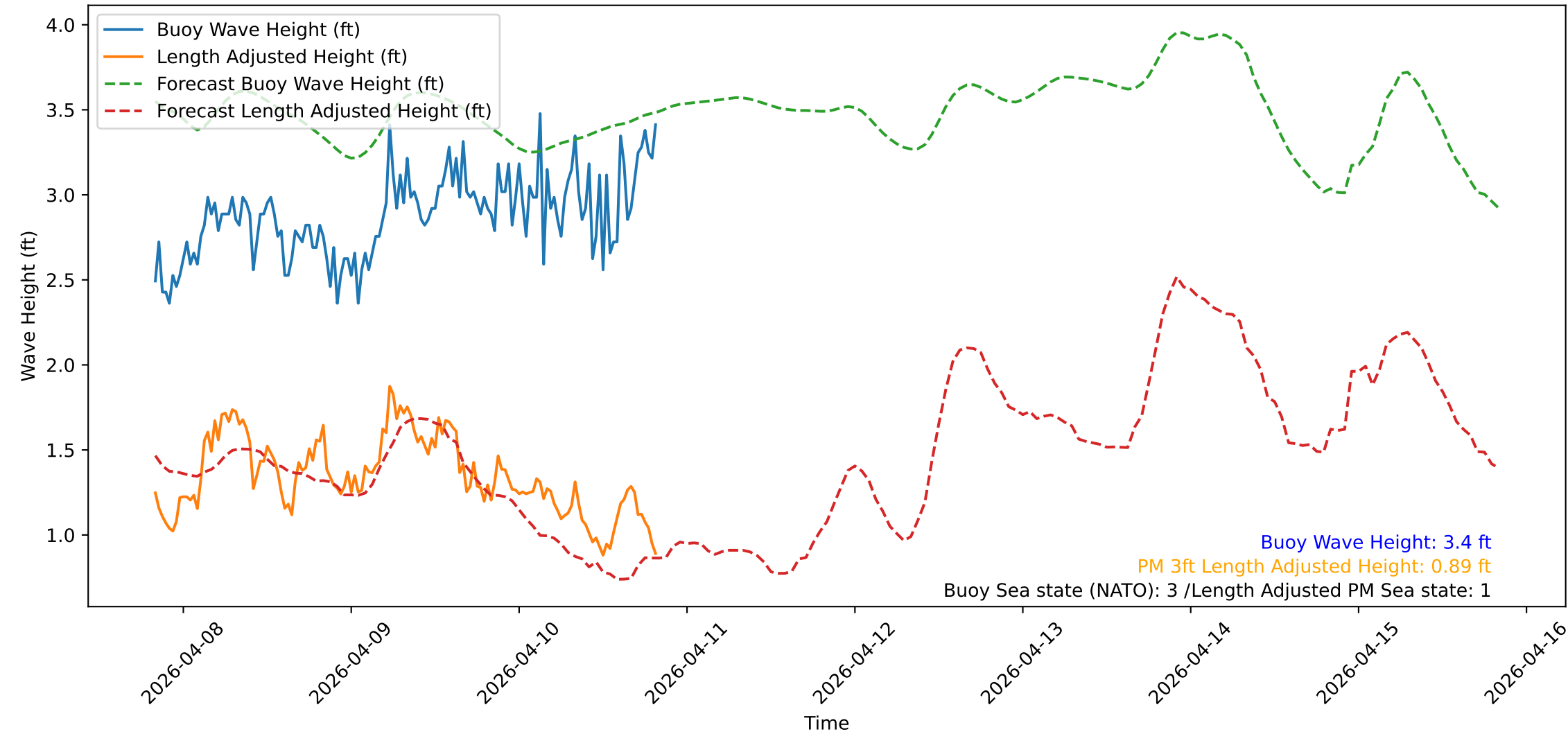
Wave Heights over Time for Green Beach at 2026-04-10 20:11:13
