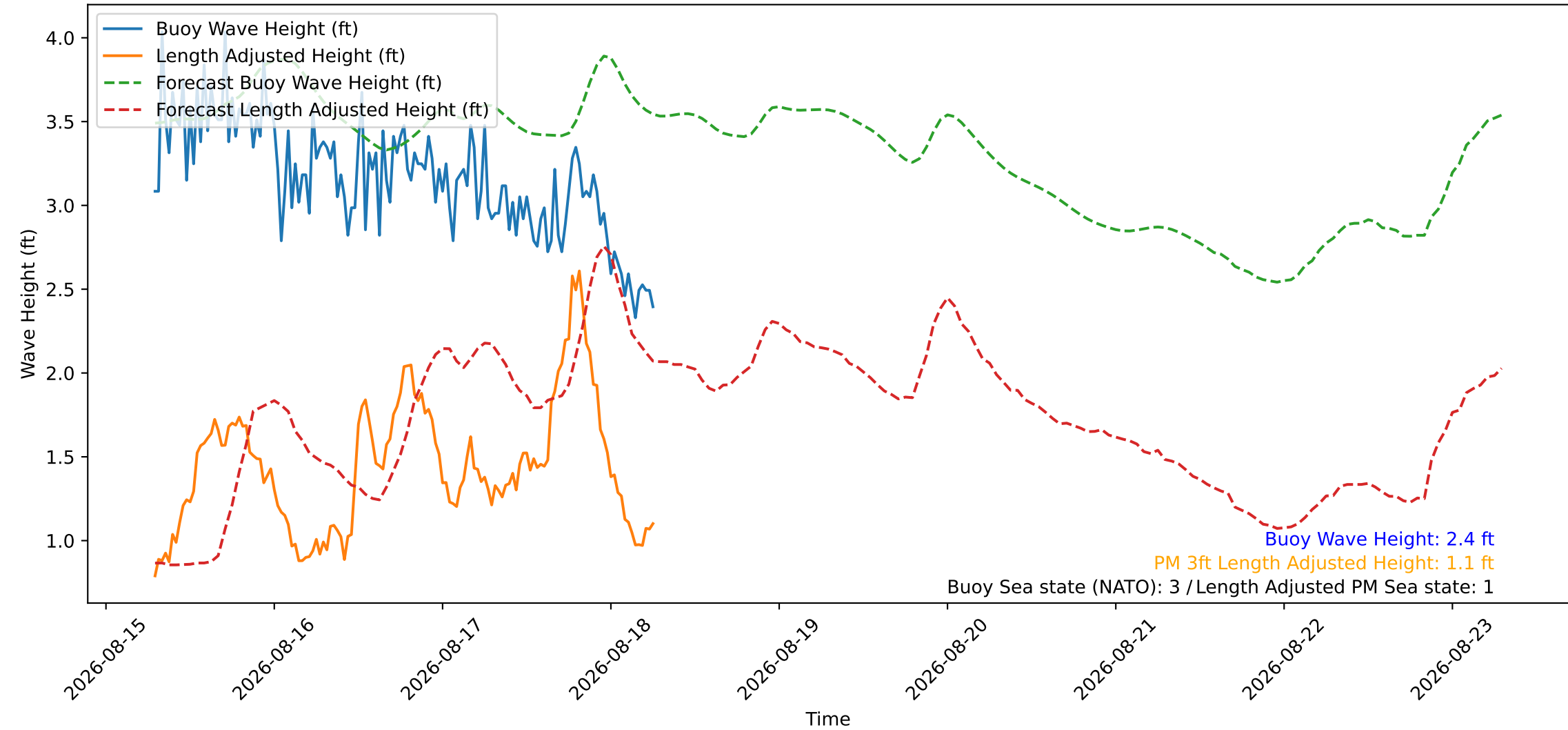
Wave Heights over Time for Red Beach at 2026-08-18 06:50:47
